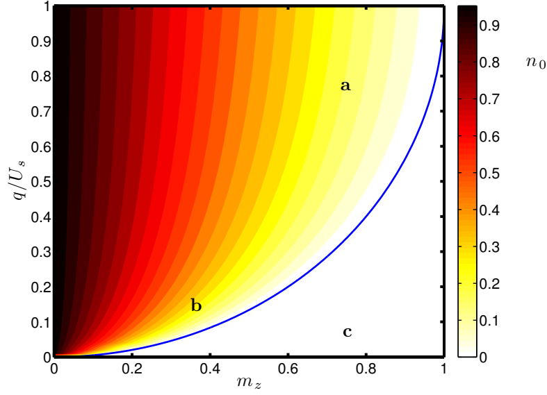
Figure 3.14: Position in the magnetic phase diagram of the three initial states considered in figure (3.13). We use U_s = 45 Hz which we calculated from the measured atom number and a numerical solution of the Gross-Pitaevskii equation. The blue line represents the critical field.
