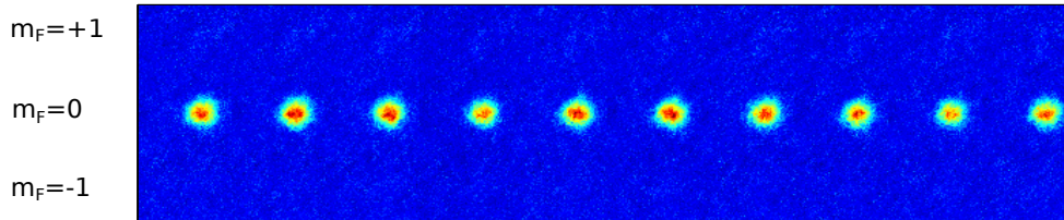
Figure 5.2: A serie of 10 experimental images after a Stern-Gerlach separation of the three spin states and absorption imaging when the applied magnetic field is 850 mG ( q = 200 Hz). Almost all the atoms are in the |m_F = 0\rangle spin state, the fluctuations are extremely reduced.
