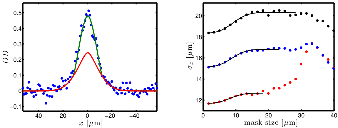
Figure 2.6: On the left: Cut along the x axis of a bimodal fit of the atomic density in an absorption image. The blue points show the measured optical density of the atomic cloud, the red and green curves correspond respectively to the fitted Bose function and Thomas-Fermi function. The evaporation point is 700 ms. On the right: Size (along the x axis) of the Bose function fitted outside the mask as a function of the mask size for an evaporation time of 600 ms. The three sets of points - red, blue and black - correspond to three different absorption images taken at different times of flight: from bottom to top 0.6 ms, 0.8 ms and 1 ms. The solid curves fit each set of points by a function of the form d - a \exp(-x^3/2b^3) , from which we extract the value of the plateau.
