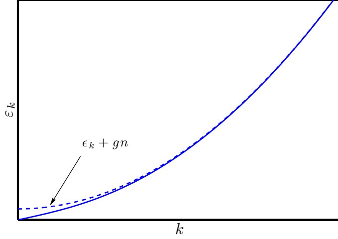
Figure 1.1: Spectrum of Bogoliubov excitations. The solid line shows the energy \epsilon_k , the dashed line shows \epsilon_k + gn .
