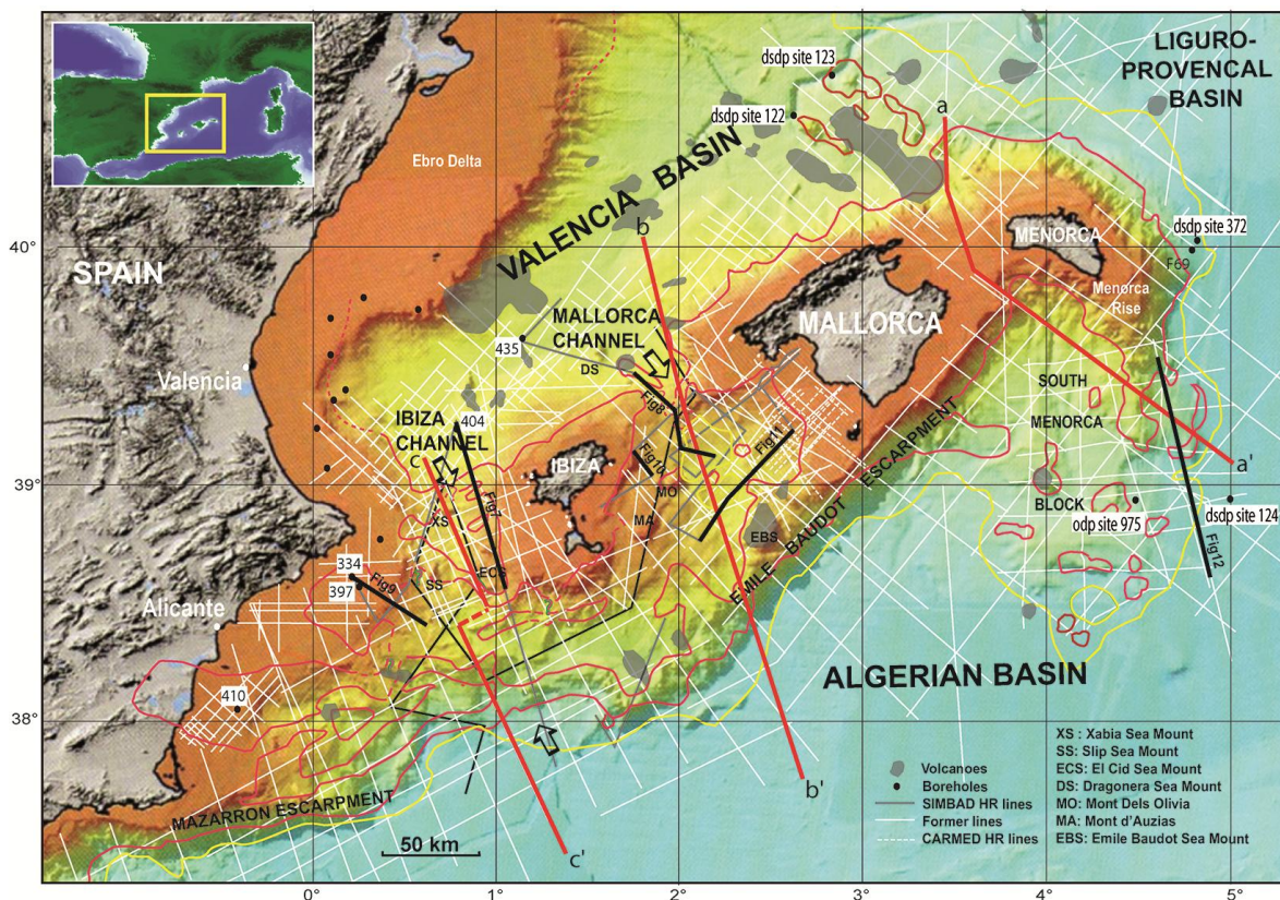
Figure IV. 2: Bathymetric map after Brossolo and Mascle, 2008, showing location of the study area. The seismic profiles used in this study are shown as well as the location of lines aa', bb' and cc' (Fig. IV.4). The thick black lines show the location of the following figures.
