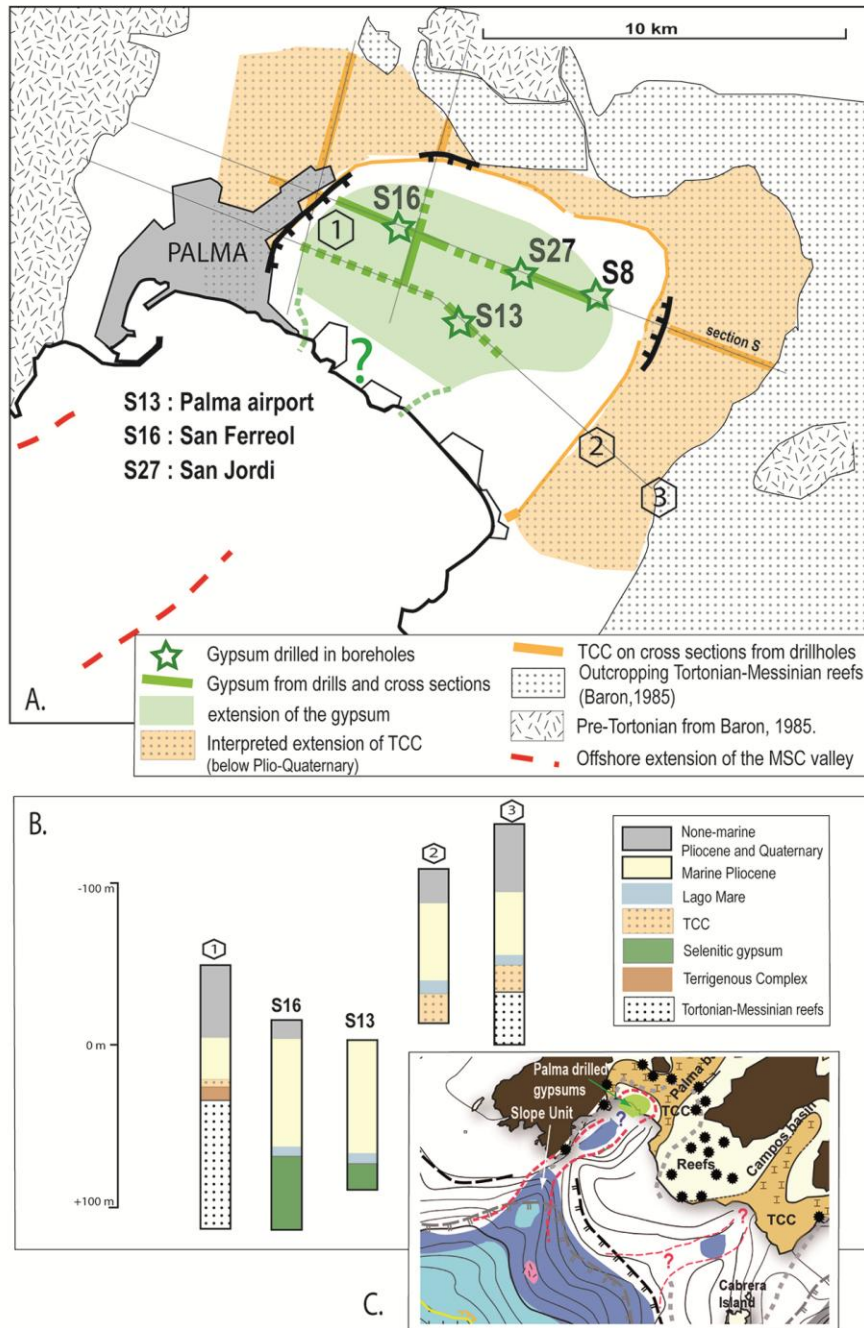
Figure IV. 24: A: map of the onland Palma depression, inferred from drilling information, and former cross-sections and maps (Baron y Gonzalez, 1984; Baron and Gonzalez, 1985). The map shows the outcropping formations after removal of the PQ unit. The light black lines indicate the locations of the sections used, the green stars the locations of boreholes where gypsum is found. B: schematic interpretation of drill hole logs simplified from Mas and Fornos, 2011. Location of the wells is given on map A. C: the location of both Messinian
