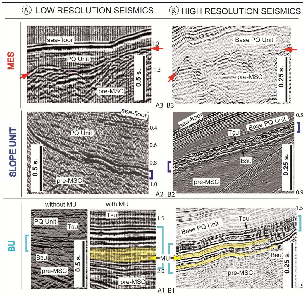
Figure IV. 18: Sections showing the different seismic facies of the MSC units and the MES in the study area, based on the available low-resolution (column A) and high-resolution
