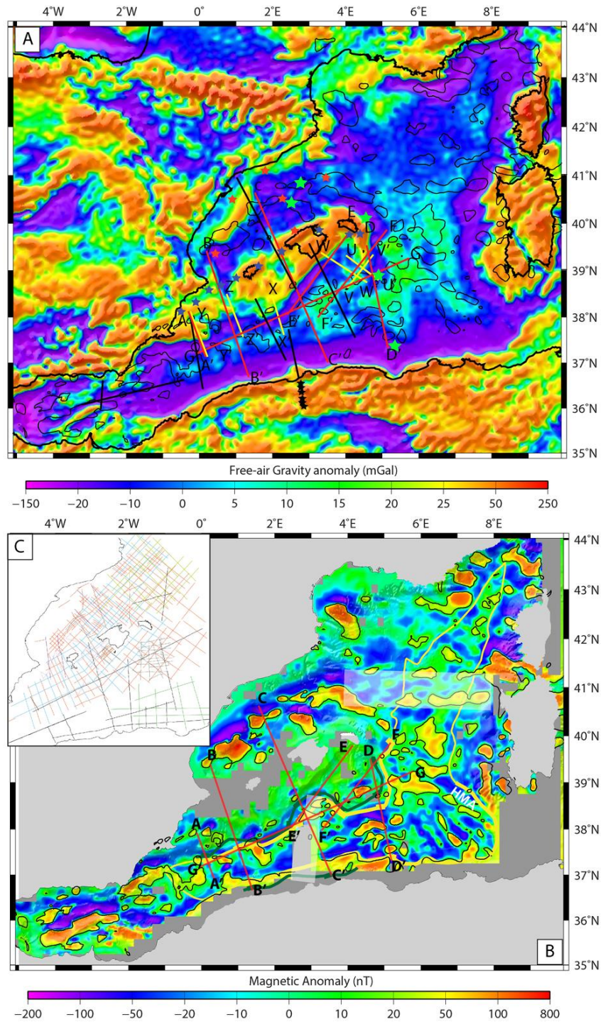
Figure III. 26: A. Free-air gravity anomalies (from Bonvalot et al., 2012), showing crustal data. Black lines: ESCI profiles (Gallart et al. 1994; Vidal et al., 1998), Meteor Profiles (Huebscher et al. 2010), and Spiral Profile (black stars on-shore, Lepretre et al. 2012). Blue stars: Banda et al. (1980) Red lines: gravity models from this study. Yellow lines: seismic profiles. B. Magnetic anomalies (from Galdeano and Rossignol, 1977). Contours show magnetic values higher than 20 nT. The two white boxes highlight two gaps between the different aeromagnetic surveys and thus anomalies interpolated from scarcer data points). The
