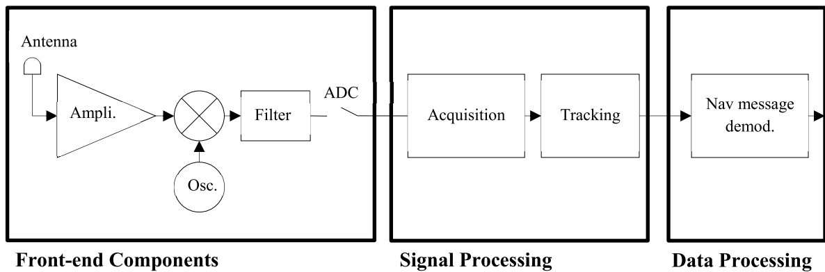
Figure 44: Real GNSS receiver block diagram
