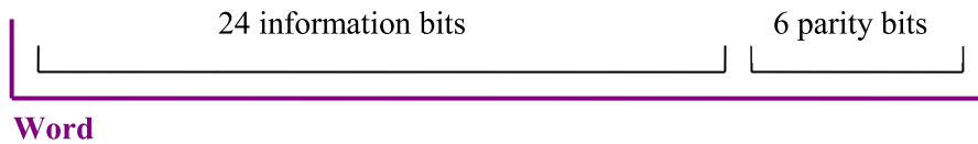
Figure 3: GPS L1 C/A navigation message word structure
