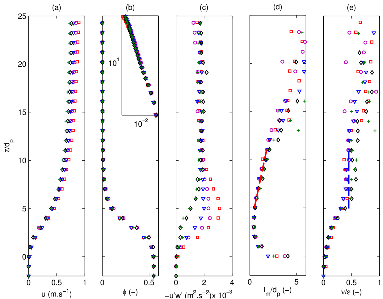
FIGURE 7.1 – Sensitivity to the non-uniformity of the flow. Mean profiles of velocity (a), concentration (b), turbulent shear stress (c), mixing length (d) and ratio between momentum and particular diffusivities (e) evaluated on the intervals t \in [30 - 36] s (squares), t \in [40 - 46] s (circles), t \in [50 - 56] s (triangles), t \in [60 - 66] s (diamonds), t \in [70 - 76] s (pluses). The dashed line on panel (d) represents the slope \kappa = 0.2 . The dashed line on panel (e) represents the Schmidt number \sigma_s = 0.45 .
