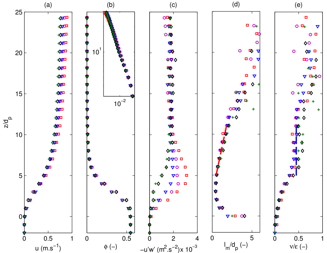
FIGURE 7.1 – Sensitivity to the non-uniformity of the flow. Mean profiles of velocity (a), concentration (b), turbulent shear stress (c), mixing length (d) and ratio between momentum and particulate diffusivities (e) evaluated on the intervals t \in [30 - 36] s (squares), t \in [40 - 46] s (circles), t \in [50 - 56] s (triangles), t \in [60 - 66] s (diamonds), t \in [70 - 76] s (pluses). The dashed line on panel (d) represents the slope \kappa = 0.2 . The dashed line on panel (e) represents the Schmidt number \sigma_s = 0.45 .
