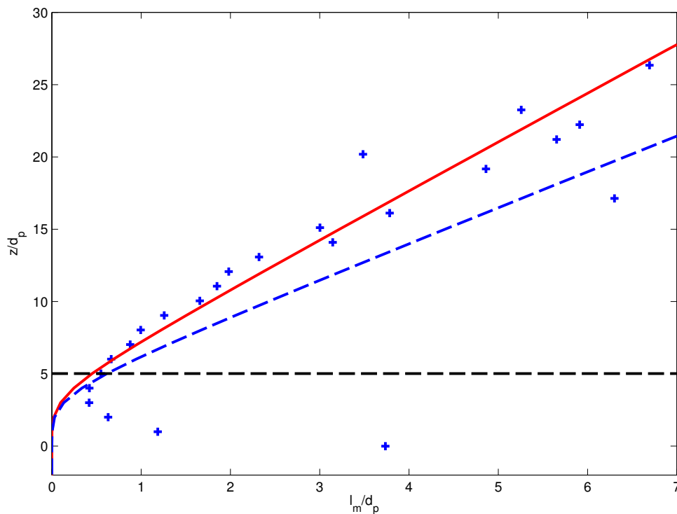
FIGURE 7.2 – Mixing length profile measured (+) and simulated from equation 4.3 of the paper using \kappa = 0.41 (- - -) and \kappa = 0.3 (—). The measured concentration profile is used here to parametrise the mixing length formulation.
