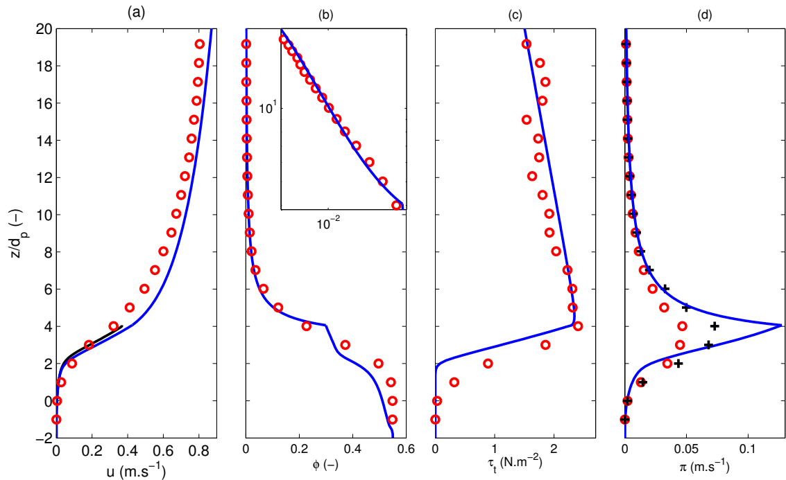
FIGURE 7.3 – Comparison between experimental measurements (o) and the results of the two-phase model (—) for the velocity profiles (the black line represents the particle velocity profile) (a), the concentration profiles (b), the turbulent shear stress profiles (c) and the sediment flux profiles (d). Two sediment flux profiles based on the experimental measurements are represented : the mean “real” flux (o) and the flux evaluated from the mean profiles of velocity and concentration (+).
