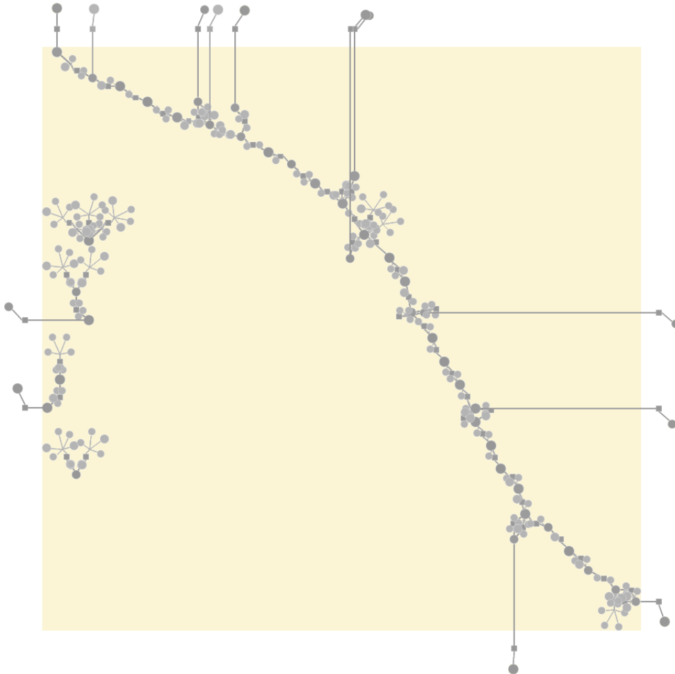
Fig. 1.2 Sixty-seven reactions happening in the peroxisome compartment of the yeast Y. lipolytica (MODEL1111190000 [Loira et al., 2012]). Reactions are represented as squares linked by edges to their reactant and product metabolites (circles). The size of the figure does not allow for readable metabolite labels, so they are omitted. The reaction graph is disconnected as the transport reactions are not shown.
