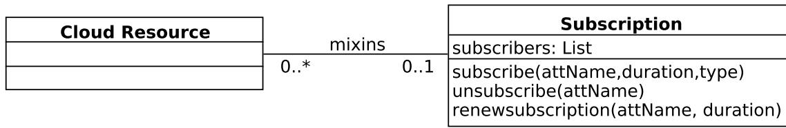
Figure 5.3: Monitoring by Subscription extension for Cloud Resources.
