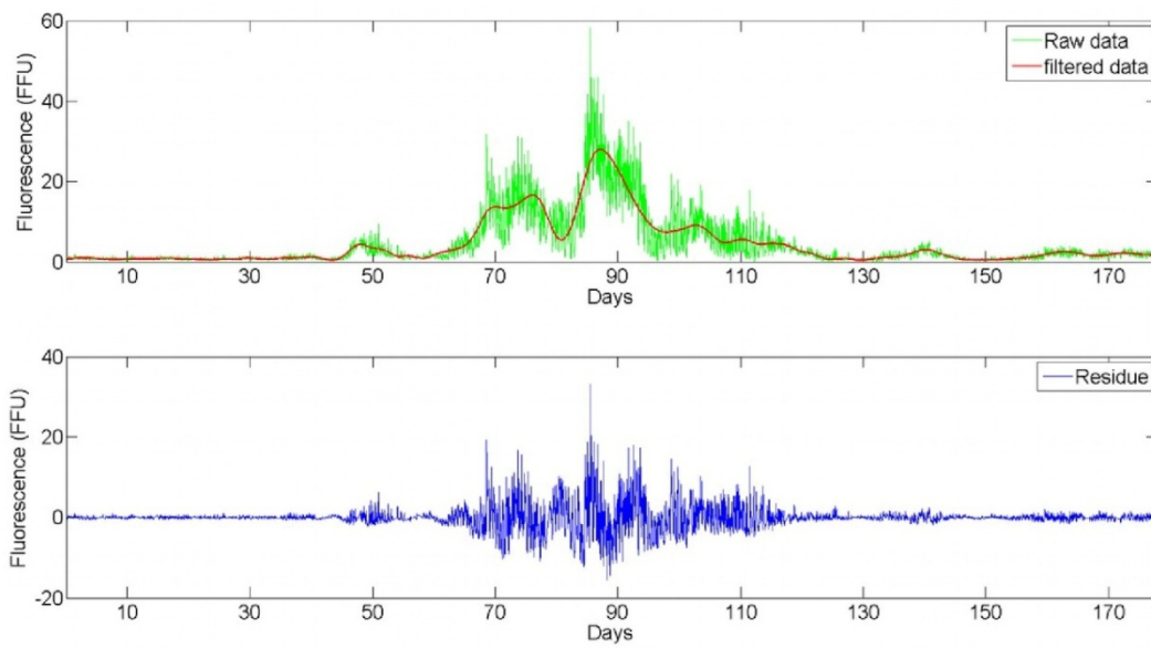
Figure 13. Raw fluorescence data for the year 2006, superposed to the trend estimated using the EMD method, modes 12 to 20, corresponding to a smoothing at scale 5 days. Below: the high frequency part, corresponding to the sum of modes from 1 to 11.
