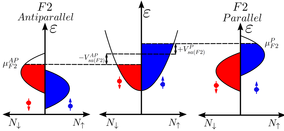
Figure 1.7: Schematic representation of the “d” band structures in the detector (F2) and the non-magnetic channel (N), for two magnetic states of F2. The spin accumulation in N can be related with the difference of voltages V_{F2}^P - V_{F2}^{AP} corresponding to P and AP configuration, in respect to the magnetization direction of the injector.
