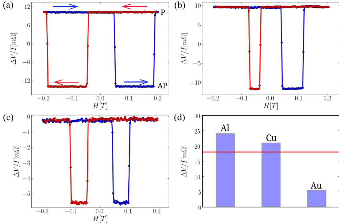
Figure 2.7: Non-local magneto-transport measurements for three types of Lateral Spin-Values with (a) Al, (b) Cu, (c) Au non-magnetic channel. Data-points were recorded at T = 77 K for the same nano-devices geometry: L = 150 nm (distance from center to center of the ferromagnetic electrodes), with nano-wires of 50 nm width. (d) Comparison of the spin signal amplitudes from three N materials. The red line representing the highest value reported in the literature [77].
