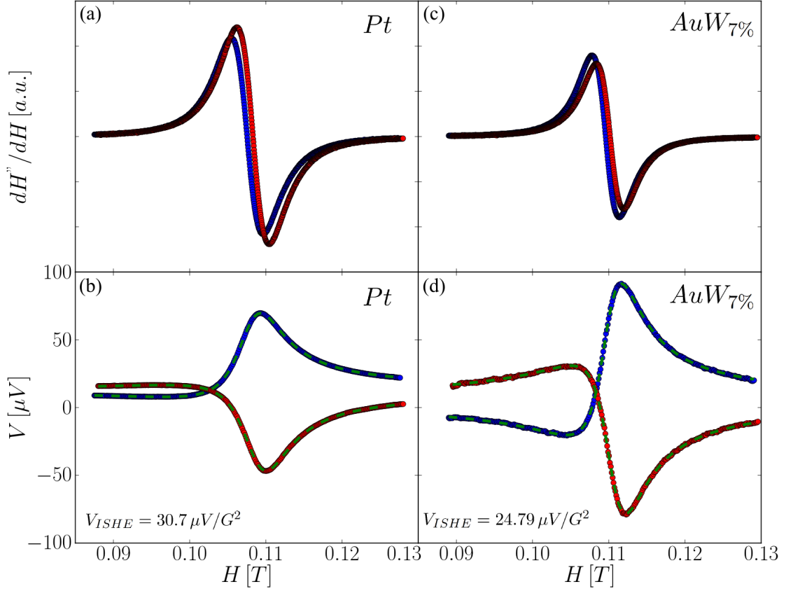
Figure 6.7: Spin pumping results corresponding to the FMR spectra and voltage measured simultaneously for (a-b) Py/Pt, and (c-d) Py/AuW 7% bi-layers. The red and blue curves stands for the parallel and anti-parallel case, respectively. The green dashed curve represents the fits according to Eq. C.1. Insets displays the inverse spin Hall voltage V_{ISHE} .
