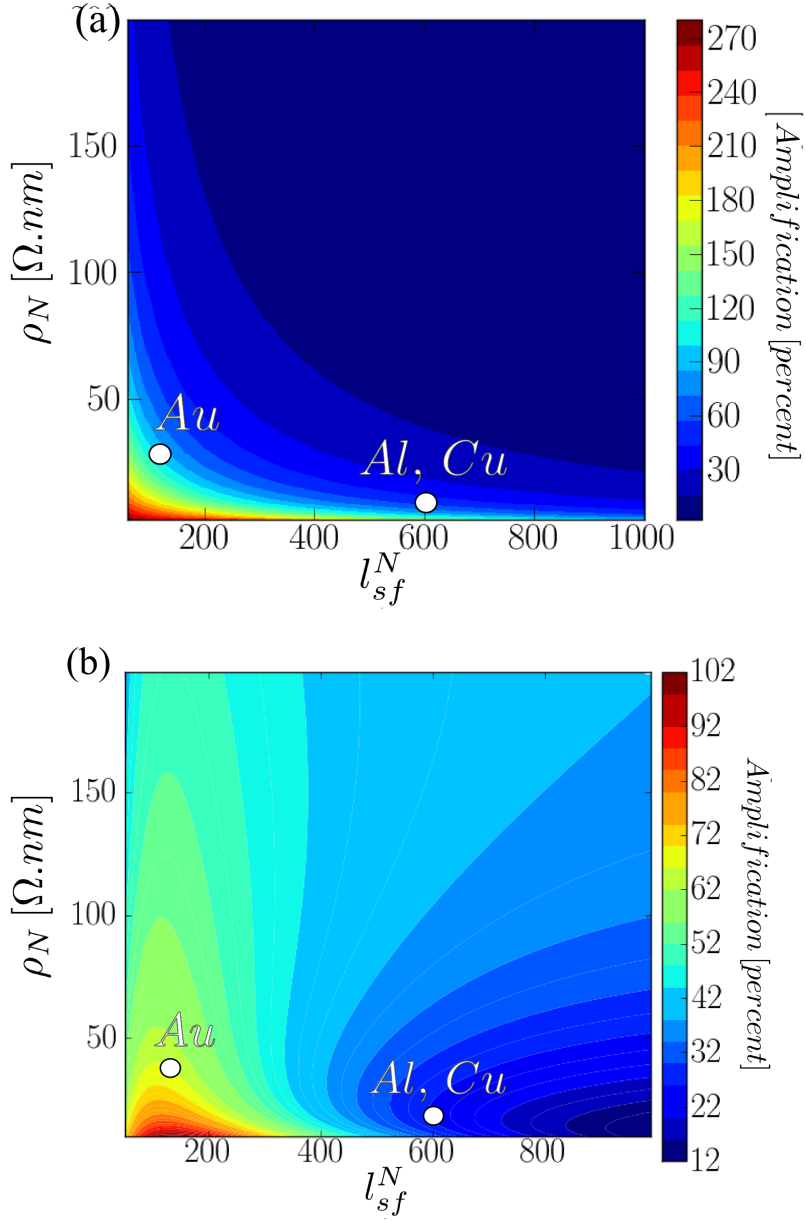
Figure 4.7: (a) Numerical calculation and (b) FEM simulations of the amplification factor as a function of l_{sf}^N and \rho_N , where the following parameters were used: L = 200 nm, w_F = 50 nm, t_F = 20 nm, \rho_F = 118 \Omega \cdot \text{nm} , w_N = 50 nm, t_N = 70 nm, P_F = 0.36 . For the FEM simulations \rho_N was varied every 1 \Omega \cdot \text{nm} , while l_{sf}^N every 10 nm, for numerical calculations these steps were 0.2 \Omega \cdot \text{nm} and 1 nm respectively.
