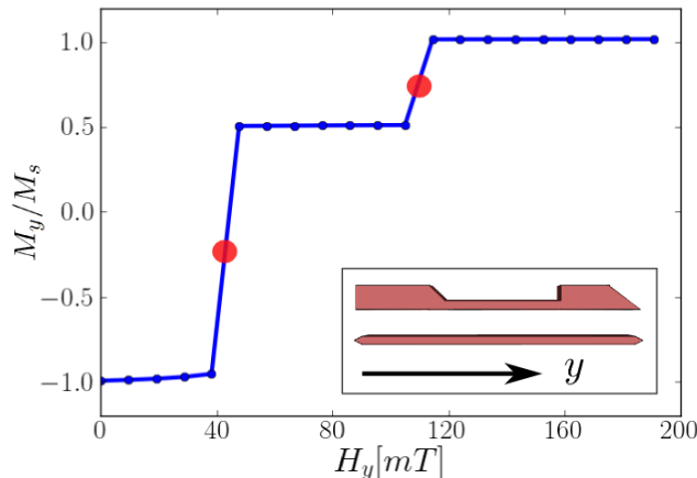
Figure 2.11: Micro-magnetic simulation by OOMMF of the magnetization curve of the two ferromagnetic contacts. Two distinguish switching fields (marked by red circles) at 40 mT and 110 mT correspond to the wire with the reservoir and the straight one, respectively. Figure in the inset represents the sketch of the studied geometry of Py nano-wires. The field is applied along the wire axis ( y ), with a small in-plane misalignment (2%).
