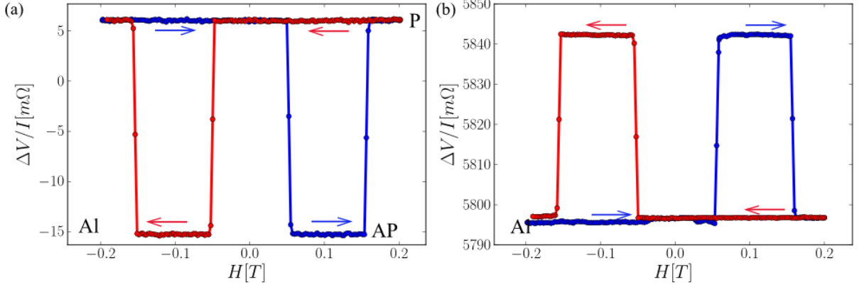
Figure 2.8: V/I measurements in (a) the Non-Local and (b) Local (GMR) probe configurations (shown in Fig. 2.3(b-c)) recorded at T = 77 K , for Py/Al nano-device made using the multi-angle evaporation method. The distance from center to center of the ferro-magnetic electrodes is equal to L = 200 nm .
