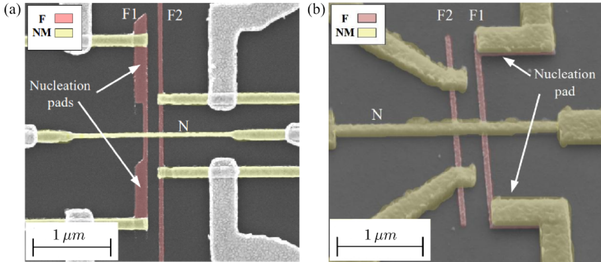
Figure 2.2: SEM images of the Lateral Spin-Valve nano-structure made by (a) multi-angle evaporation technique and (b) multi-level technique (cf. Section 2.3). Two ferro-magnetic ( F ) 15 nm thick nanowires are connected by a non-magnetic ( N ) 60 nm thick channel. One of the magnetic stripes ( F1 ) contains nucleation pads in order to facilitate the domain wall nucleation process leading to the lowering of its reversal field.
