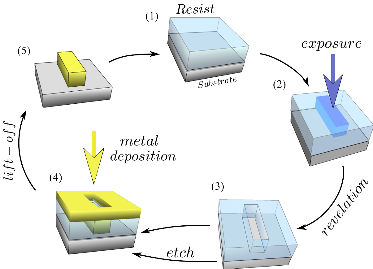
Figure B.1: Schematic representation of the nano-fabrication procedure cycle, consisting of (1) resist deposition on the Si substrate, (2) e-beam lithography exposure of the desired pattern, (3) revelation of the resist, (4) material evaporation, and (5) the lift-off process.
