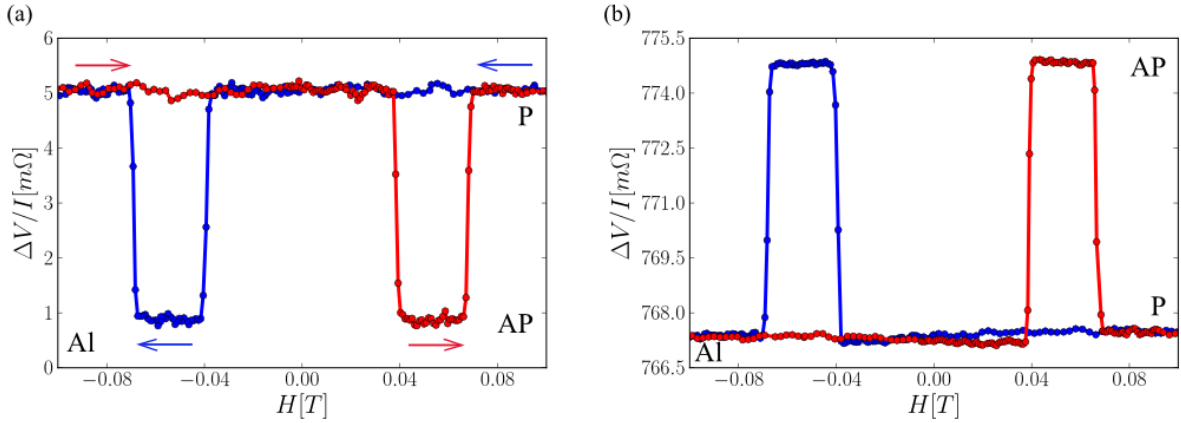
Figure 2.4: V/I measurements in (a) Non-Local and (b) Local (GMR) probe configurations shown in Fig. 2.3(b-c), recorded at T = 77 K for Py/Al nano-device made using the multi-level nano-fabrication method. The distance from center to center of the ferro-electrodes is equal to L = 200 nm . The amplitude of variation is (a) 4.16 m\Omega and (b) 7.55 m\Omega for Non-Local and Local configuration respectively [cf. Fig. 2.3(b-c)]. Blue and red curves correspond to positive and negative magnetic field sweep directions.
