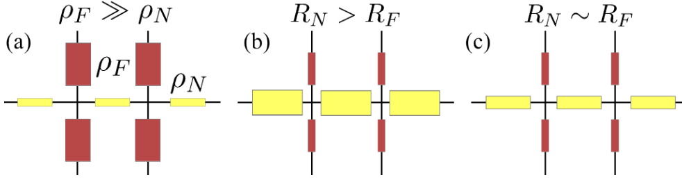
Figure 4.1: Electric circuit schematics of the lateral spin-valve nano-structure for (a) charge and (b-c) spin current. The normal (spin) resistances are represented by red and yellow squares for ferro-magnetic and non-magnetic material respectively, and their size reflects the value of the resistance attributed to flowing charge/spin current. In the case of the spin current circuit two cases are represented: (b) R_N > R_F^* which is valid for Py/Al and Py/Cu, and (c) R_N \sim R_F^* which stands for the case of Py/Au nano-structures.
