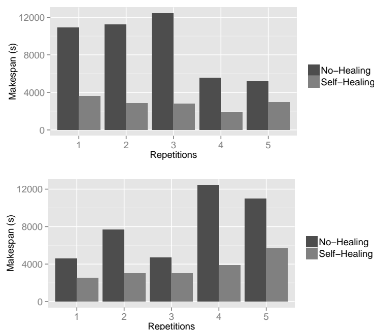
Figure 5.7: Execution makespan for FIELD-II/pasa (top) and Mean-Shift/hs3 (bottom) by using the Median Estimation method.
