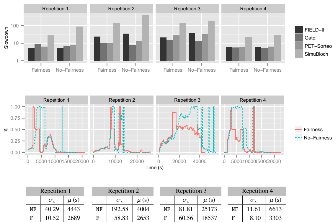
Figure 7.4: Experiment 3 (different workflows). Top: comparison of the slowdown; middle: unfairness degree \eta_r ; bottom: unfairness \mu and slowdown standard deviation.
