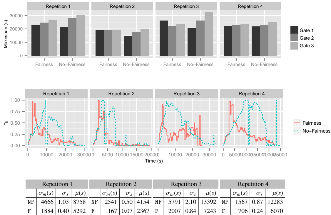
Figure 7.2: Experiment 1 (identical workflows). Top: comparison of the makespans; mid: unfairness degree \eta_u ; bottom: makespan standard deviation \sigma_m , slowdown standard deviation \sigma_s and unfairness \mu .
