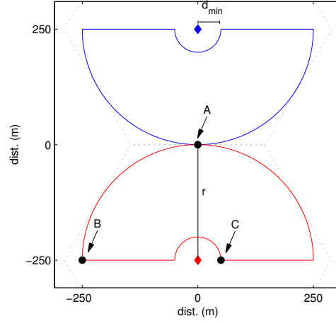
Figure 4.9: Simplified network for SIC gain bounds. Both users will be placed in the lower cell. Positions [A, B] and [C, A], represent the worst case and the best case for SIC gain respectively.
