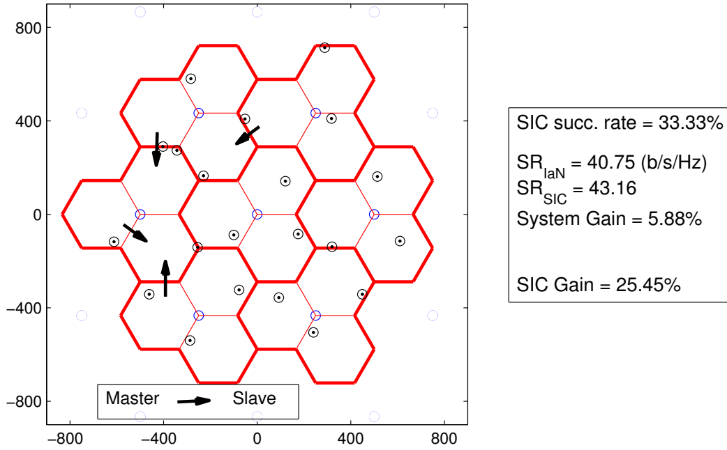
Figure 4.19: 21-cell network layout. Users are placed randomly, arrows indicate Master-Slave relations. The values on the right-hand side are calculated for this particular realization.
