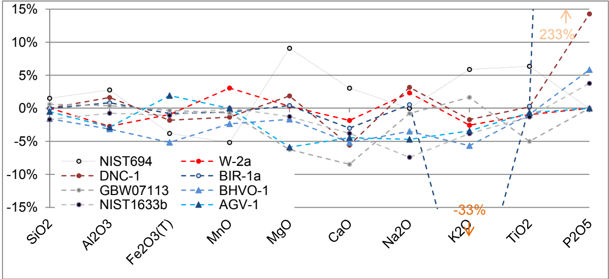
Figure II.75: Inter-comparison of the relative deviation to certified value for the reference materials included in the actlabs serie.
