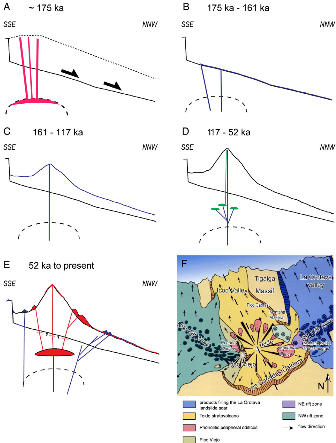
Fig. 8. New model of evolution for the T–PV complex. The map shown in subset F is modified after Navarro (2004).
