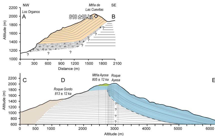
Figure 3: Geological map of the Cho Marcial Volcano zone, displaying all the ages available. The diamond corresponds to the sample JCD-576 of Carracedo et al. (2011). The triangles are ages of Ancochea et al. (1990). The direction and value of the dip of the formations measured on the field are reported. Synthetic cross sections across the northern flank of the CMV and the pre-landslide serie underlying the Ayosa formation are shown.
