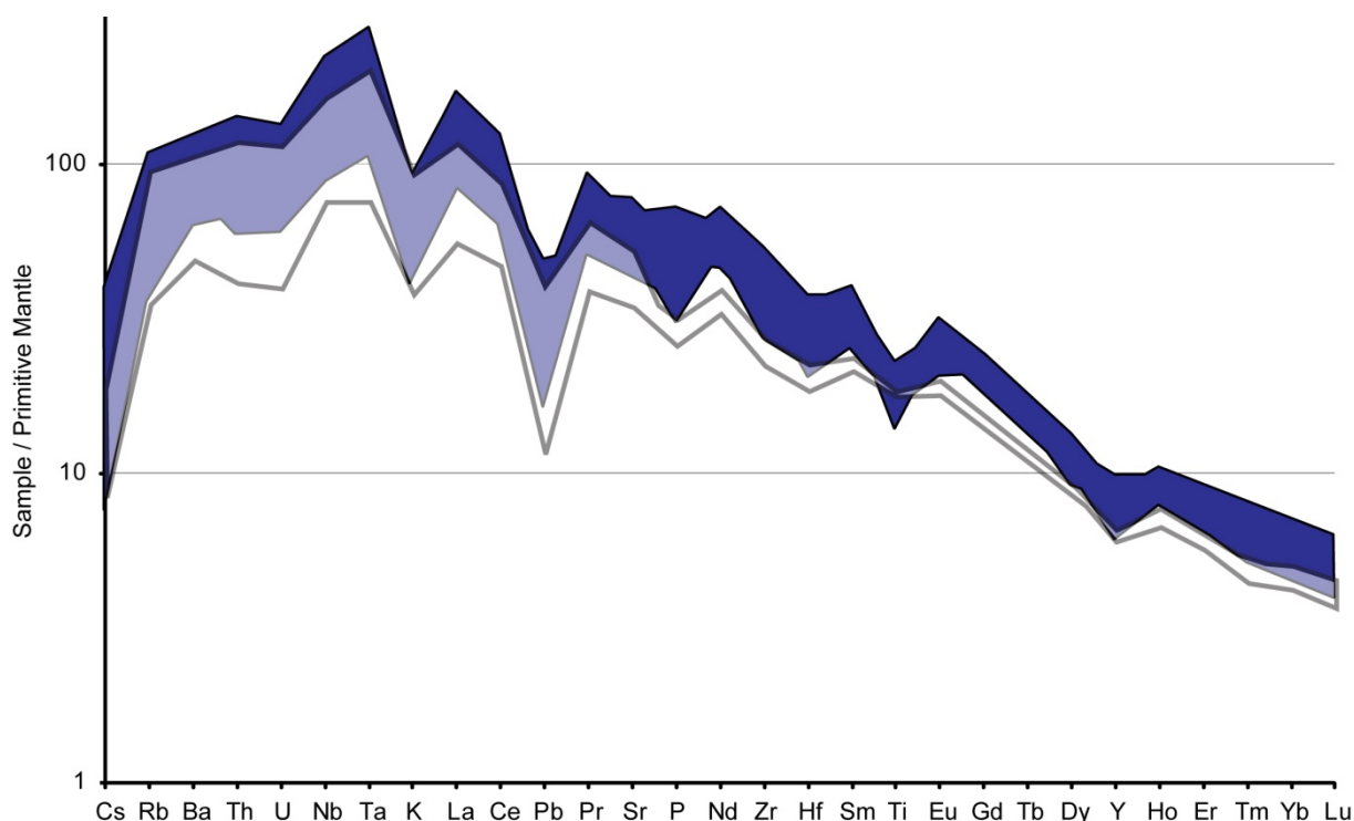
Figure 8: Spidergrams of the analysed mafic lavas. Normalization to the primitive mantle after McDonough and Sun (1995). The hollow field corresponds to the analysed basalts (n=6). The blue field corresponds to the composition range for the basanites (n=46, including 16 analysis from the literature)
