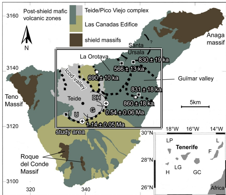
Figure 1: Simplified geological map of Tenerife showing the main edifices of the island, after Ablay and Marti (2000), modified. Previous ages of Ancochea et al. (1990), Cantagrel et al. (1999) and Carracedo et al. (2011) are reported with circled crosses, circle, and squares, respectively. The white squares stand for samples of the pre-landslides units, while the black squares stand for the landslide scar filling units. The names and limits of the 3 main inferred calderas are from Marti et al. (1997): U: Ucanca, G: Guajara and DH: Diego Hernandez. Dashed lines stand for the limits of the landslide scars. The black and white frame shows the extension of Figure 2. Map of the archipelago in inset; L: Lanzarote, F: Fuerteventura, GC: Gran Canaria, LG: La Gomera, LP: La Palma, H: El Hierro. Coordinates in kilometers from the Spanish national grid (UTM).
