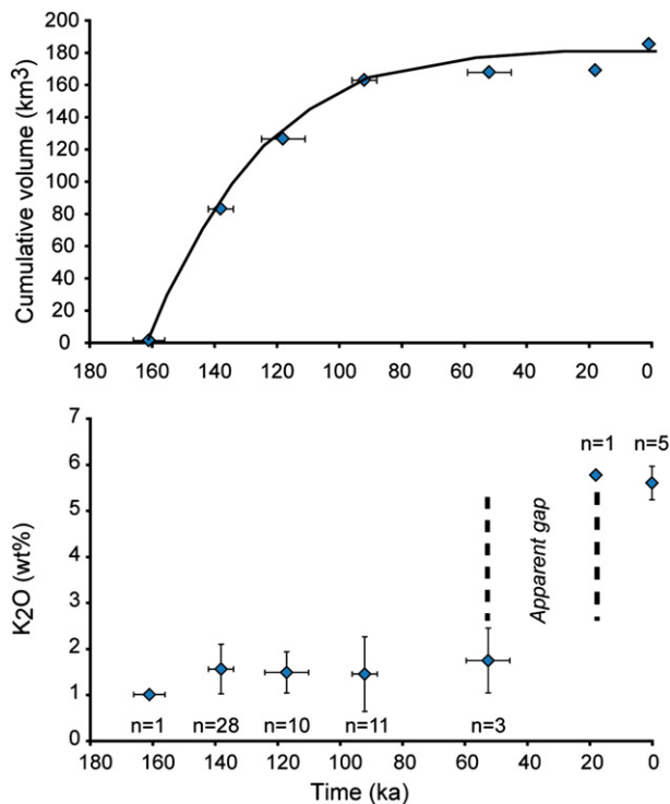
Fig. 6. Cumulative volume and average K 2 O computed for the T–PV complex post-landslide volcanic succession at successive time steps. The number of samples ( n ) taken into account to calculate the mean K 2 O and its associated standard deviation (shown as vertical error bars) are indicated at each step.
