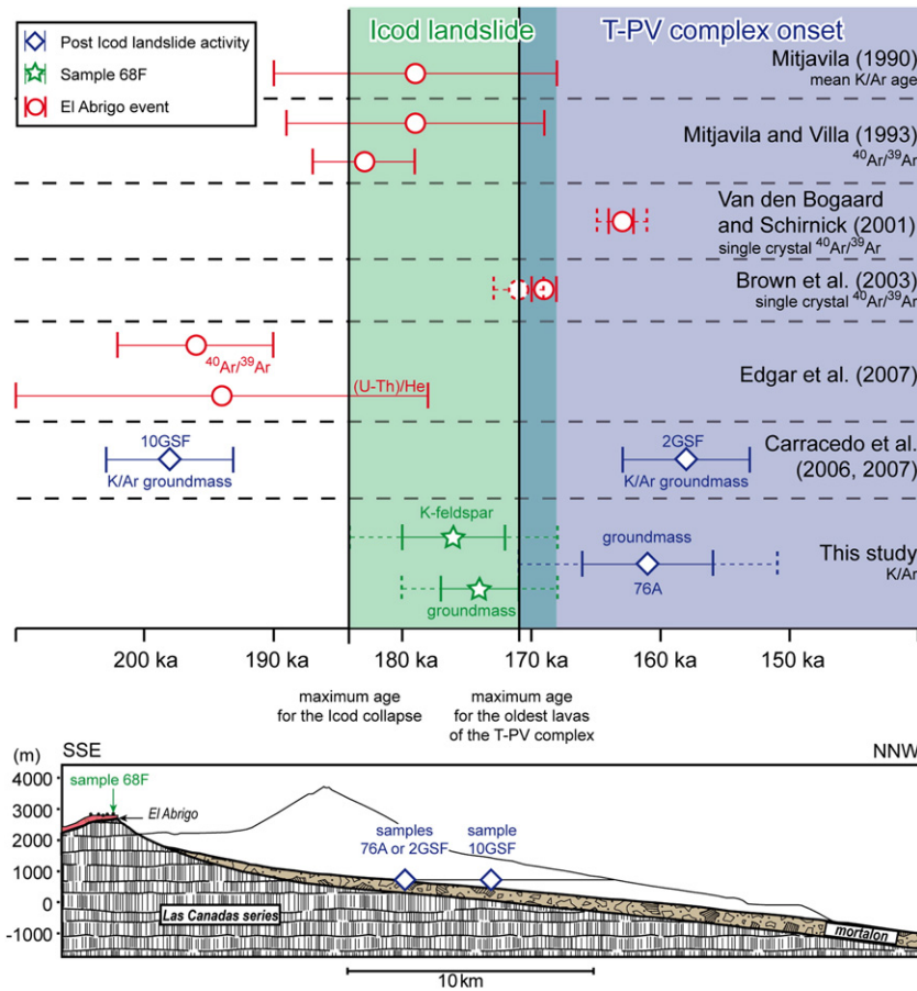
Fig. 7. Summary of the available geochronological data relevant to the determination of the age of the Icod landslide event. All the data at 2\sigma : dashed lines represent recalculated error bars for the present study and Brown et al. (2003). The green zone highlights the period during which the Icod landslide occurred. The blue zone stands for the post-collapse activity.
