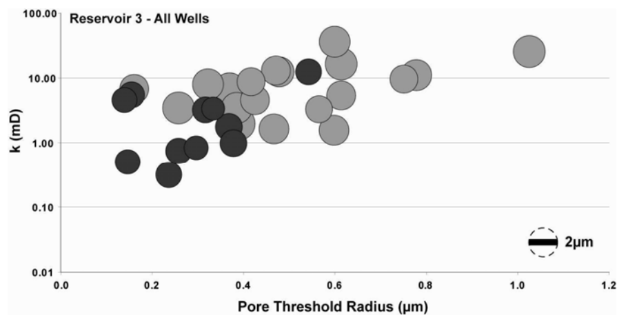
Figure 7.11: Mean pore throat radius (PTR) versus permeability for strictly microporous samples from the Reservoir 3 (Mishrif Formation). The diameter of the discs represents the 2D crystallometry of the particles (see scale bar). Fine micrites (crystallometry < 2\mu\text{m} – in black) with low permeability values are invariably associated with small micropores less than 0.5\mu\text{m} on average. Contrariwise, coarse micrites (crystallometry > 2\mu\text{m} – in grey) are associated with higher permeability.
