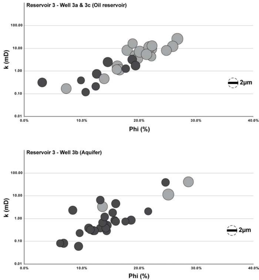
Figure 7.10: Porosity versus permeability (measured on plugs) and associated crystallometry for strictly microporous samples of three wells of Reservoir 3 (Mishrif Formation). The diameter of the discs represents the crystallometry of the particles; (see scale bar). Black discs represent fine (crystallometry < 2\mu\text{m} ) micrites, and grey discs coarse (crystallometry of 2\text{--}4\mu\text{m} ) micrites. Well 3a and 3c (oil reservoir) have a predominance of coarse micrites, whereas Well 3b (aquifer) has a predominance of fine micrites. Fine micrites are associated with the lowest petrophysical properties: porosity and permeability are generally less than 20% and 10mD, respectively.
