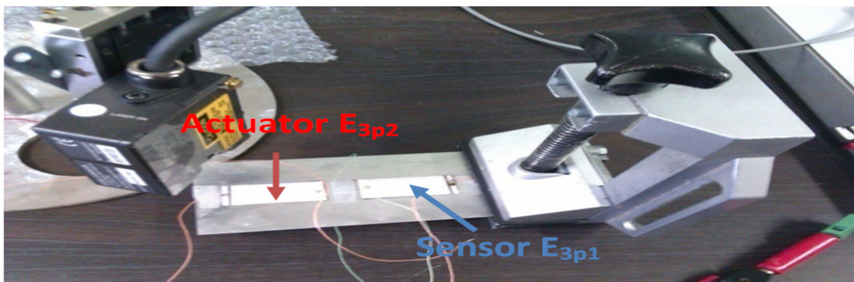
Figure 7.3: Piezoelectric transformers
