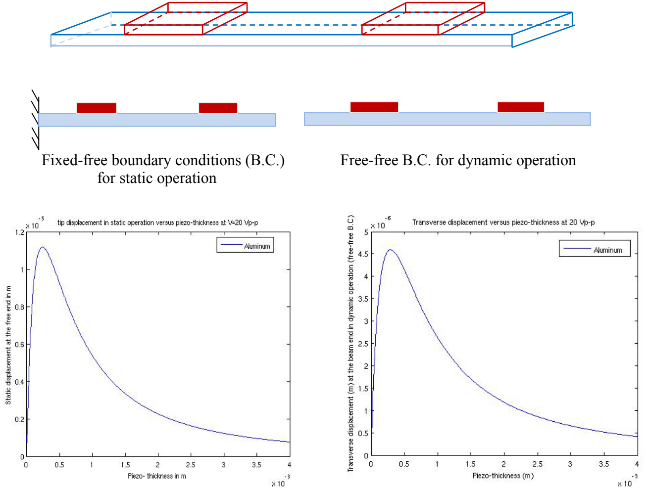
Static and dynamic transverse displacement at the free end versus piezoelectric thickness
