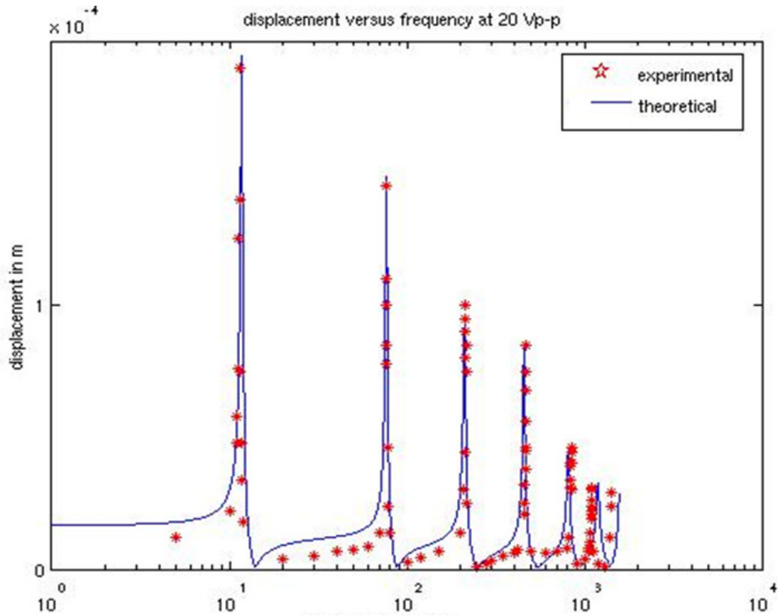
Figure 4.13: Tip displacement of the beam versus frequency
