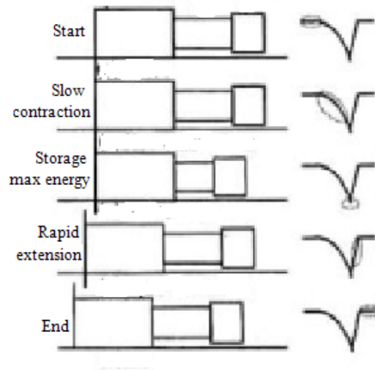
Figure 1.12 : impact drive principle [ (Stepping principles, 2010)]
