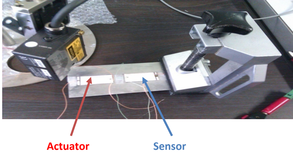
Figure 4.21: Piezoelectric actuator-sensor functionality
