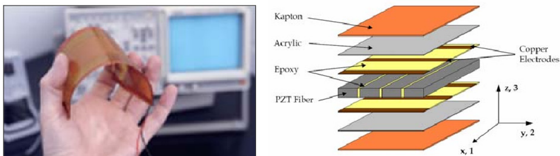
The Macro Fiber Composite (MFC) actuator. Left: A demonstration of the flexibility of the actuator. Right: Layers of the actuator. [ (Bilgen, 2007)]
