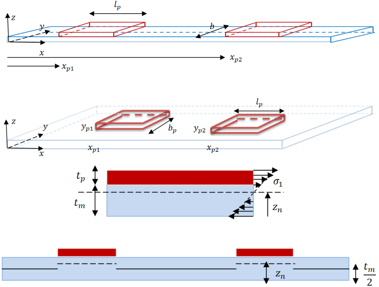
Figure 3.7: Geometric parameters for the system (top figures) and schematic figures for the position of the neutral axis (plane) in the case of this asymmetric studied system (bottom figures).
