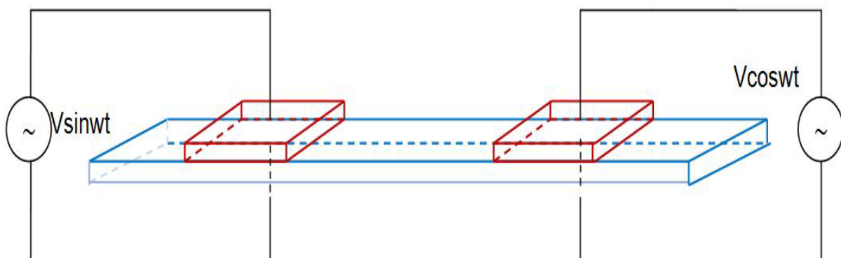
Schematic figure of the two modes excitation: 2ME
