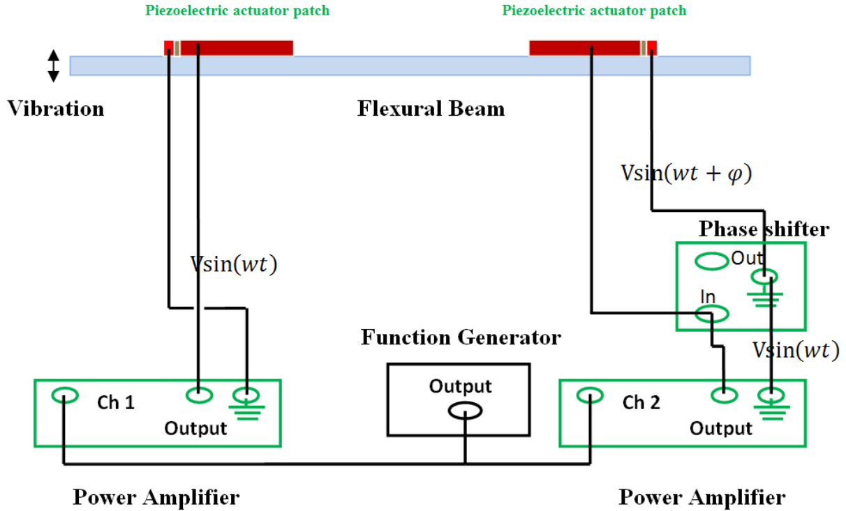
Figure 6.4 : configuration of the two modes excitation
