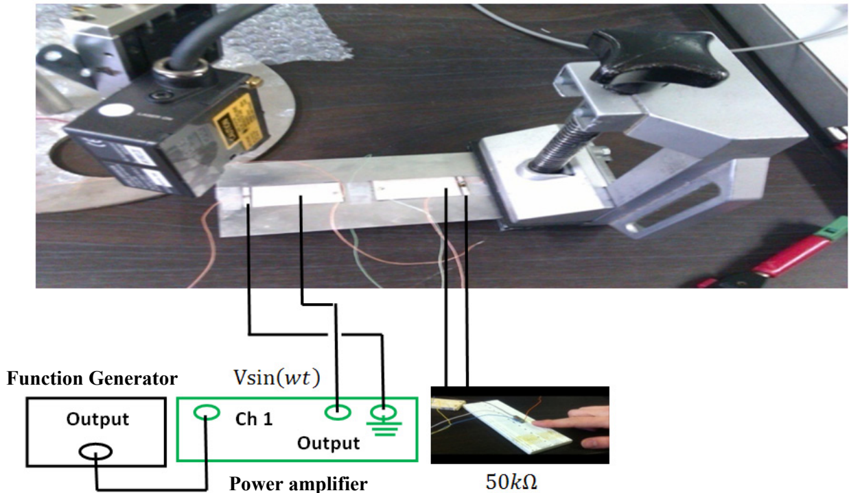
Figure 7.9: Experimental setup case of resistance shunt circuit
