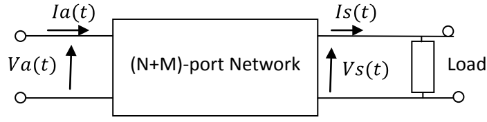
Figure 7.21: (N+M) port-network for thin plates with non-collocated piezoelectric patches actuators/sensors
