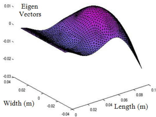
mode order 5
