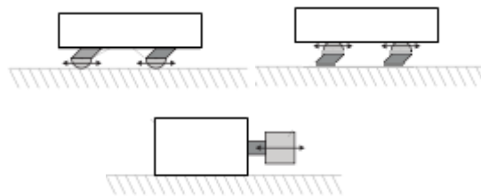
Figure 1.10: inertial drive design
