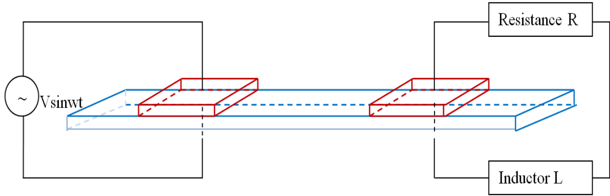
Figure 5. 19: Operation principle of the one mode excitation
