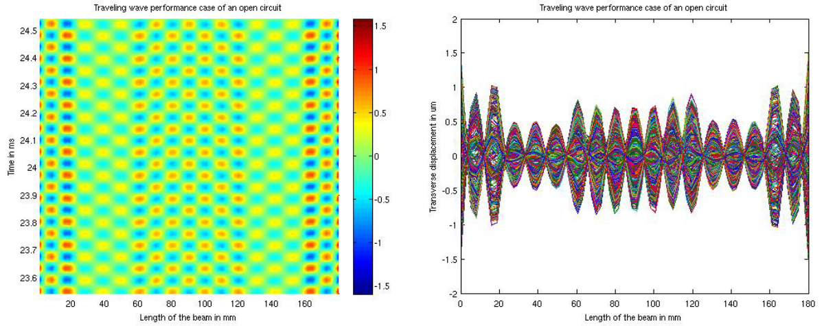
Figure 5.30: Wave performance case of an open circuit
