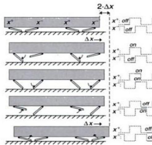
Figure 1.2 : mechanisms (Robot motion) [(Ebefors, et al., 2005)]
