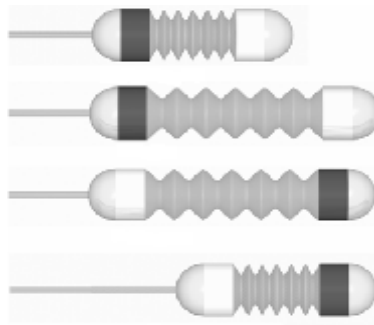
Figure 1.6 : Inchworm principle (slider motion) [(May, 1975.)]
