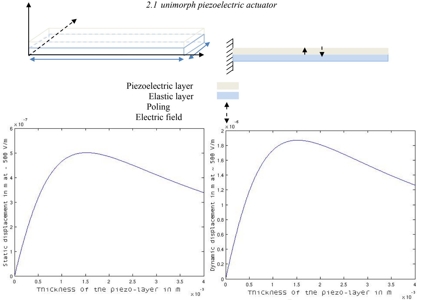
Static (left) and dynamic (right) transverse displacement at the free end of the unimorph piezoelectric actuator
