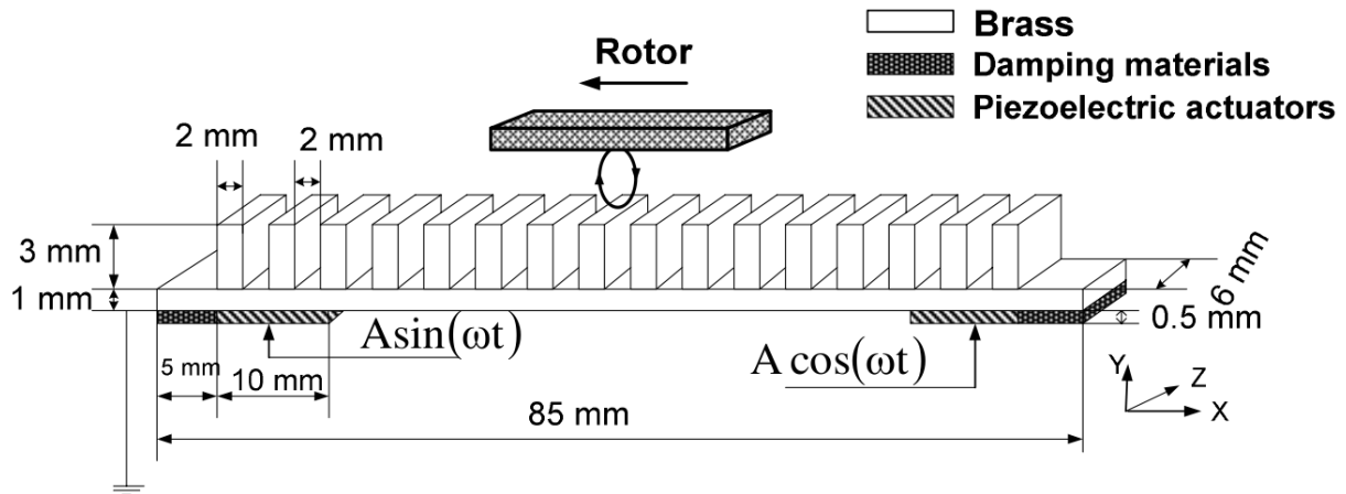
Figure 5. 5: The schematic diagram of the dual piezoelectric actuators ultrasonic linear motor presented by (Suybangdum, et al., 2009)
