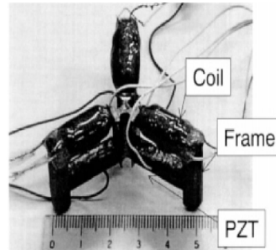
Figure 1.9: Inchworm locomotion examples [(Codourey, et al., 1995) & (Torii, et al., 2001)]
