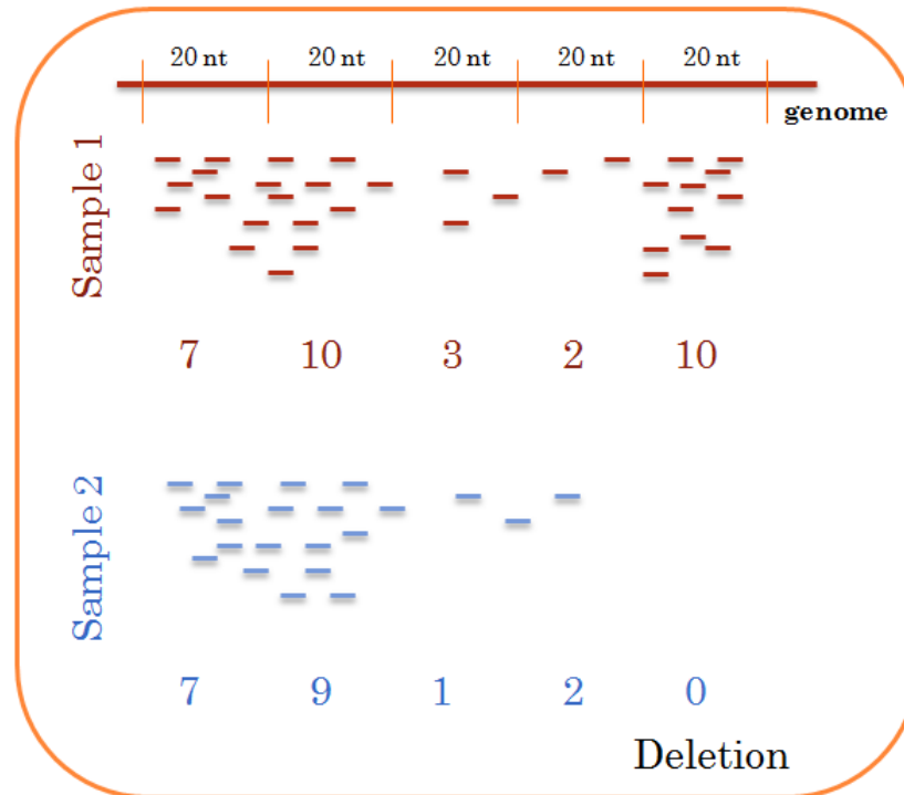
Figure 20: Micro deletion detection. A coverage-based method where the number of reads in a sliding window of 20nt is computed across the genome for each sample and then this coverage is compared to the coverage of the same window in a randomly selected sample. In the first window from right, there is a deletion in sample 2, as the depth of coverage in sample 1 is 10 reads whereas the depth of coverage is 0 in sample 2.
