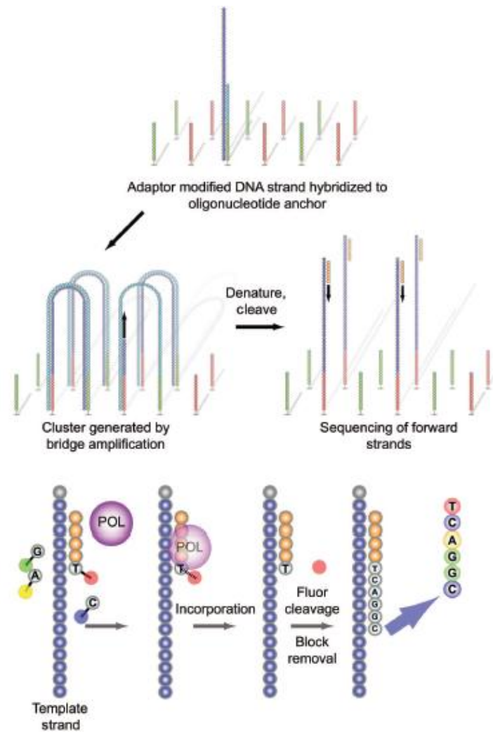
Figure 9: Illumina sequencing technology. Genomic DNA is fragmented randomly and adaptors are ligated to both ends of fragments. Single strand fragments are bound randomly to the surface of the flow cell channels. Bridge amplification is started by adding unlabeled nucleotides and enzyme. Nucleotides are incorporated by enzyme to make double-stranded bridges. Single-strand templates anchored to the surface are made by denaturation. Several million dense clusters of double-stranded DNA are generated in each channel of the flow cell. Four labeled reversible terminators, DNA polymerase and primers are added to initiate the sequencing cycle. The emitted fluorescence from each cluster is captured after laser excitation and the nucleotide is identified. The sequencing cycles are repeated to identify the nucleotides in a fragment, one base at a time. The data are aligned and compared to a reference genome, and nucleotide differences are identified.
