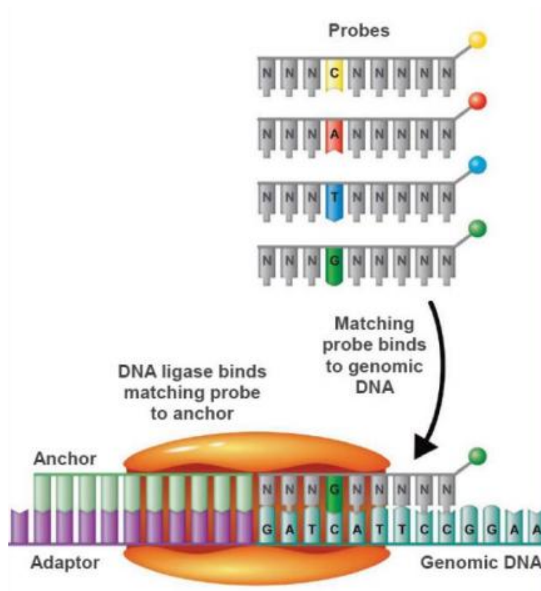
Figure 13: The complete genomics sequencing technology. a) Multiple adaptor library construction process: paired-end DNA libraries consist of genomic DNA fragments with adaptors interspersed within the genomic DNA at regular intervals. The adaptors act as initiating points for reading up to 10
