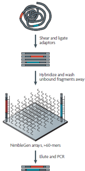
Figure 6: Solid-phase capture and enrichment. Adaptor sequences are ligated to fragmented genomic DNA. After stringent washing to remove non-selected fragments, the enriched targets are eluted, PCR amplified and sequenced.
