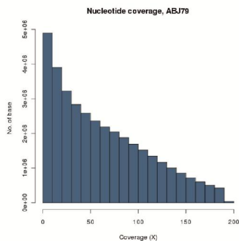
Figure 27: Sequence coverage for targeted nucleotides in ABJ75 and ABJ79. Most of the nucleotides have depth of coverage more than 60 times in both samples.
