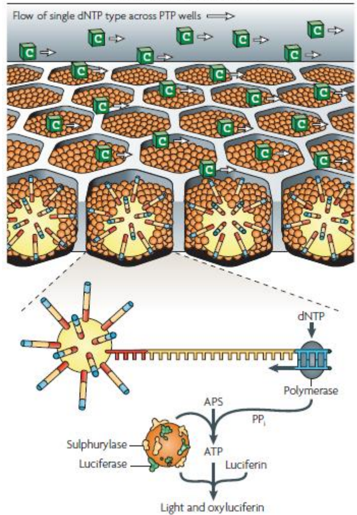
Roche/454 — Pyrosequencing 1-2 million template beads loaded into PTP wells
