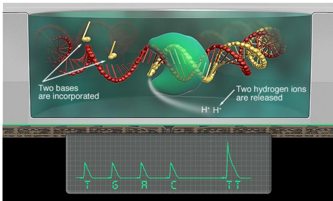
Figure 12: Semiconductor sequencing using in Ion torrent platform. a) When one nucleotide is incorporated into a DNA, a hydrogen ion is released. The charge of this ion will change the pH of the solution which will be detected by ion sensors by detection of voltage change. The sequencer machine will convert the chemical information to digital information. b) The sequencer then sequentially floods the chip with one nucleotide after another. If the next nucleotide that floods the
