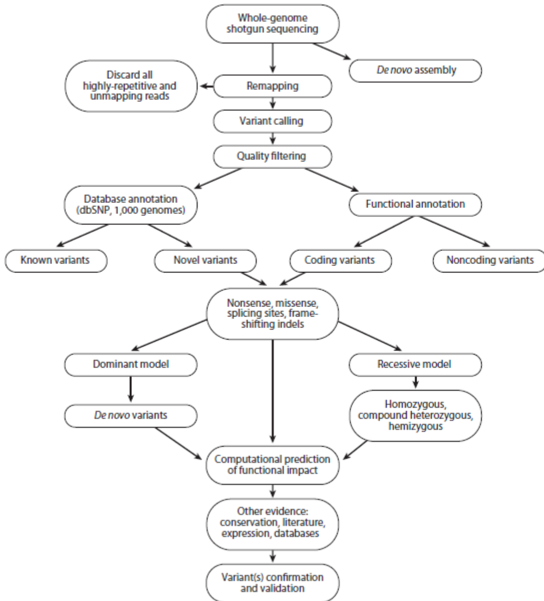
Figure 35: Schematic filtration workflow for genome as well as exome datasets. After sequencing, mapping is carried out against the human reference genome in order to obtain the list of variants. After removing low-quality variants, several filtration steps such as removing variants present in SNP databases or removing non-coding variants are performed. List of extracted variants are analyzed in different scenarios related to mode of inheritance. For few remaining candidates, more criteria such as predicted effect of change, conservation or expression profiles are taken into account in order to prioritize the variations.
