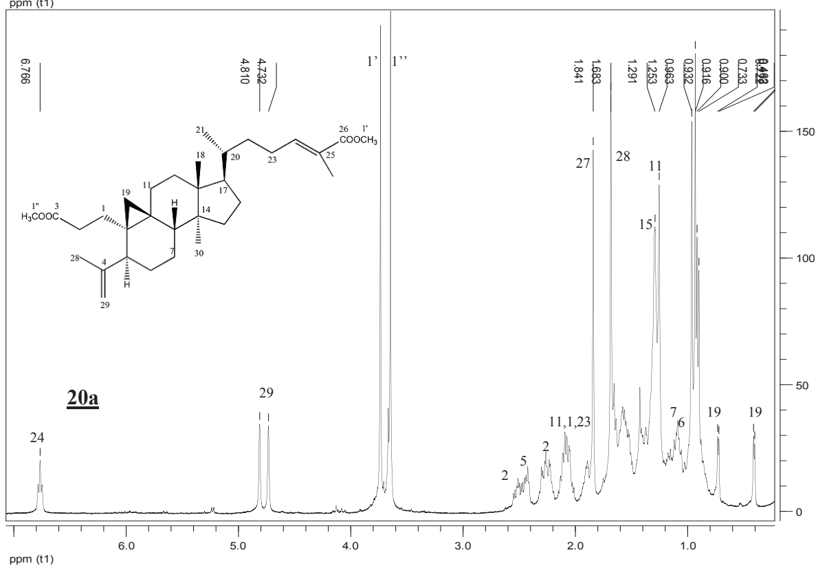
Figure 68. The ^1\text{H} NMR spectrum (300 MHz) of 20 and 20a (in \text{CDCl}_3 )
