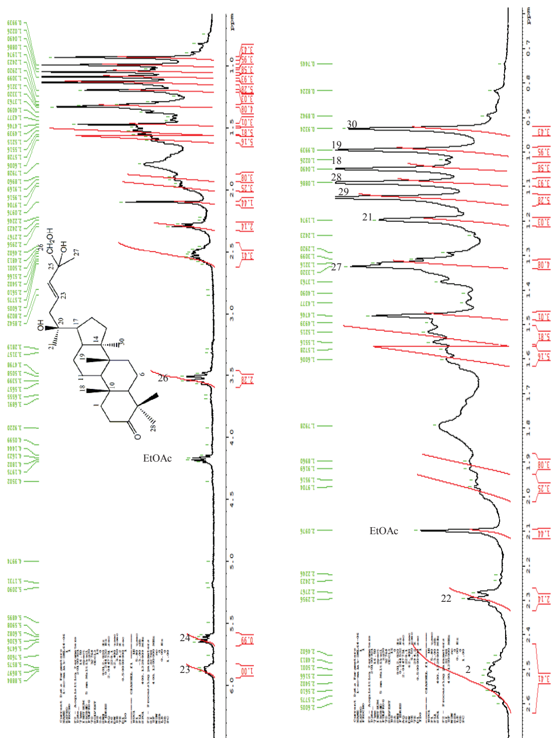
Figure 124. The 1 H NMR spectrum (300 MHz) of 46 (in CDCl 3 ) and expanded spectrum in the range of 0.7-2.7 ppm.
