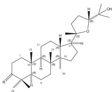
R=O ocotillone ( 34 )
