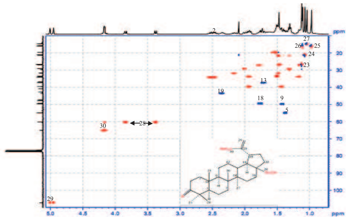
Figure 47. Expanded HSQCedited spectrum of 16 (in CDCl 3 ) in the range of \delta_H 0.7-5.1 ppm and \delta_C 10-110 ppm.
