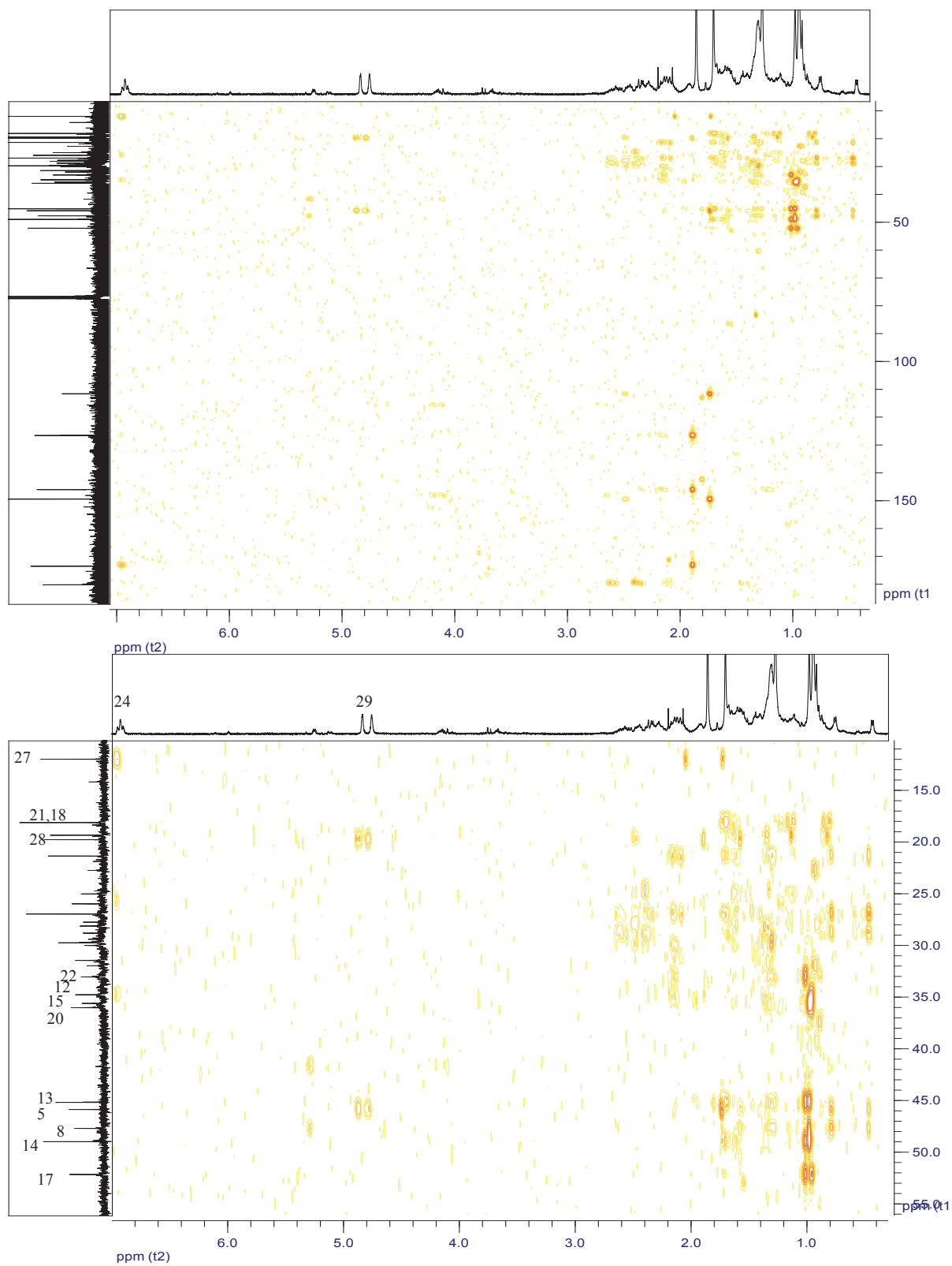
Figure 67. The HMBC correlation of 20 (in CDCl_3 ) and expanded spectrum in the range of \delta_H 0.3-7.0 ppm and \delta_C 10-56 ppm.
