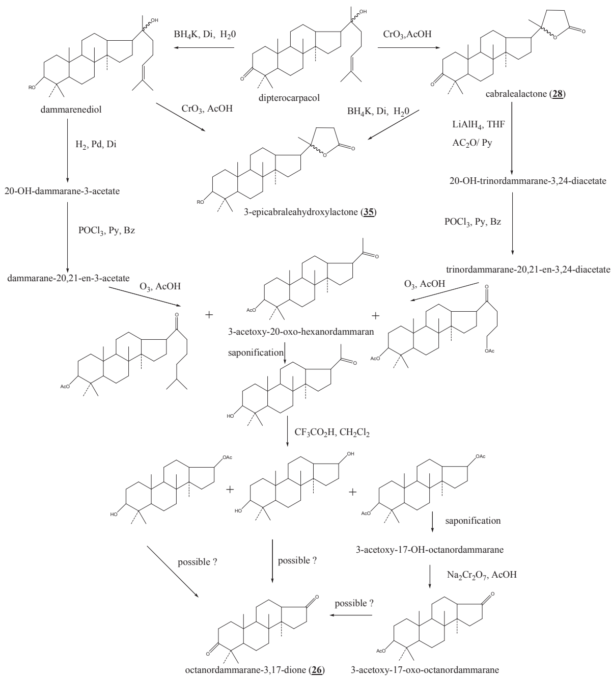
Scheme 22. Semisynthesis of cabralealactone ( 28 ), 3- epicabraleahydroxylactone ( 35 ) and 3β-acetoxy-17-oxo-octanordammarane from diptercarpol ( 22 ) [70, 229, 235]
