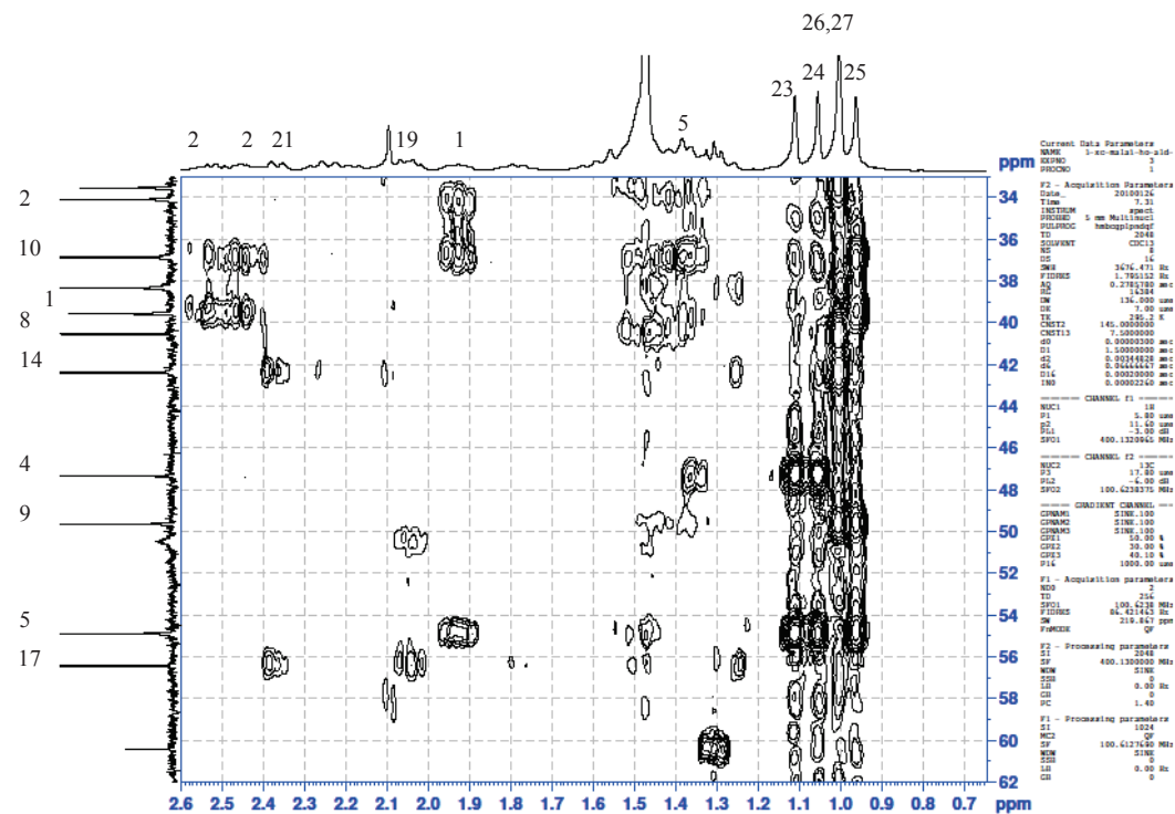
Figure 44. The HMBC correlation of 14 (in \text{CDCl}_3 ). a) whole spectrum b.) expanded HMBC spectrum in the range of \delta_{\text{H}} 0.7-2.6 ppm and \delta_{\text{C}} 33-62 ppm.
