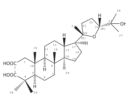
(20 S ,24 R )-20,24-epoxy-25-hydroxy-2,3-secodammarane-2,3-dioic acid ( 47 )***
