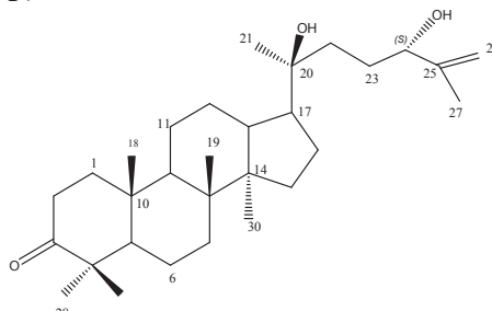
(20 S ,24 S )-20,24-dihydroxydammar-25-en-3-one ( 38 )
