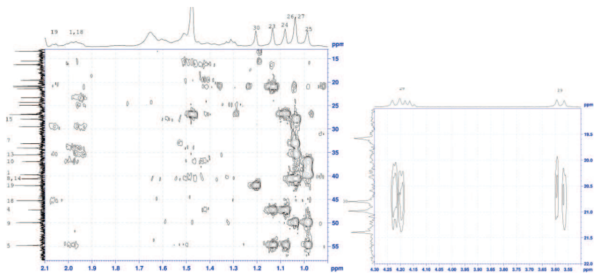
Figure 104. The HMBC correlation of 36 (in \text{CDCl}_3 ) and expanded spectrum in the range of \delta_{\text{H}} 0.9-2.1 ppm, \delta_{\text{C}} 13-58 ppm and \delta_{\text{H}} 3.5-4.3 ppm, \delta_{\text{C}} 19.5-22.0 ppm.
