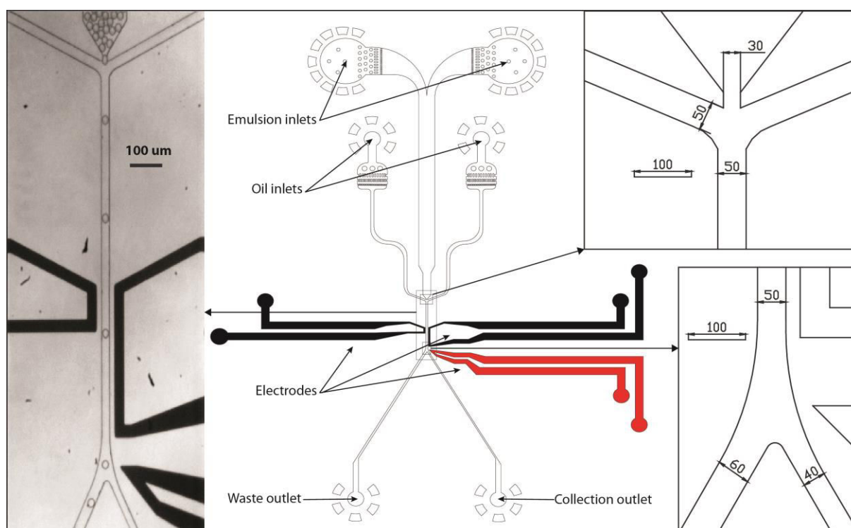
Figure 52. Microfluidic device for fluorescence-activated droplet sorting. Depth 25 \mu\text{m} . The dimensions of all device features are indicated in \mu\text{m} .
