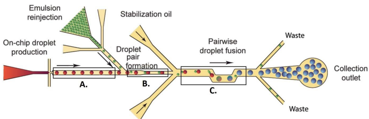
Figure 58. Passive fusion technique. Regions on the microfluidic device: A. Unstabilized droplets before pairing; B. Pairing region; C. Zig-zag channel for fusion and stabilization.
