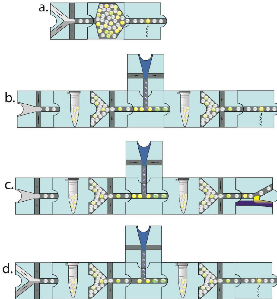
Figure 21. Microfluidic platforms for in vitro protein evolution. a) Monitoring in vitro expression of GFP. The GFP encoding genes are co-encapsulated with IVTT mixture. Produced droplets are stored in a reservoir on-chip. Green fluorescence is monitored at the outlet of the device after a certain incubation time [172]. b) Single DNA molecule isothermal amplification and analysis. Droplets containing HRCA mixture and \beta -galactosidase genes are incubated off-chip for amplification to occur. Further, droplets are fused with IVTT/substrate mixture and incubated for protein expression and substrate conversion. Successively, the fluorescent readout is performed [210]. c) In vitro screening of \beta -galactosidase. The same as b) , except the final step, where the detection has been substituted by selection of the more active variant by fusion with a continuous flow [213]. d) Kinetic analysis of in vitro translated laccase. The coupled in vitro transcription and translation (IVTT) of genes is followed, after droplet fusion, by an enzymatic assay of the translated CotA protein (laccase) [214].
