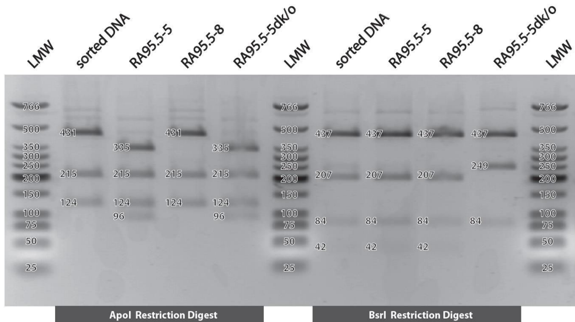
Figure 40. Agarose gel of digested DNA. Unlabeled bands represent the whole gene and partial digests.
