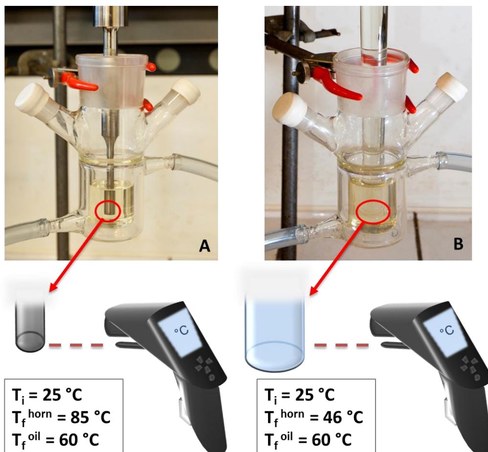
Figure II.10. Temperature assessment of both ultrasonic horns after sonication ( T_i . initial temperature, T_f . final temperature).
