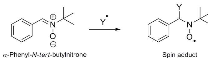
Figure II.8. The spin trapping mechanism of a free radical ( Y^\bullet ) by the \alpha -phenyl- N - tert -butylnitron.
