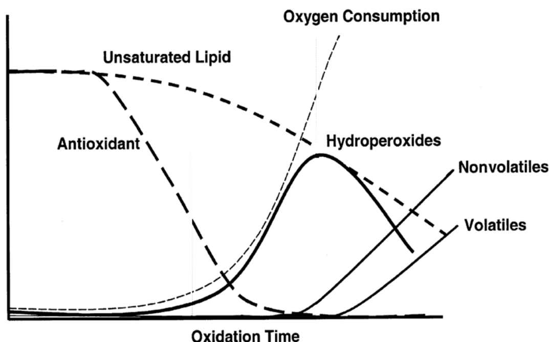
Figure II.2. Kinetic curve of autooxidation of polyunsaturated fatty acids.
