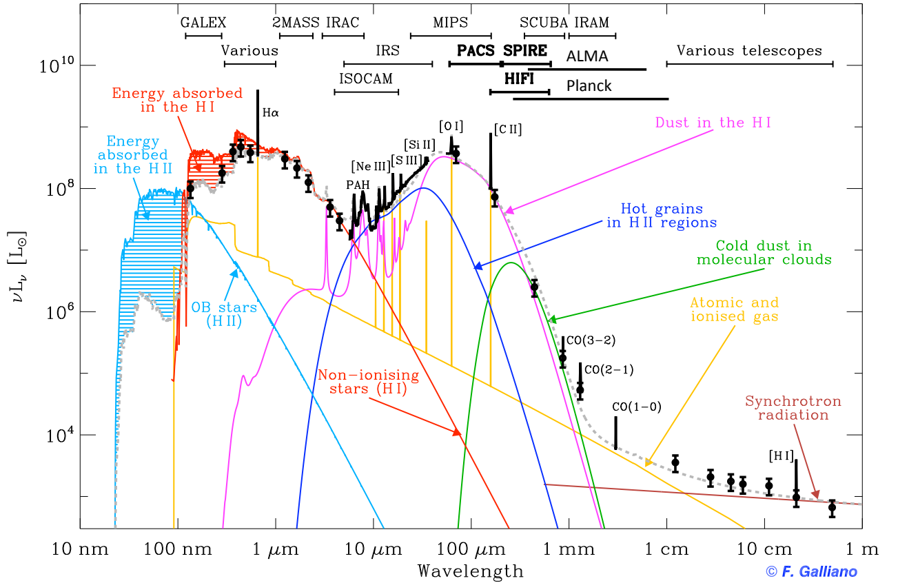
Fig. 1.15. Detailed view of the SED of a galaxy with the contributions from stars (in cyan and red), dust (in pink, green and blue) and gas (in yellow and brown). The total SED is the dashed grey line. Observations are the black points and spectrum.
