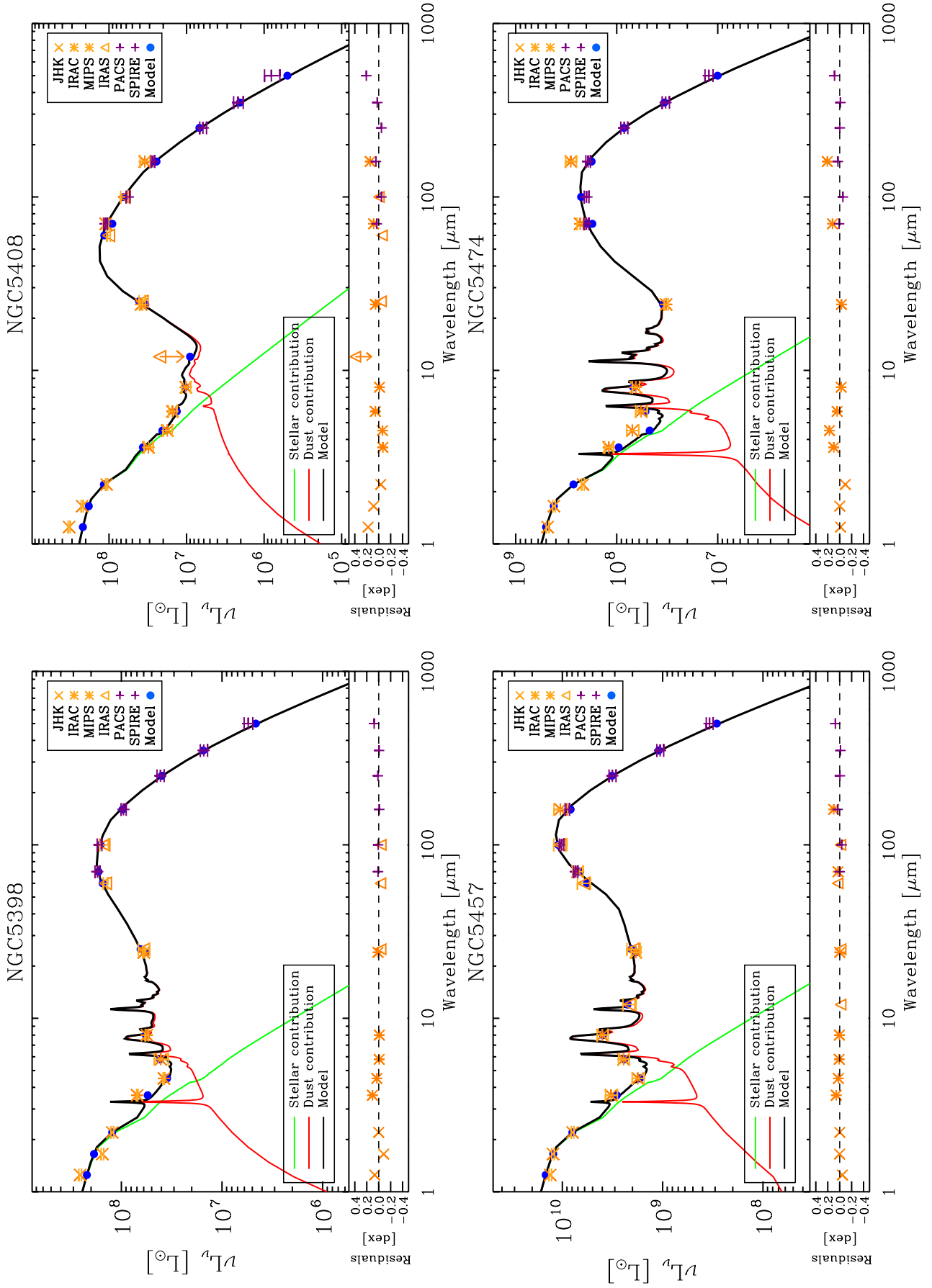
Fig. 7.24. (continued) for NGC5398 (top left), NGC5408 (top right), NGC5457 (bottom left), NGC5474 (bottom right).
