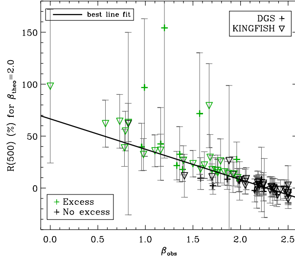
Fig. 5.11. Relative residual at 500 \mu\text{m} versus \beta_{\text{obs}} (from Section 5.3) for DGS (crosses) and KINGFISH (downward triangles) galaxies. The green symbols mark the galaxies presenting an excess at 500 \mu\text{m} . The best fit line is indicated as a solid black line, and corresponds to: R(500) = (66.6 \pm 7.1) + (-29.2 \pm 3.4) \times \beta_{\text{obs}} .
