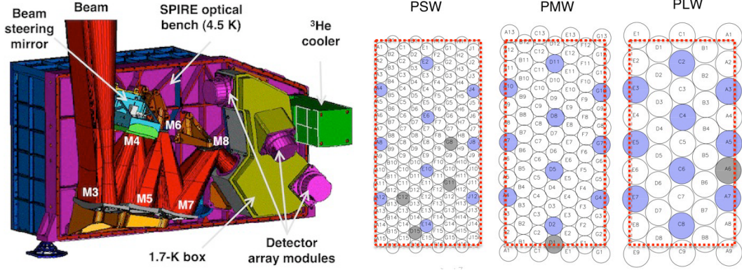
Fig. 3.7. (left) SPIRE focal plane unit on the photometer side. (right) Schematic view of the bolometers arrays. The blue bolometers are the bolometers centered on the same position on the sky for the 3 arrays. The grey bolometers are the dead bolometers. The 4' \times 8' field of view is delineated by the red dashed rectangle.
