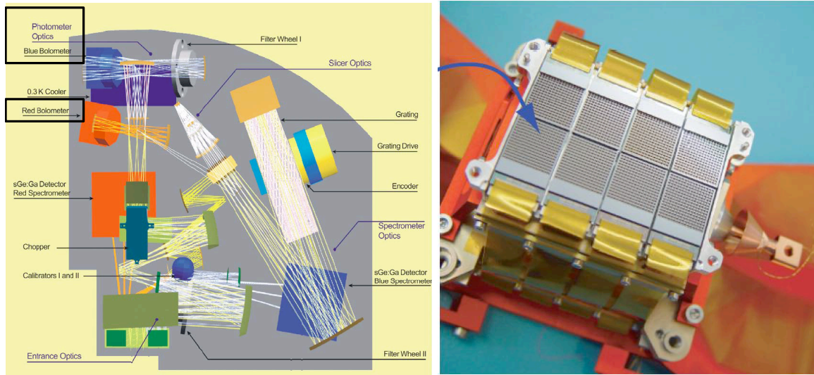
Fig. 3.4. ( left ) Optical layout of the PACS instrument. The photometer optics are on the top left of the picture (framed by the black rectangles). ( right ) Bolometer matrices of the PACS blue bolometer array. The total blue bolometer array assembly is 64x32 pixels and is composed of 4x2 monolithic matrices of 16x16 pixels, as shown here. In a similar way, the red bolometer array assembly is 16x32 pixels (2x1 monolithic matrices).
