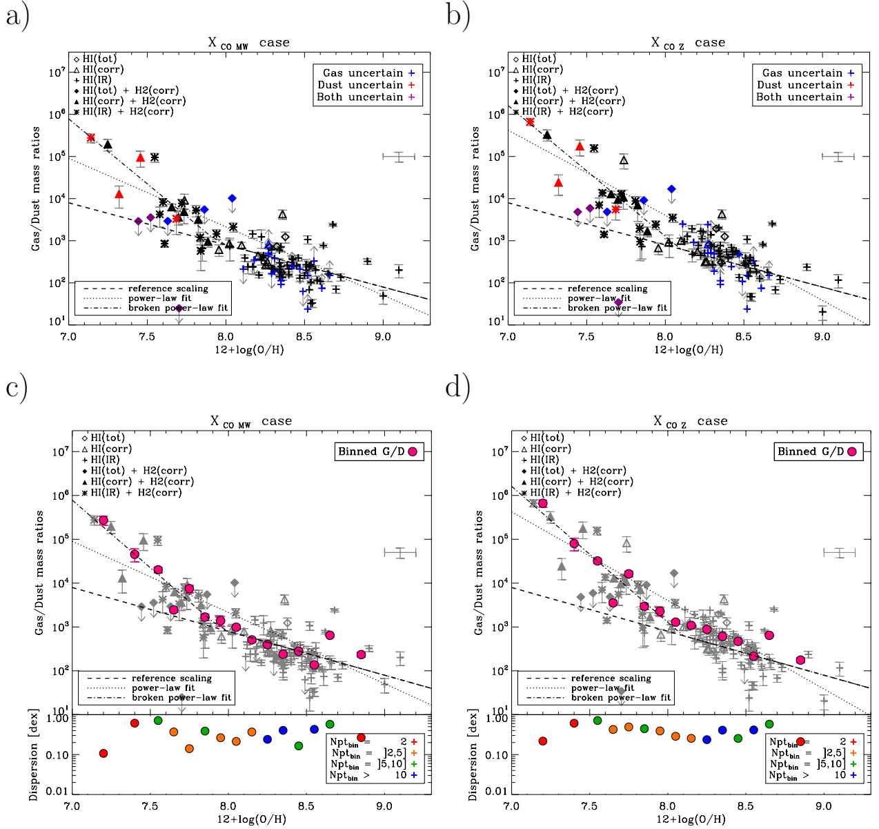
Fig. 9.4. ( Top row ): G/D as a function of metallicity for the 2 values of X_{\text{CO}} : X_{\text{CO},\text{MW}} (a) and X_{\text{CO},\text{Z}} (b). The mean error for the data points is shown in grey on the right of the plots. The colours code the reliability of the point depending if the gas mass is uncertain (in blue), the dust mass is uncertain (in red) or if both are uncertain (in purple). The symbol traces the changes made in the HI and H 2 masses (see text for details on the uncertainties and the changes on the gas masses). The dashed line represents the reference scaling of the G/D with metallicity (not fit to the data). The dotted and dash-dotted lines represent the best power-law and best broken power-law fits to the data. ( Bottom row ): Same as top row for X_{\text{CO},\text{MW}} (c) and X_{\text{CO},\text{Z}} (d), where the binned G/D values (see text) have been added as pink filled circles. For clarity, the observed G/D values are now shown in grey. On the bottom panels the relative dispersion in each bins, in terms of standard deviation, is shown and the colours show the number of galaxies in each bin.
