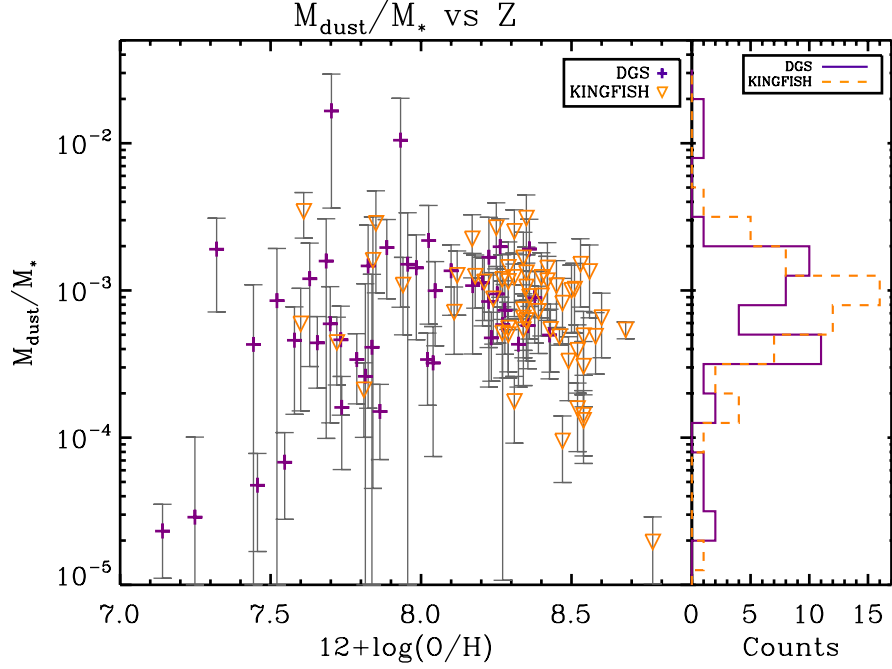
Fig. 8.5. Dust-to-stellar mass ratios for the DGS (purple crosses) and KINGFISH (orange downward triangles) samples as a function of metallicity. The distribution of M_{\text{dust}}/M_* is indicated on the side for both samples: plain purple line for DGS and dashed orange line for KINGFISH.
