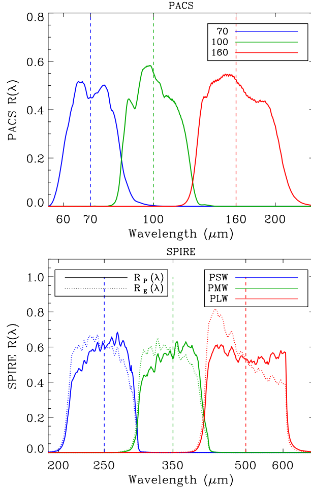
Fig. 3.9. ( top ) PACS filter transmissions, R(\lambda) . ( bottom ) SPIRE filter transmissions for point sources, R_P(\lambda) , plain lines, and extended sources, R_E(\lambda) , dotted lines (see text for details). On both plots, the dashed lines mark the reference wavelength for each band.
