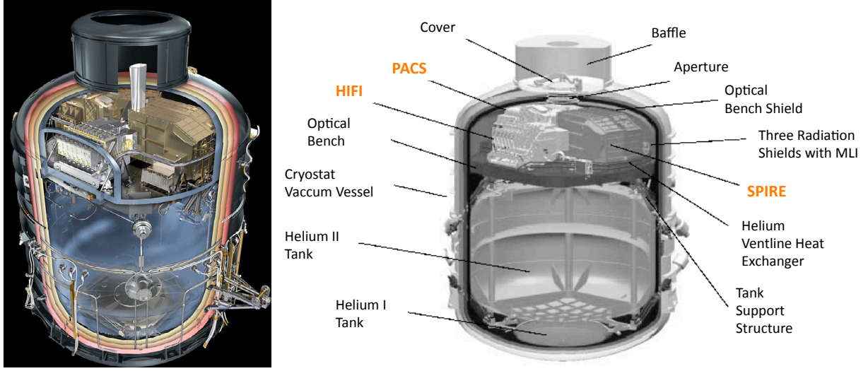
Fig. 3.2. (left) The payload module (from Pilbratt et al. (2010) ). (right) Schematic view of the payload module where all of the components have been labelled. The three instruments are highlighted in orange (adapted from the Herschel Observers' Manual).
