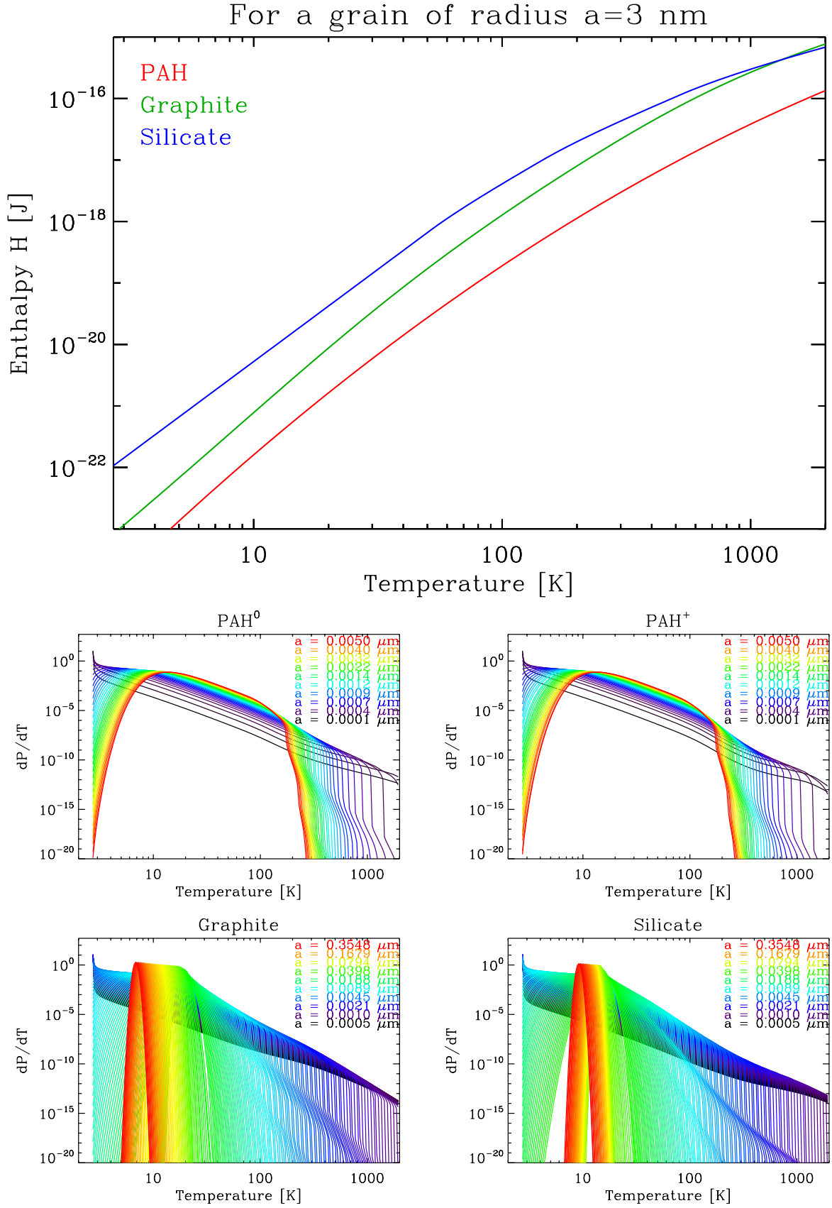
Fig. 7.4. (top): Enthalpies for the considered dust species. (bottom row) Temperature probability distributions for the different grain species. The colour codes the grain size: from black (small radius) to red (big radius).
