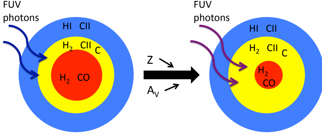
Fig. 2.5. Illustration of the impact of metallicity and extinction on the structure of the molecular clouds, inspired from Wolfire et al. (2010). The harder FUV photons penetrate deeper into the cloud at low metallicity, increasing the relative size of the region where H_2 is co-existing with CII and CI (yellow zone), compared to the region where both H_2 and CO are present (red zone). The blue zone corresponds to the atomic phase, where no H_2 is present.
