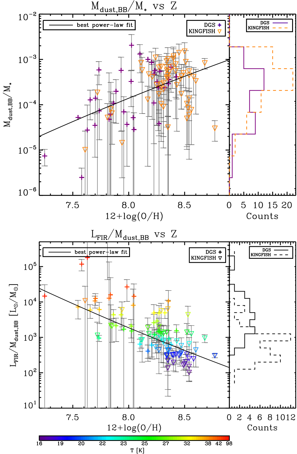
Fig. 5.7. (top) M_{\text{dust,BB}}/M_* as a function of metallicity for DGS (purple crosses) and KINGFISH (orange downward triangles). The best power-law fit is indicated as a black line, and corresponds to: \log(M_{\text{dust,BB}}/M_*) = (-20.4 \pm 1.6) + (18.4 \pm 1.8) \times \log(12+\log(\text{O}/\text{H})) . The distribution of M_{\text{dust,BB}}/M_* is indicated on the side for both samples: plain purple line for DGS and dashed orange line for KINGFISH. (bottom) L_{\text{FIR}}/M_{\text{dust,BB}} as a function of metallicity for DGS (crosses) and KINGFISH (downward triangles). The colours code the temperature, T . The best power-law fit line is indicated as a black line, and corresponds to: \log(L_{\text{FIR}}/M_{\text{dust,BB}}) = (24.4 \pm 1.1) + (-23.6 \pm 1.2) \times \log(12+\log(\text{O}/\text{H})) . The distribution of L_{\text{FIR}}/M_{\text{dust,BB}} is indicated on the side for both samples: solid line for DGS and dashed line for KINGFISH. On both plots: the errors on the metallicities are omitted for clarity. They are of about 0.1 dex on average.
