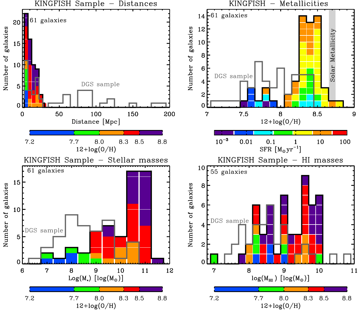
Fig. 3.14. Properties of the KINGFISH sample: Distributions of distances, D , ( top left ), metallicities, in terms of 12+\log(\text{O}/\text{H}) , ( top right ), stellar masses, M_* ( bottom left ) and HI masses ( bottom right ). The colour scale represents the range of star-formation rate for the top right panel and metallicity for the others. Colour scales are identical as for Fig. 3.11 and 3.12. Galaxies for which the parameter is not available or is an upper limit are not shown here. The number of KINGFISH galaxies on the plot is indicated on the top left of each panel. The DGS distributions for each parameter are indicated in grey.
