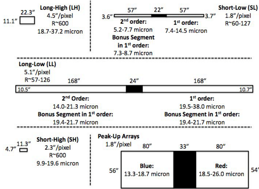
Fig. 6.4. Schematic view of the IRS slits. Note that the slits are not parallel in the Spitzer plane as shown here. Actual slit position angles relative to a Spitzer roll angle of 0° are SL = +84.7°, LL = +181.2°, SH = +221.5°, LH = +136.7°, and IRS Peak-up = +177.0°.
