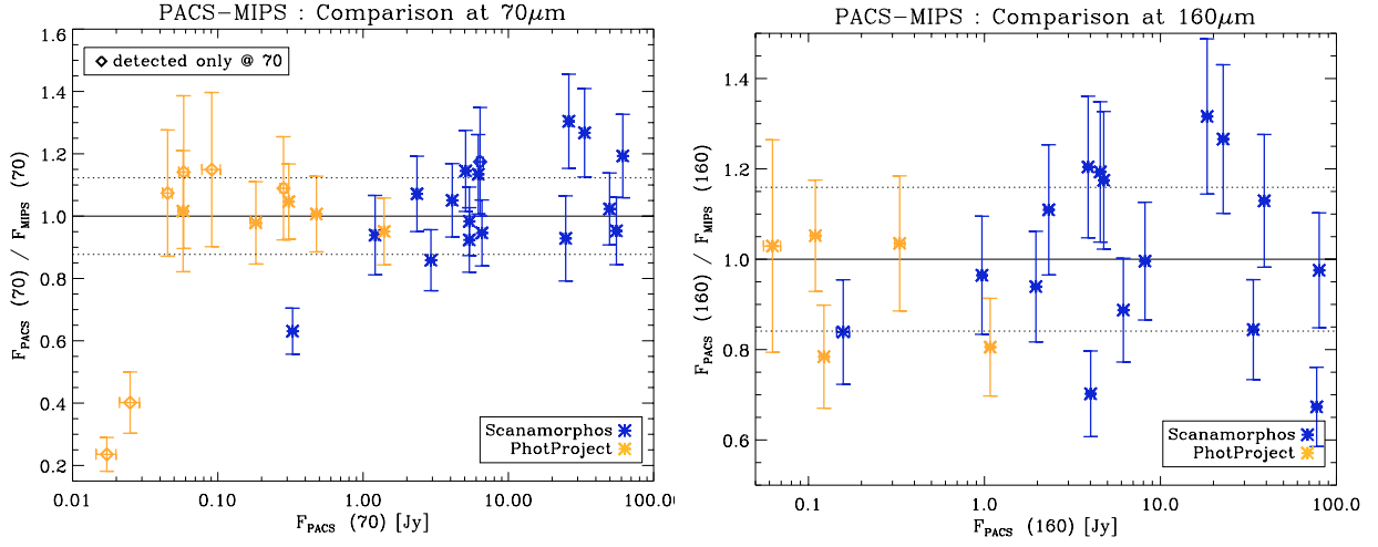
Fig. 6.8. Comparison of PACS flux densities and MIPS flux densities: PACS-to-MIPS flux density ratios as a function of PACS flux density at 70 \mu\text{m} ( left ) and 160 \mu\text{m} ( right ). As a guide to the eye, the unity line is added as a solid line as well as the average uncertainties on the ratio in both bands as dotted lines. These average uncertainties are \sim 12\% and \sim 16\% at 70 and 160 \mu\text{m} . Colours distinguish the selected mapping method (see Chapter 4).
