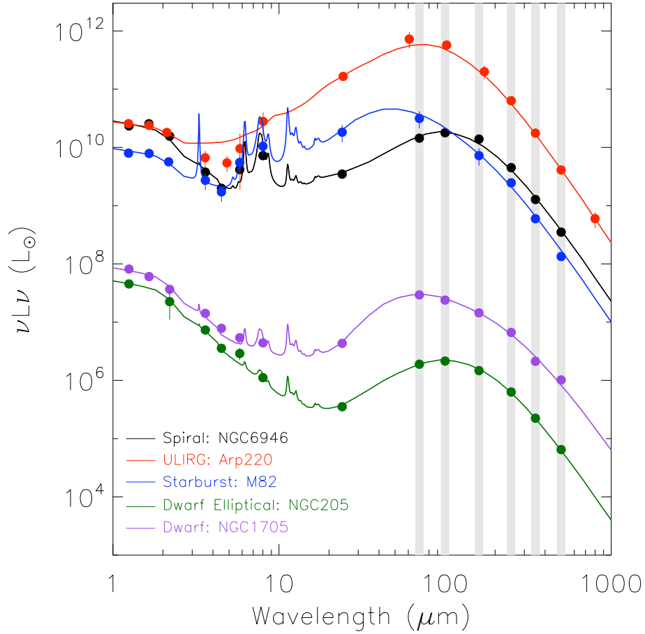
Fig. 1.16. SEDs for various galaxy types (from Madden et al. 2013 ): Spiral (NGC6946, in black), Dwarf (NGC1705, in purple), Dwarf Elliptical (NGC205, in green), Starburst (M82, in blue) and ULIRG (Arp220, in red). The differences in their SED shapes are due to the variations in the relative contribution of each ISM phase to the total emission of the galaxy. The grey stripes indicate the wavelength coverage of the 6 Herschel bands (see Chapter 3).
