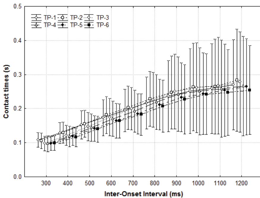
Figure II.15: Contact times are presented as a function of the tempo (inter onset interval – IOI) imposed by an external metronome
