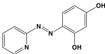
Figure 6 : 4-(2-pyridylazo)resorcinol.
