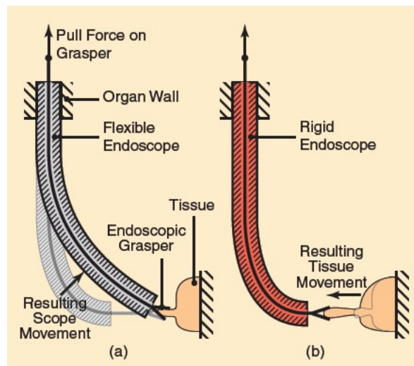
Fig. 2.22. Force limitation problem when using flexible systems (reprinted from [109]).
