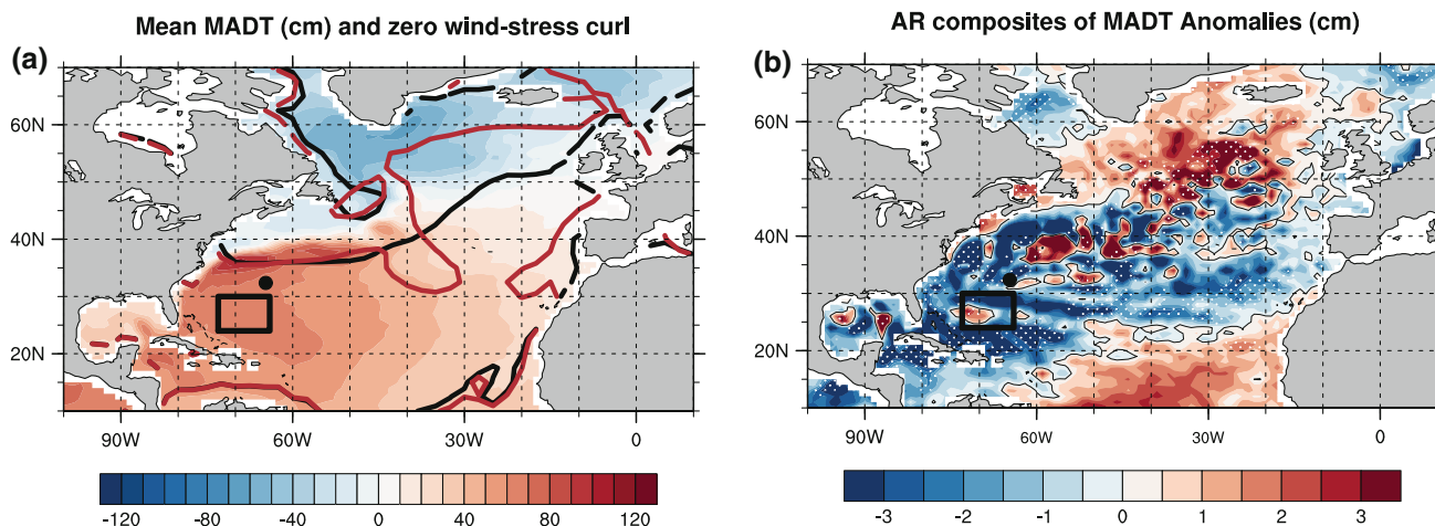
Fig. 4 (Left) Mean map of absolute dynamic topography (colors). Climatological (black contours) and AR composite (red contours) zero wind-stress curl. (Right) Map of absolute dynamic topography
