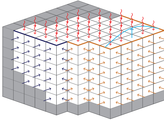
Figure 5.3: Schematic describing the functioning of PAGO. Each cube represents a temperature grid point. Gray points represent land cells. Red arrows represent surface heat fluxes, centered on the cells. Sections (resp. transport across the sections) are represented by blue/orange lines (resp. blue/orange arrows). A cyan blue line symbolises the ocean free surface.
