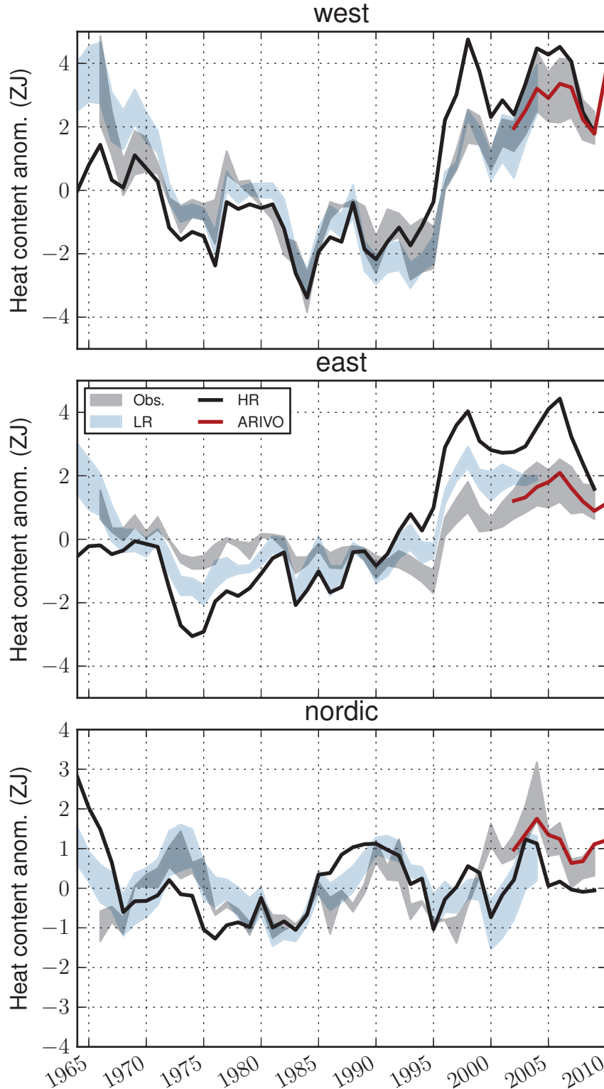
Figure 5.5: Observed and modelled heat content anomalies over the first 0 – 700m of the water column. The gray shading represents the envelope between heat content anomalies of the EN3 and of the WOA09 datasets. The blue shading represents the envelope between the heat content anomalies of the LR experiments, while the black line represents the HR heat content anomalies. In all these time-series, the anomalies are computed by removing the 1966-2004 mean. The brown line represents the ARIVO heat content anomalies computed by removing the 2002-2009 average and by adding the 2002-2009 average of WOA09/EN3. ZJ=10^{21} J
