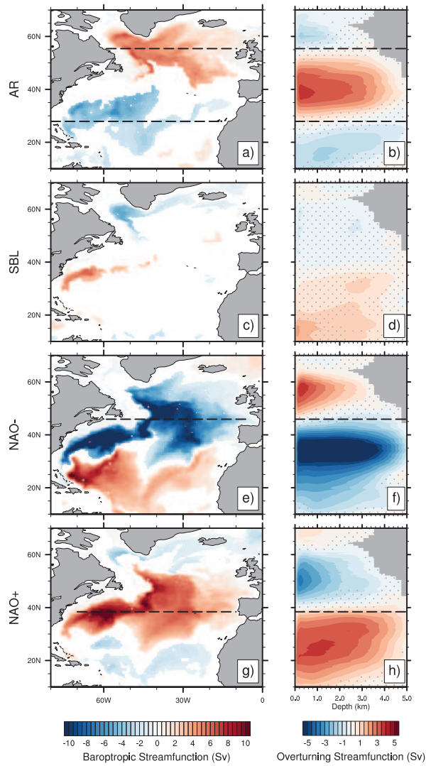
FIG. 4. Monthly composites of barotropic (a, c, e, g) and overturning (b, d, f, h) streamfunction anomalies issued from REF (see text for details). Non-significant values ( t -test at the 95% level of confidence) are omitted in the left panels and stippled in the right panels. Dashed black lines represent meridional Ekman transport anomalies convergence/divergence, determined from zonally averaged zonal winds.
