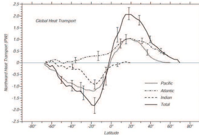
Figure 1.3: Ocean heat transport decomposed into the contributions of the Pacific, Atlantic and Indian Oceans. Source: Houghton et al. 1996 with data of Trenberth and Solomon, 1994
