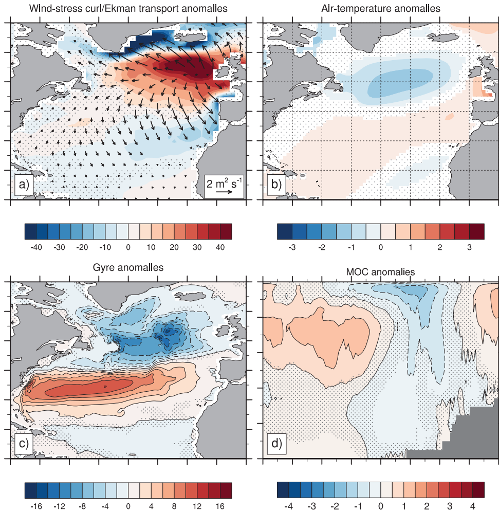
Figure 4.5: (a) Wind-stress curl and Ekman transport anomalies. (b) Air-temperature anomalies (c and d) gyre and overturning anomalies averaged over the last 10 years of the AL-only experiment.
