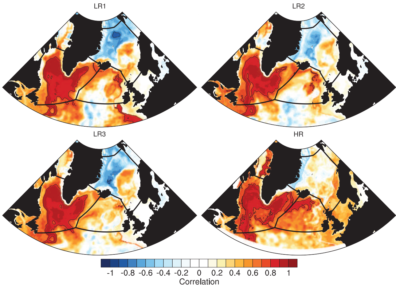
Figure 5.24: Correlation map between heat content anomalies at each grid point and heat content anomalies in the western subpolar gyre (figure 5.13, left panel). Black contour lines represent the -0.8/ +0.8 contours.
