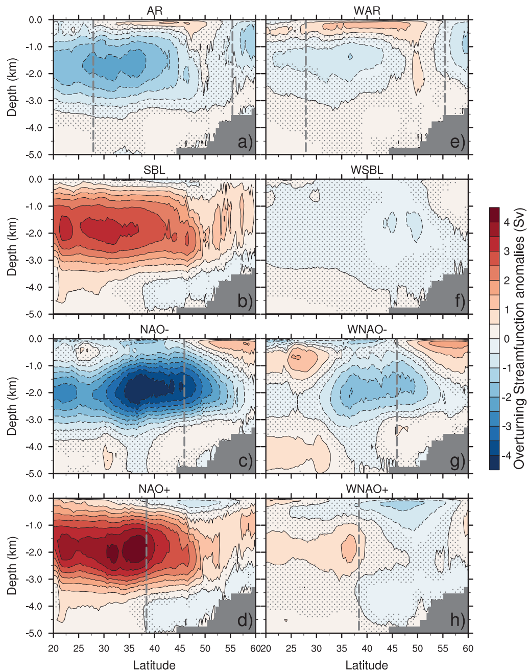
FIG. 9. Same as figure 7 but for the overturning streamfunction. Dashed gray lines represent meridional Ekman transport anomalies convergence/divergence, determined from zonally averaged zonal winds.
