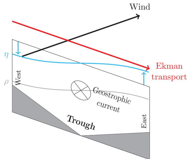
Figure 5.9: Ekman driven response of the water mass exchange between the Atlantic and the Nordic Seas to BLK wind anomalies. The black arrow represents the wind anomalies associated with BLK and the red arrow the corresponding Ekman transport. The blue line represents the sea-surface height and the gray line an isopycnal. The geostrophic current is directed northward ( \otimes symbol).
