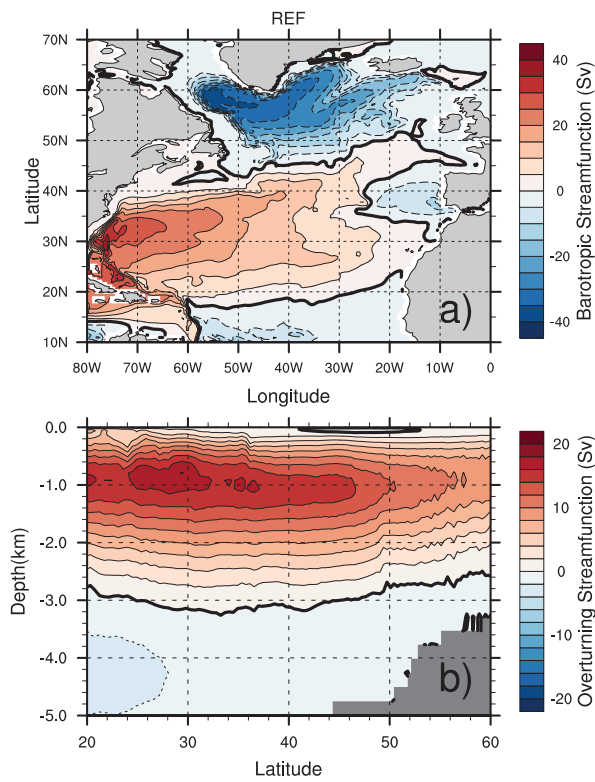
FIG. 3. Mean circulation in the REF experiment averaged over 45 years. a) Barotropic streamfunction (contour interval: 5 Sv). b) Meridional Overturning Streamfunction (contour interval: 2 Sv).
