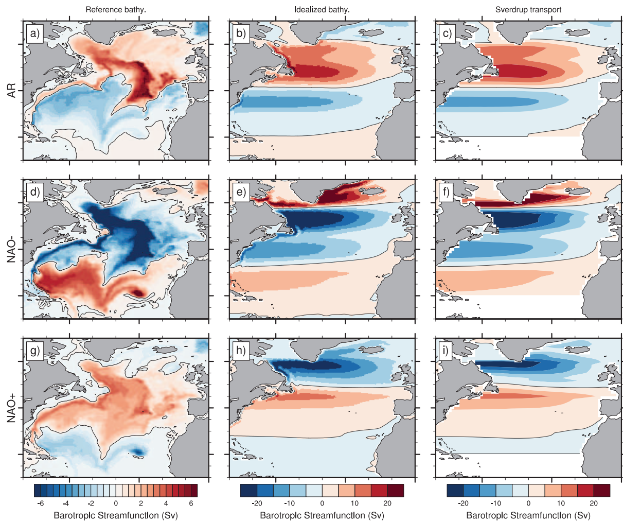
FIG. 5. Barotropic streamfunction averaged over the 4 th year of the idealized barotropic experiments (a, b, d, e, g, h). Left panel: reference bathymetry. Middle panel: idealized bathymetry (3000 m everywhere). Right panel: classical Sverdrup theory.
