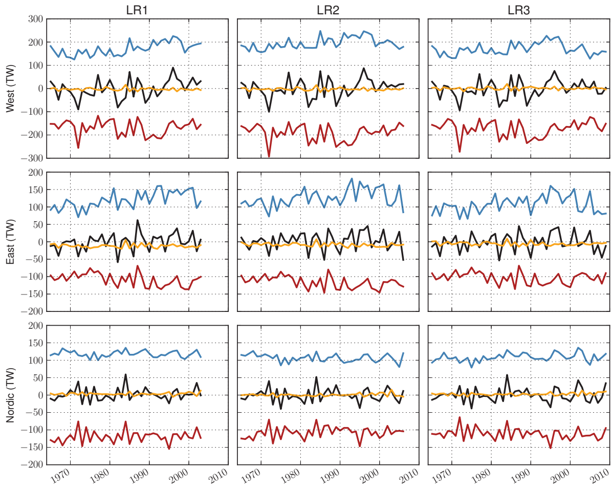
Figure 5.4: Variations in heat content within a year (black line) and yearly averaged OC (blue), SF (brown) and residual (orange).
