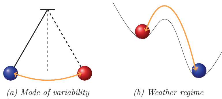
Figure 2.11: Schematic of the two visions of the NAO described in this chapter. Positive NAO is represented by a red marble, negative NAO is represented by a blue marble. Orange arrows represent changes from one phase to another.
