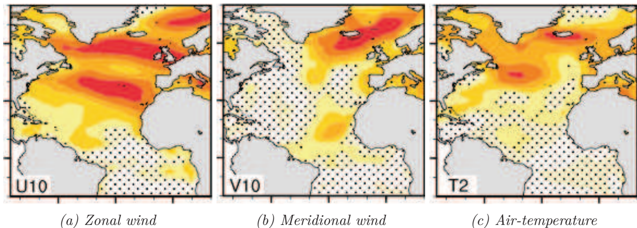
Figure 2.9: Interannual linear correlations between winter averaged observed forcings and reconstructed forcings via multiple linear regression with the weather regimes winter occurrences.
