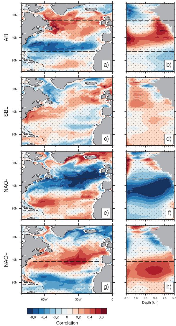
FIG. 6. 0-lag correlations between yearly averaged barotropic (a, c, e, g) and overturning (b, d, f, h) streamfunction anomalies issued from REF and the winter WRs occurrences. Non significant values ( t -test at 95%) are stippled. Dashed black lines represent meridional Ekman transport anomalies convergence/divergence, determined from zonally averaged zonal winds.
