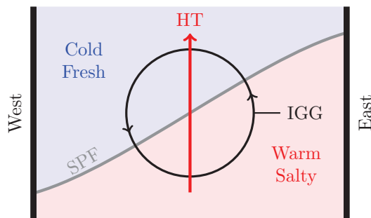
Figure 5.10: Schematic of a cyclonic intergyre gyre (IGG) associated driven by \text{NAO}^- (black circle). The gray line represents the subpolar front (SPF). The thick red line represents the overall heat transport (HT).
