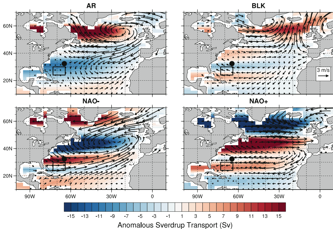
Fig. 3 Daily composites of winter wind-field anomalies (arrows, reference = 3 \text{ m}\cdot\text{s}^{-1} ) and corresponding anomalous Sverdrup transport (colors, contour interval = 1 Sv). The black point shows the
