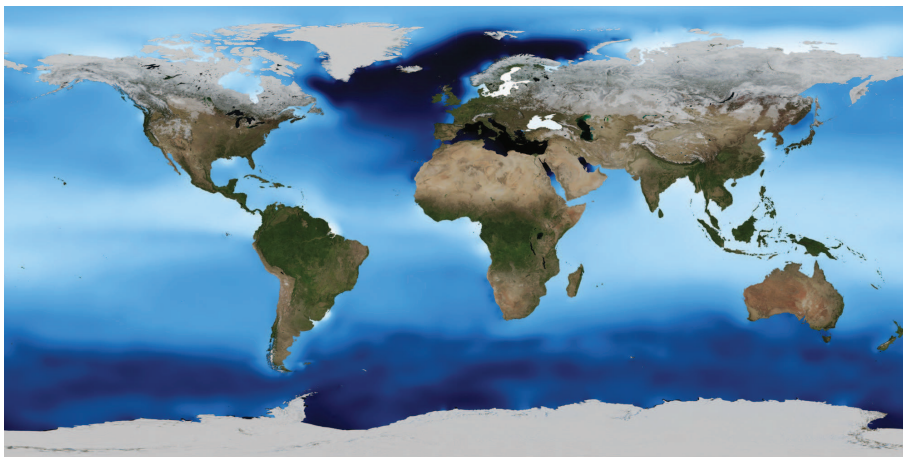
Figure 1.4: Sea-surface density ( \text{kg m}^{-3} ). Deep blue characterises density greater than 1017 \text{ kg m}^{-3} . Source: NASA/Goddard Space Flight Center Scientific Visualisation Studio, with data from the World Ocean Atlas 2005 (Locarnini et al., 2006).
