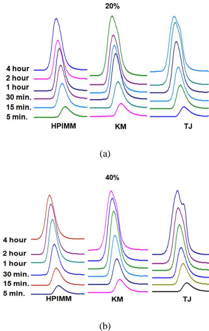
Figure 4.SI 1. GPC traces for 20% (a) and 40% (b) BzMA composition at different residence times and for the three micromixers employed.
