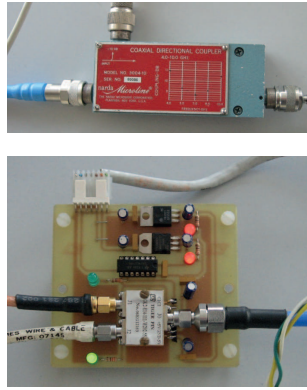
Directional coupler and SPDT switch for Tx-Rx synchronization
