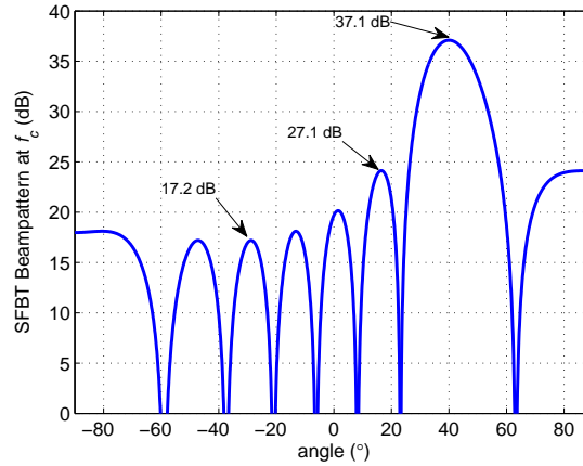
FIGURE 3.11: The SFBT beampattern in dB at f_c .
