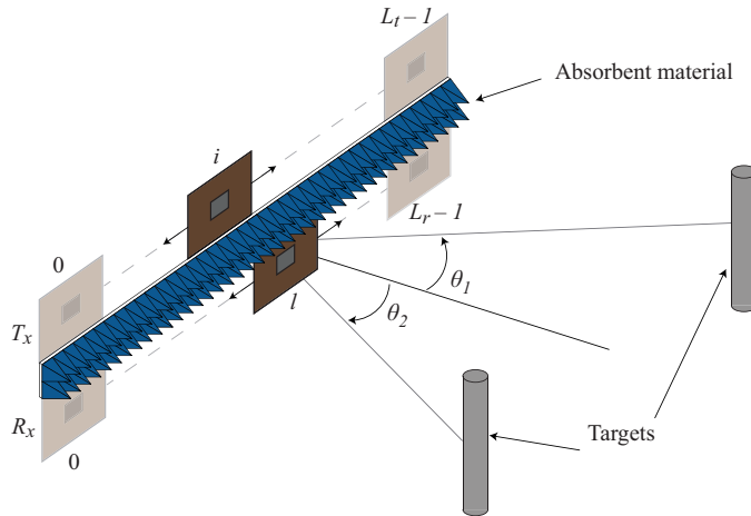
FIGURE 5.1: Scheme of the antenna configuration of the measurement platform.
