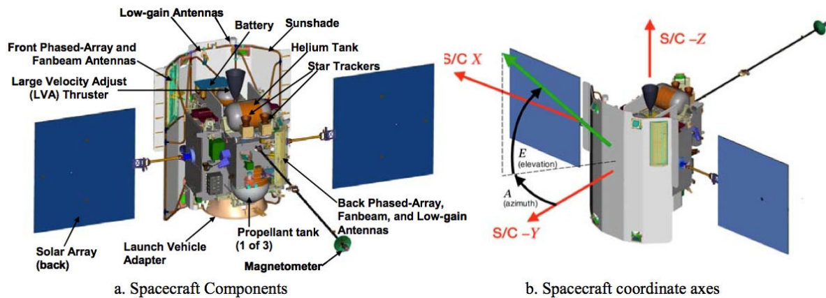
Figure 5.2: MESSENGER spacecraft geometry (Vaughan et al., 2006).
