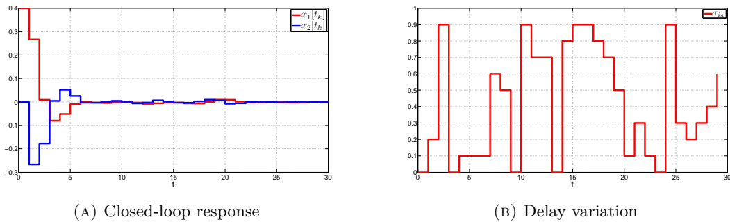
FIGURE 5.4: Stable closed-loop response
