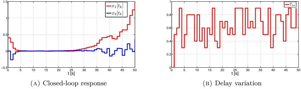
FIGURE 5.9: Closed-loop response when \|\omega\|_\infty \leq 0.004
