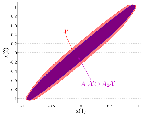
FIGURE 4.7: D-contractive set for the dDDE (4.33).
