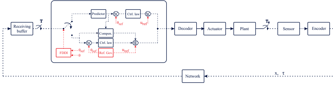
FIGURE 5.14: Model-based controller with delay detection and compensation
