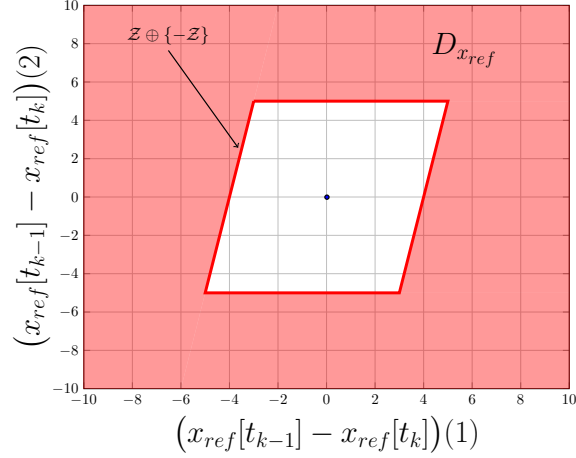
FIGURE 5.15: Reference admissible set
