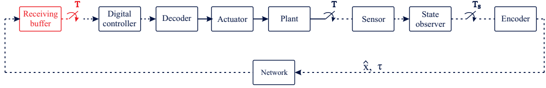
FIGURE 5.6: Single-channel networked control system
