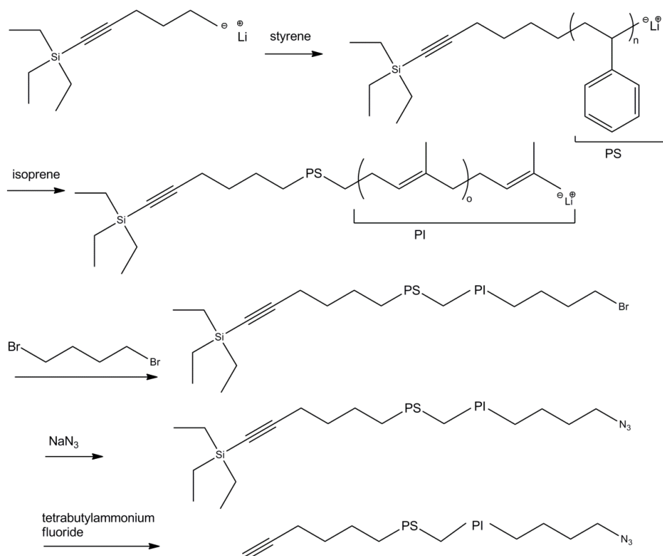
Scheme 39: Schematic representation of the synthesis of \alpha -acetylene- \omega -azido-PS- b -PI (taken from ref. 118 ).
