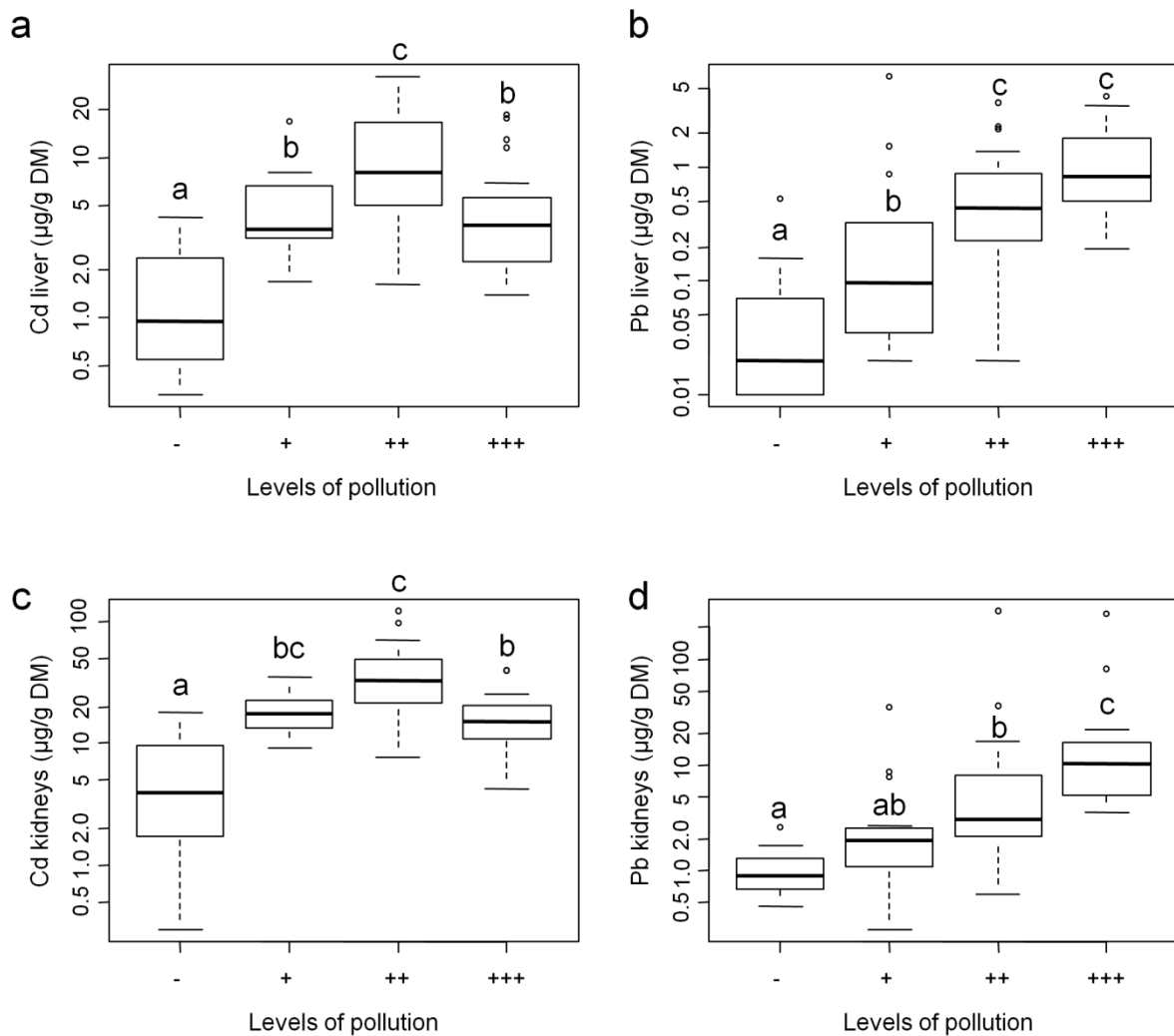
Figure III.2 \text{Log}_{10} -transformed concentrations ( \mu\text{g/g DM} ) of Cd in the liver (a), Pb in the liver (b), Cd in the kidneys (c) and Pb in the kidneys (d) as a function of the gradient of contamination. Different letters indicate significant differences among groups (Tukey's HSD, p < 0.05 ).
