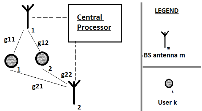
Fig. 1. An example illustration of a 2 \times 2 virtual MIMO with g_{i,j} representing the channel between BS antenna i and user j .
