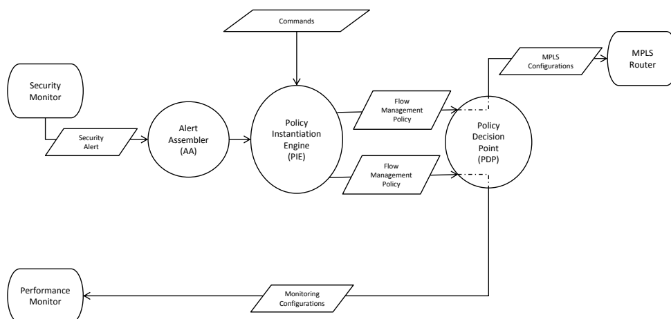
FIGURE 4.3: Workflow of the flow admission policy
