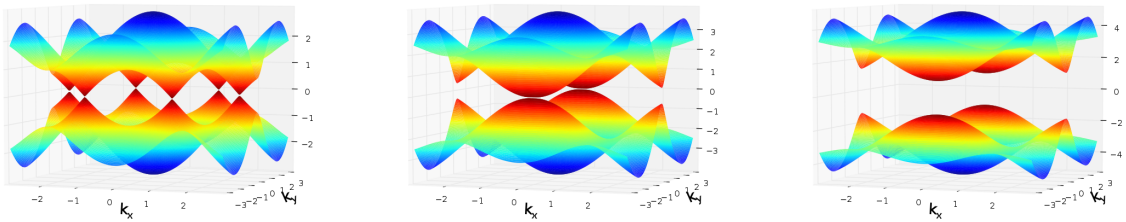
Fig. 1.6 Dispersion relation for t' = t , t' = 2t and t' = 3t (from left to right).
