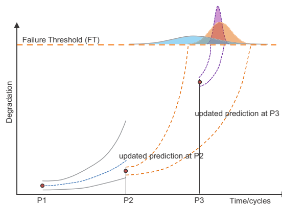
FIGURE 1.4: Uncertainty bands associated with RUL estimations (adapted from [191])
