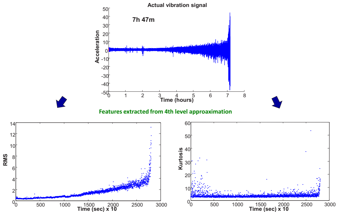
FIGURE 2.6: Classical features extracted from a degraded bearing
