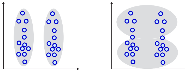
FIGURE 4.7: Example of clustering with D_{SE} (left) and ED (right) metrics [3]
