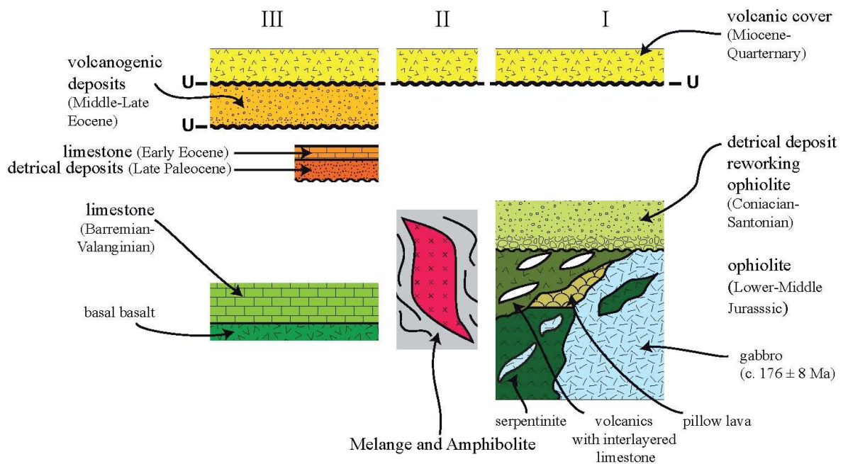
Figure 18 - Synthetic lithostratigraphic log of the three main units of the Amasia ophiolite window. I, the upper unite corresponding to ophiolite. II, the metamorphic unit comprising of the tectonic melange and the lens of garnet bearing amphibolites. III, the lower unit.
