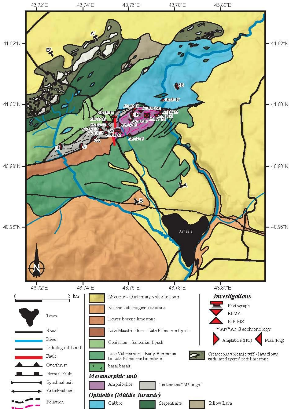
Figure 32 - Structural map of the Amasia ophiolite window. Location is indicated on Figure 30. Plot of geological sections of Figure 33B along with the locations of photographs of Figure 34 as well as of samples investigated through ICP-MS, EPMA, and 40 Ar/ 39 Ar geochronology methods of Figures 36, 37 & 39, respectively.
