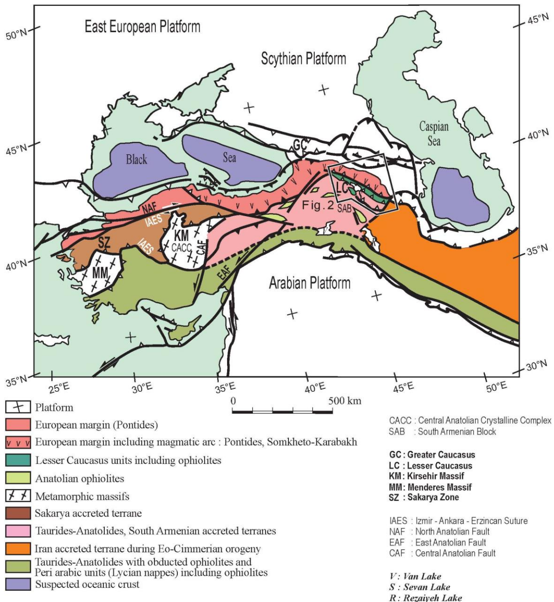
Figure 14 - Tectonic map of the Middle East–Caucasus area, with main blocks and suture zones, after Avagyan et al. (2005), modified. Location of figure 2 indicated.
