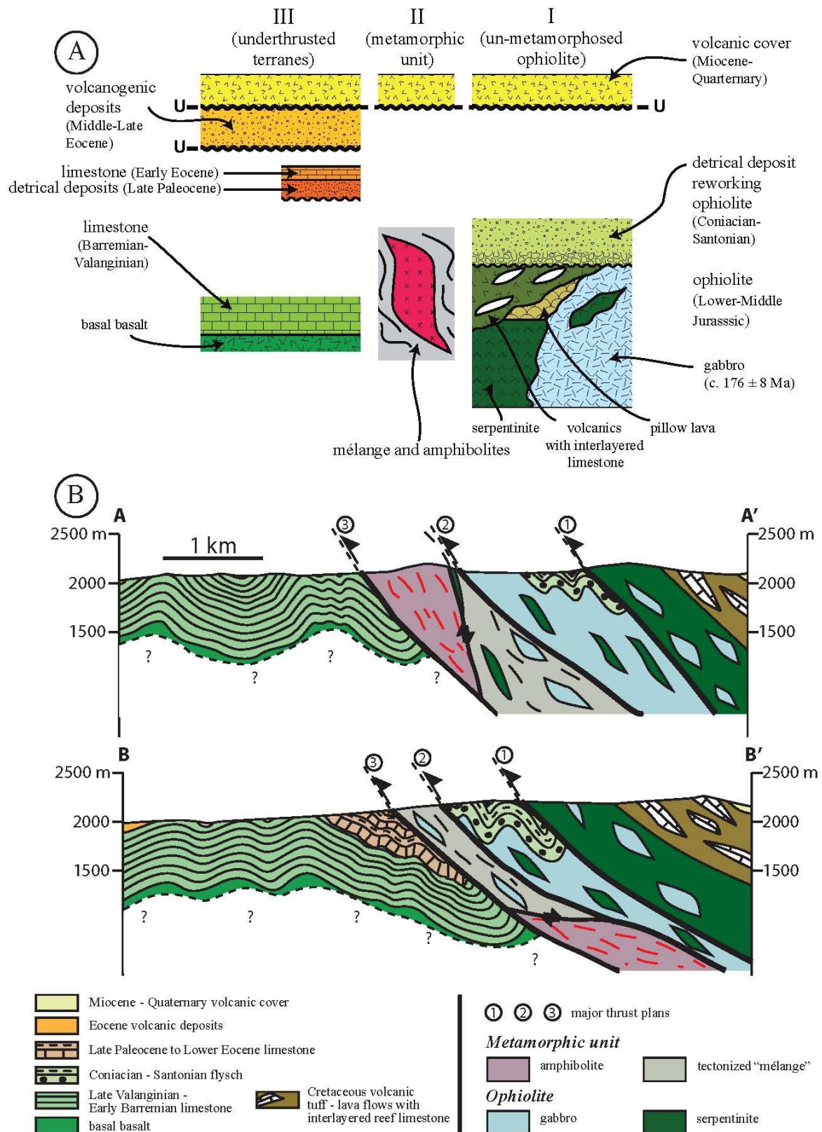
Figure 33 - (A), synthetic litho-stratigraphic record of the three main units of the Amasia ophiolite window; I) upper unit corresponding to the un-metamorphosed ophiolite, II) metamorphic unit comprising of the tectonic mélange and the lens of garnet bearing amphibolites, III) the lower (Southern) unit. (B), sketch geological cross sections of Amasia ophiolite. Locations are indicated on Fig. 32.
