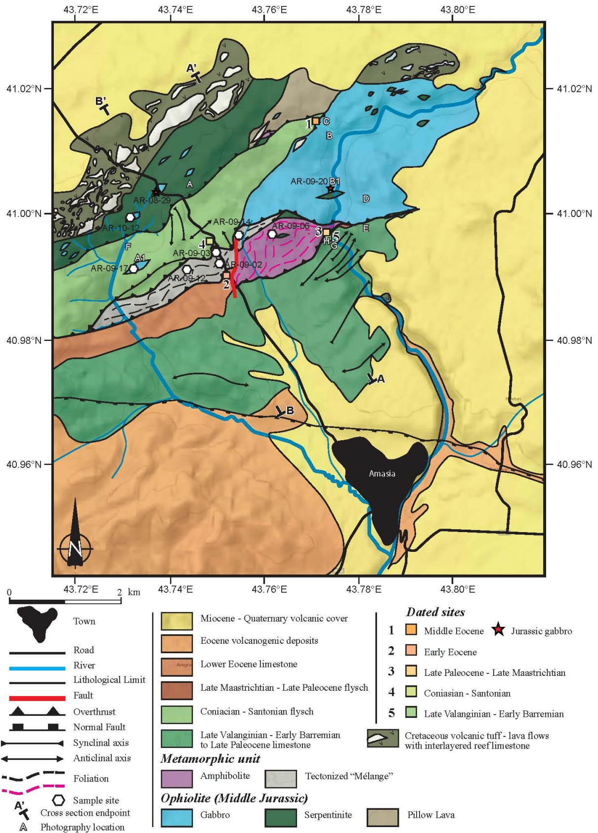
Figure 17 - Structural map of the Amasia ophiolite window. Location is indicated on figure 16. Plot of geological sections of figure 18 along with dated samples by the Ar-Ar method and paleontological identification are shown.
