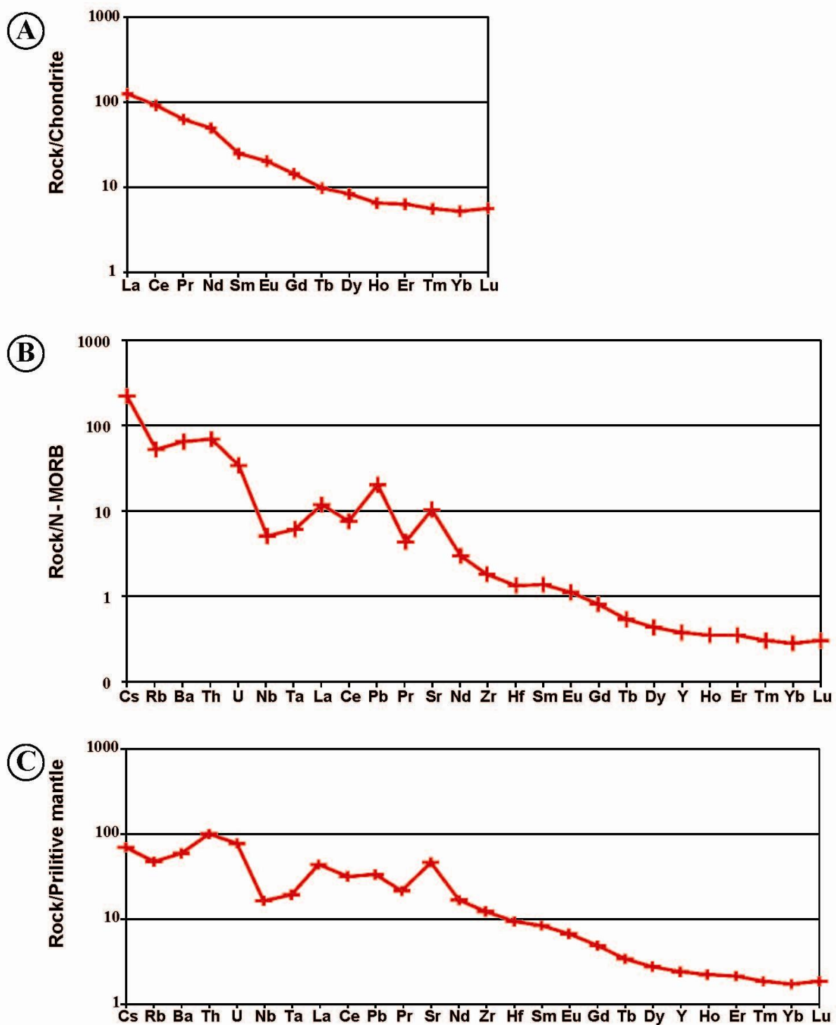
Figure 57 - Chondrite normalized REE and N-MORB and primitive mantle normalized multi-element spider diagrams of the granodiorite sample ARL-10-33. Normalizing values are from Sun and McDonough (1989).
