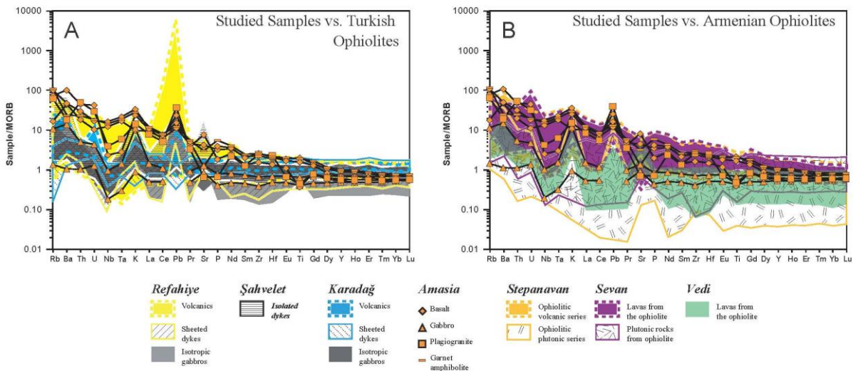
Figure 27 - N-MORB normalized multi-element spider diagrams. Data concerning Erzincan-Erzurum region (Refahiye, Şahvelet and Karadağ) from Parlak et al. (2012) and concerning Stepanavan, Sevan and Vedi from Galoyan et al. (2007; 2009) and Rolland et al. (2009b; 2010). Normalizing values are from Sun and McDonough (1989).
