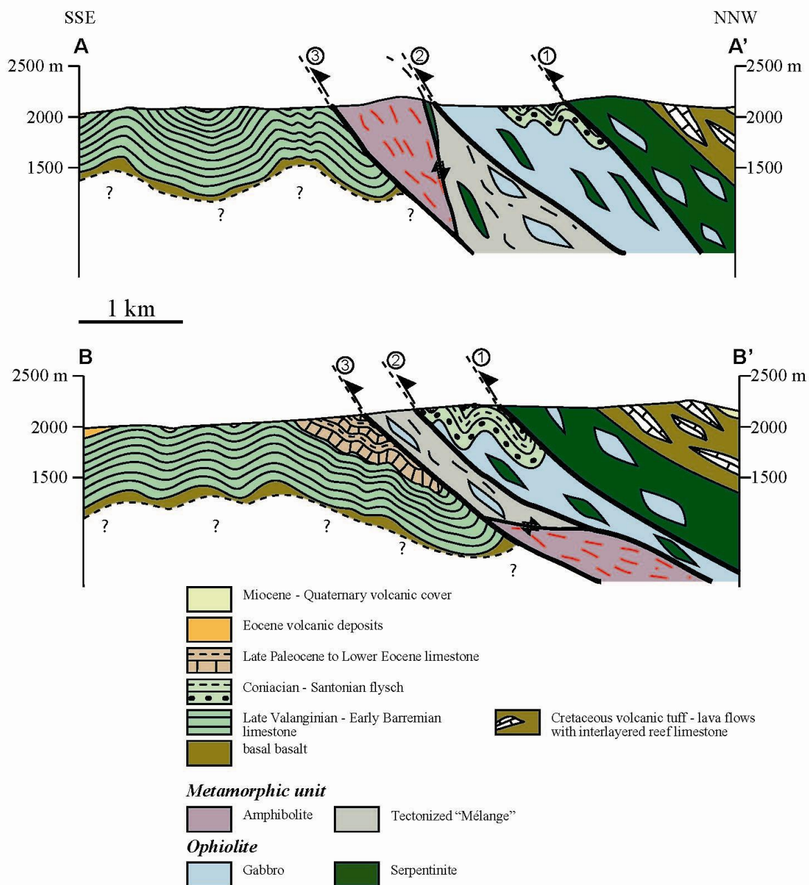
Figure 19 - Sketch geological cross sections of Amasia ophiolite. Locations are indicated on figure 17.
