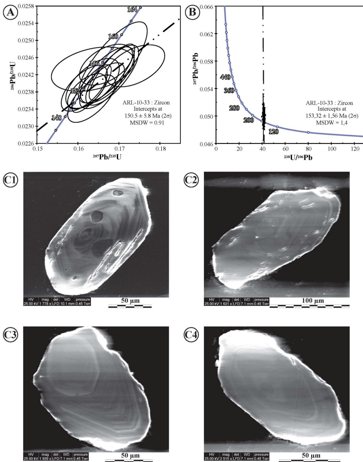
Figure 56 - U-Pb laser ICP-MS ablation concordia, A, and Tera-Wasserburg age diagrams, B, for the samples ARL10-33. C1, C2, C3 and C4 scanning electron microscope photography of dated granodiorite zircons corresponding to numbered analyses of table 15, respectively. Location of the sample is shown on Figure 52.
