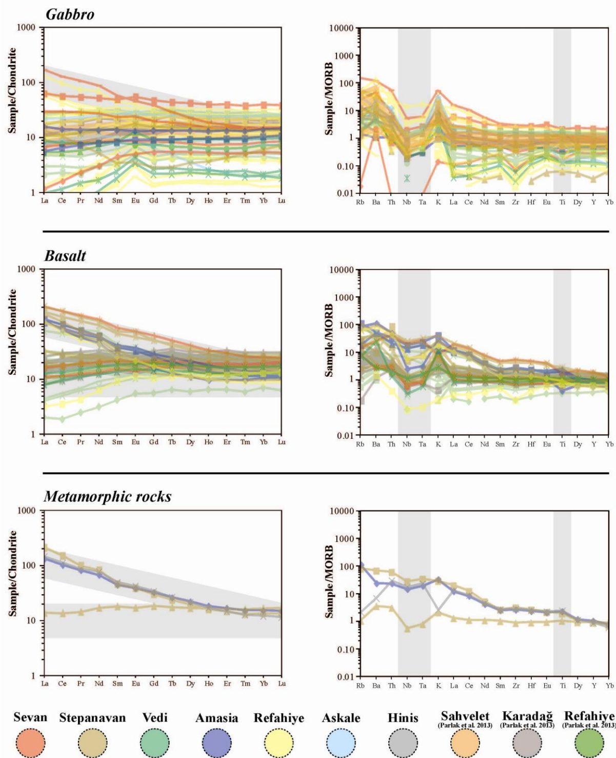
Figure 47 - Chondrite normalized REE spider diagrams and N-MORB normalized multi-element spider diagrams. Data concerning Erzincan–Erzurum region (Refahiye, Şahvelet and Karadağ) from Parlak et al. (2013) and concerning Stepanavan, Sevan and Vedi from Galoyan et al. (2007, 2009) and Rolland et al. (2009b, 2010). Normalizing values are from Sun and McDonough (1989).
