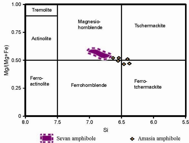
Figure 23 - Chemical composition of amphibole from the AR-08-21 and AR-08-22 gabbro samples, after Leake et al. (1997). Data concerning Sevan amphiboles from Galoyan et al. (2009).
