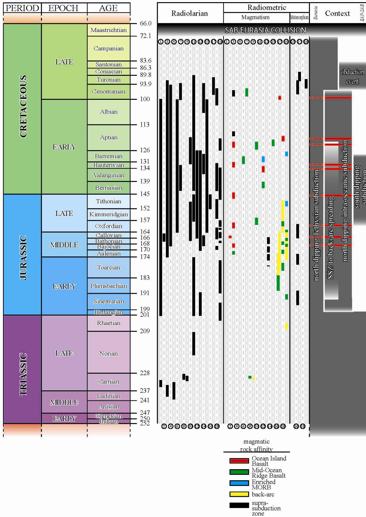
Figure 65 - Compilation of chronological data including extension of the radiolarian fauna, magmatic series of the ophiolite bodies outcropping emplaced prior to the obduction event and metamorphic lithologies marking the limit between the ophiolites and the Eurasian margin as well as between the ophiolites and the underthrust EAP-SAB
