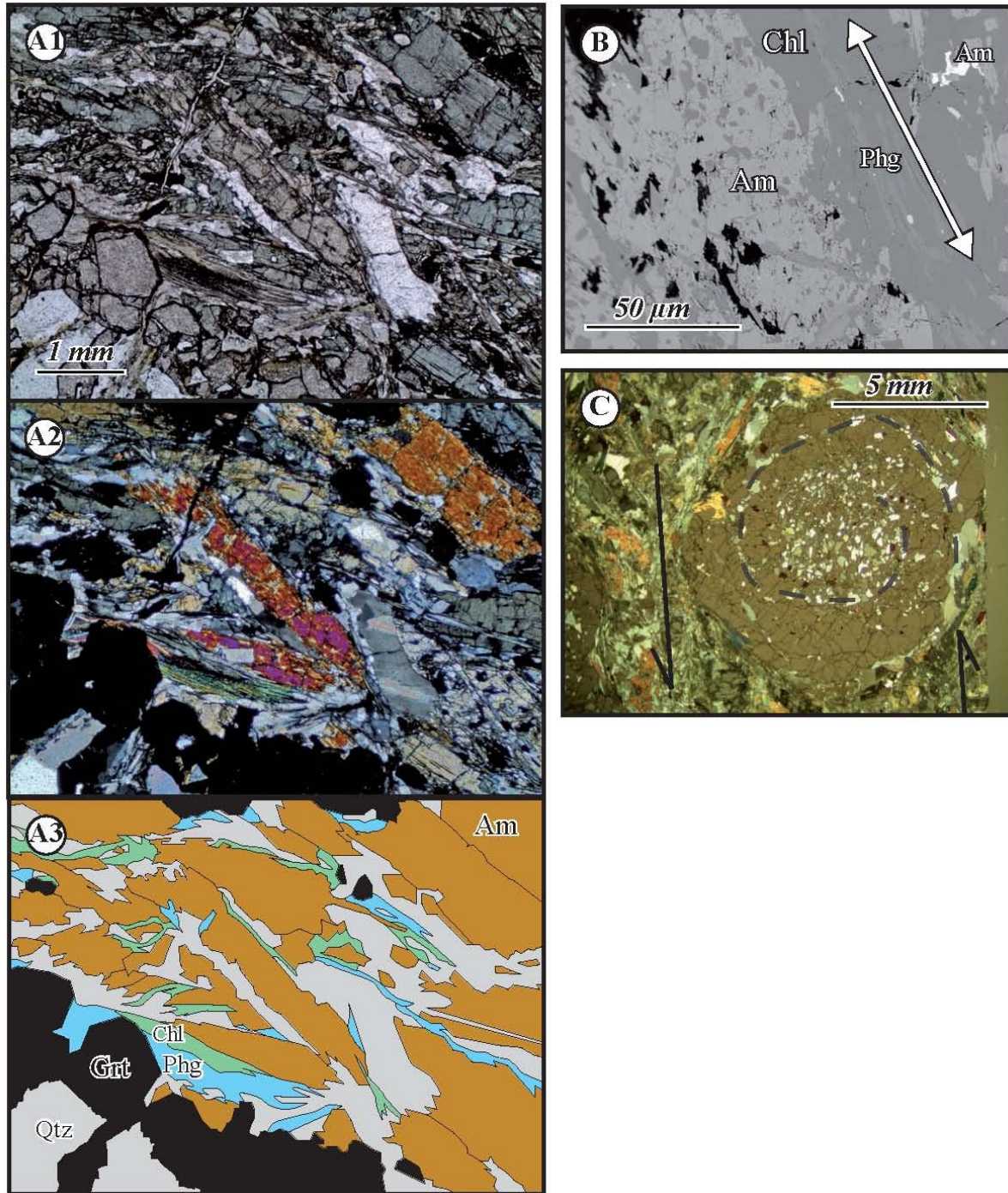
Figure 35 - (A1) and (A2), photographs of a thin section of garnet amphibolite sample AR-08-09c in plain and cross-polarized light, respectively. (A3), sketch of thin section photographs. Cross cutting relationships of amphiboles with micas (Phg) and chlorites (Chl) indicate the existence of amphiboles (Phg) prior to micas. This is also supported by the garnets (Grt) and amphiboles, which are molded by micas and chlorites. (B), back-scatter image of garnet amphibolite sample AR-09-08. Lineation is exhibited with the alignment of amphiboles (Am), white micas (Phg) and chlorites (Chl). (C), microscope photography of garnet amphibolite sample AR-09-09. The garnet is rolled in response to syn-kinematic growth during shearing.
