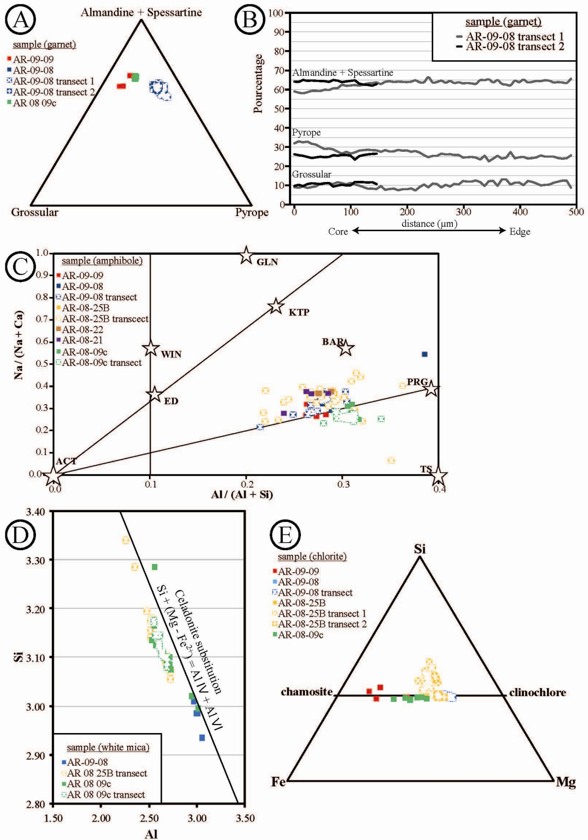
Figure 37 - Diagrams of analyzed of Amasia garnet amphibolite minerals. (A), triangular plots showing chemical compositions of Amasia amphibolite garnets. (B), compositional profiles of two garnets of the Amasia amphibolites.
