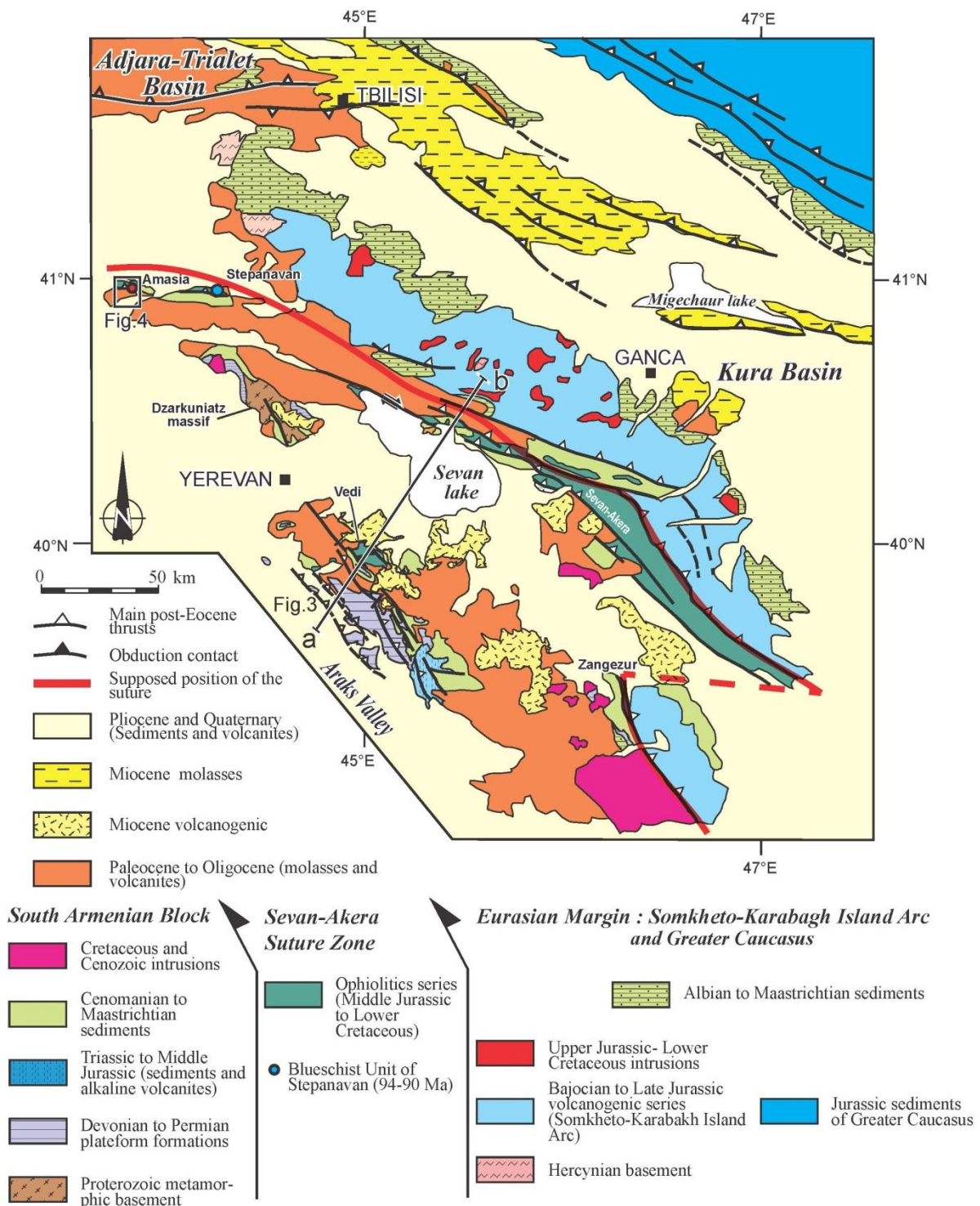
Figure 15 - Structural map of the Lesser Caucasus modified from Sosson et al. (2010). Location is indicated on figure 14. Plot of geological section figure 16 and location of figure 17 indicated.
