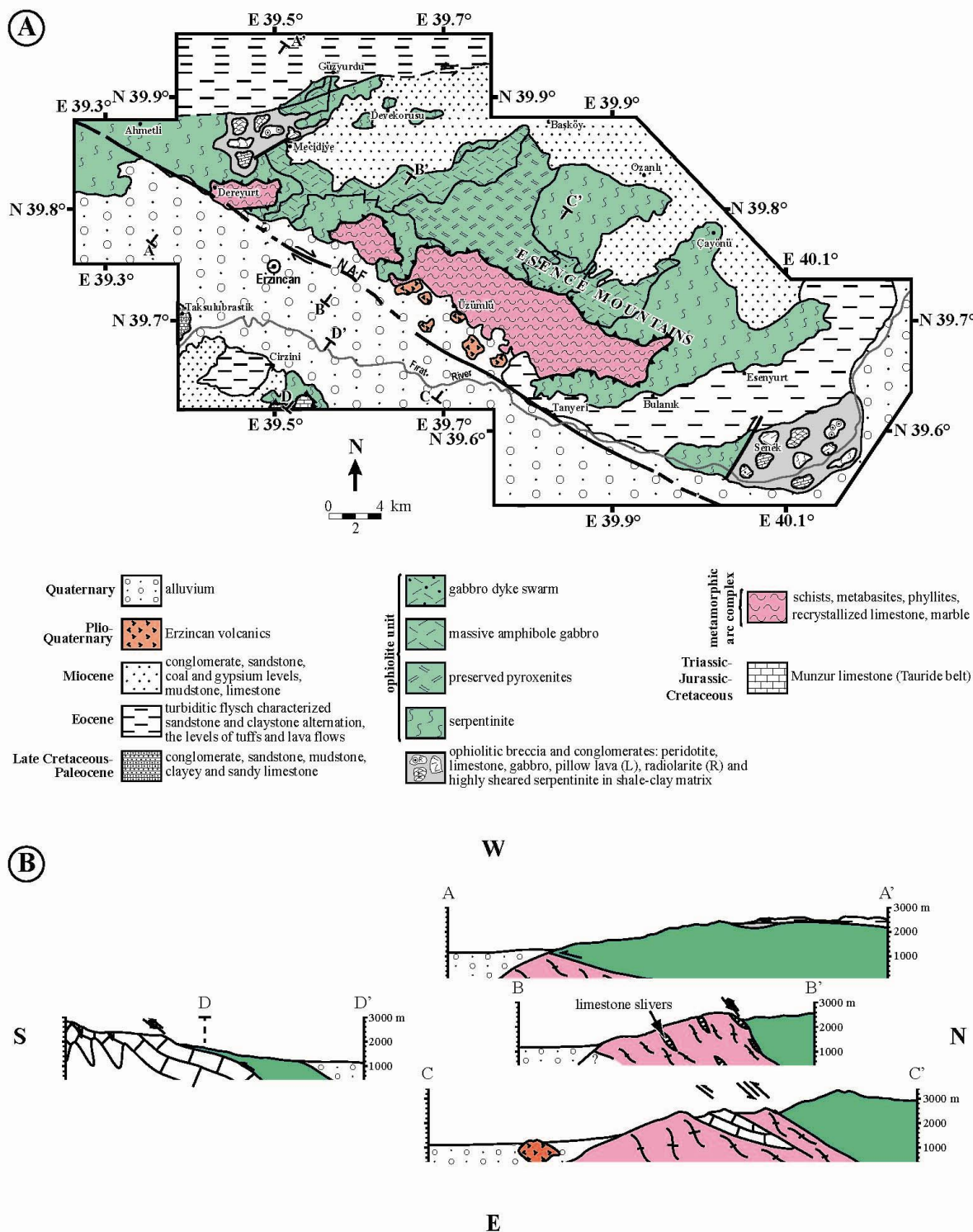
Figure 44 - Geological map and cross-sections of the Refahiye ophiolite in the vicinity of Erzincan. A: Geological map featuring the position of the cross-sections (modified after Aktimur et al., 1995; Özen et al., 2006; Sarıfakıoğlu et al., 2009). B: Geological cross-section illustrating the positioning and structural relationships between the main units based on field observations.
