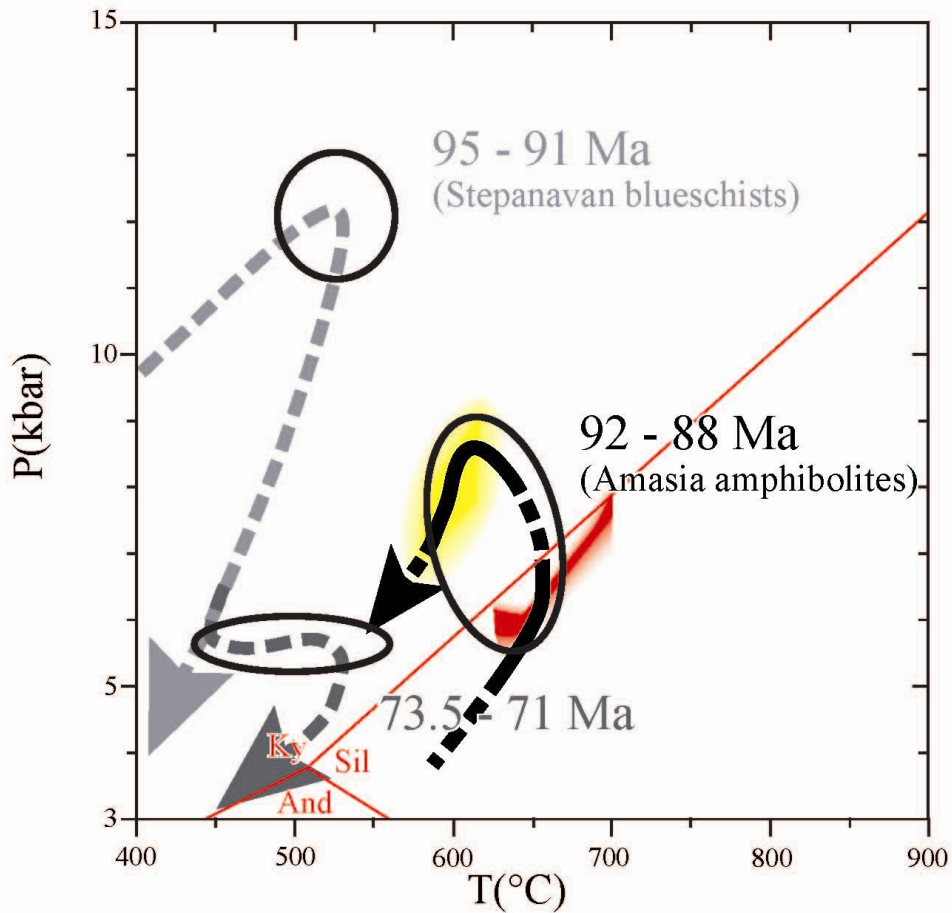
Figure 40 - Compilation of determined PT-t paths for the Amasia-Sevan-Akera metamorphic rocks found in basal position of ophiolite bodies inferred through this study of the outcrops of Amasia garnet amphibolite in black and Stepanavan blueschist (Rolland et al. , 2009a) in grey.
