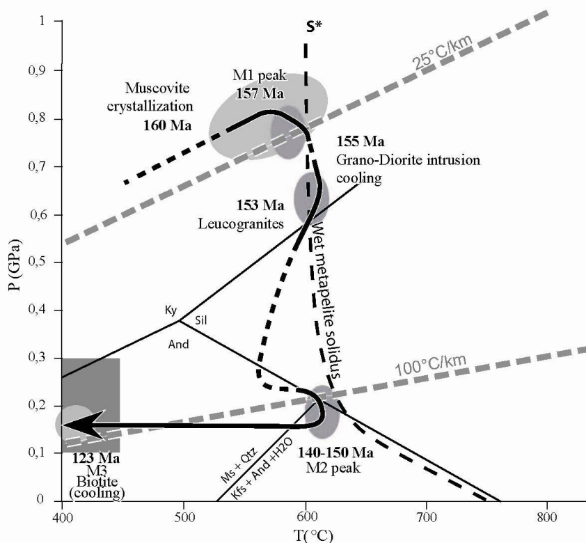
Figure 60 - PT-t path including metamorphic (Figure 55C), ^{40}\text{Ar}/^{39}\text{Ar} and U-Pb age data.
