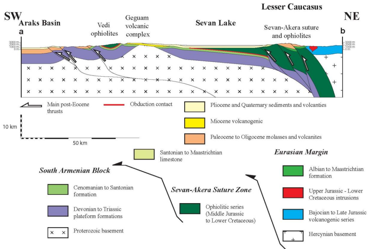
Figure 16 - Interpretative crustal-scale sketch cross-section of the Armenian-Azerbaijan transect. Location is indicated on Figure 15.
