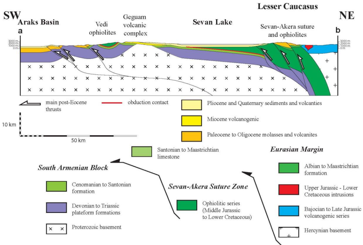
Figure 31 - Interpretative crustal-scale sketch cross-section of the Armenia-Azerbaijan transect. Location is indicated on Figure 30.
