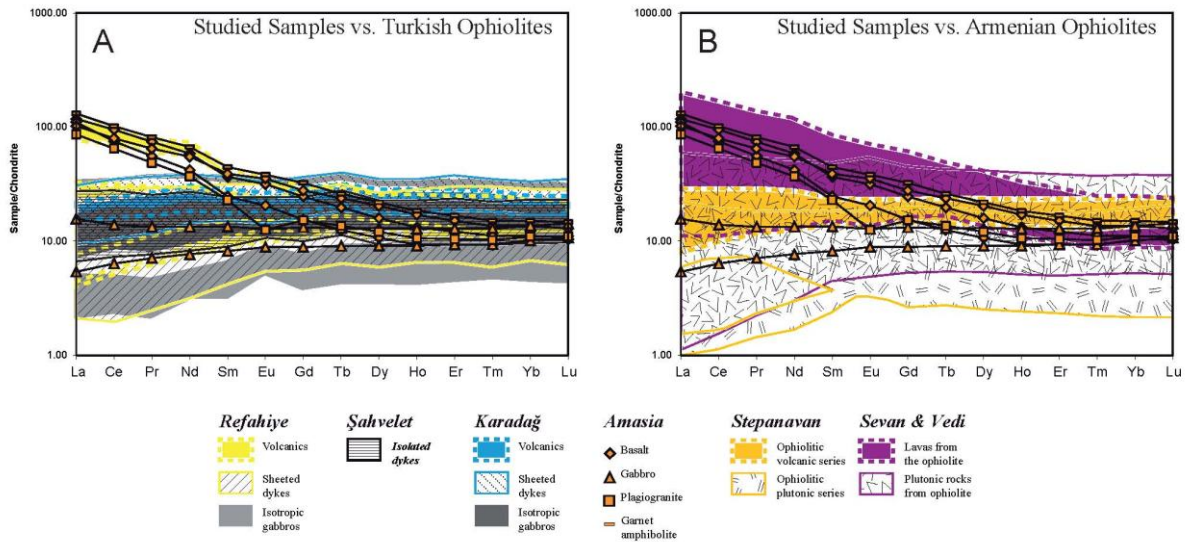
Figure 26 - Chondrite normalized REE spider diagrams. Data concerning Erzincan-Erzurum region (Refahiye, Şahvelet and Karadağ) from Parlak et al. (2012) and concerning Stepanavan, Sevan and Vedi from Galoyan et al. (2007; 2009) and Rolland et al. (2009b; 2010). Normalizing values are from Sun and McDonough (1989).
