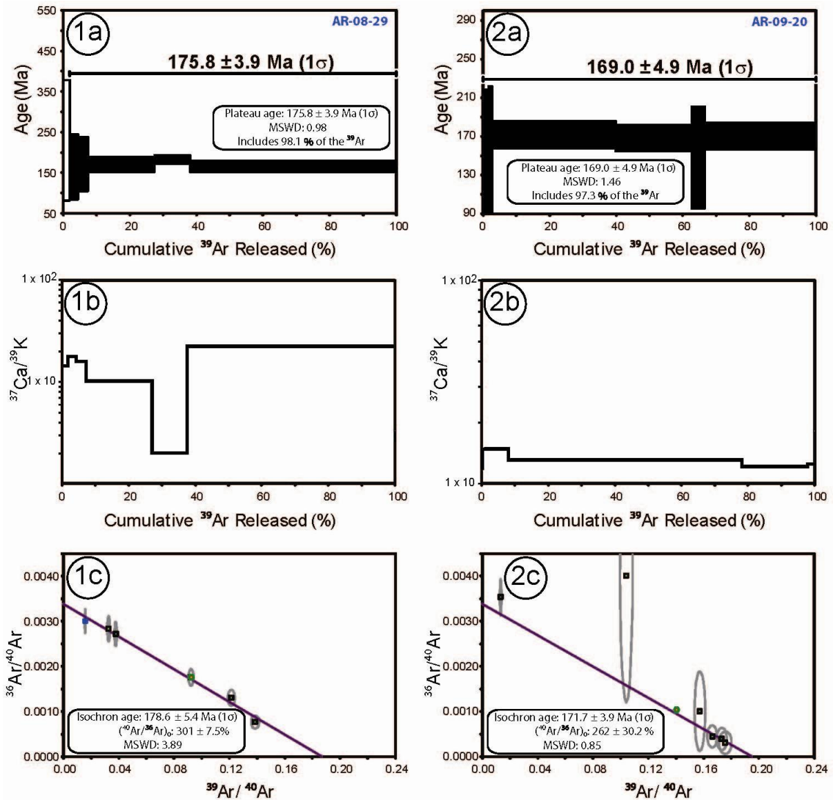
Figure 22 - ^{40}\text{Ar}/^{39}\text{Ar} age spectra Ca/K spectra and inverse isochrones of gabbro amphiboles. Locations of samples are shown on figure 17.
