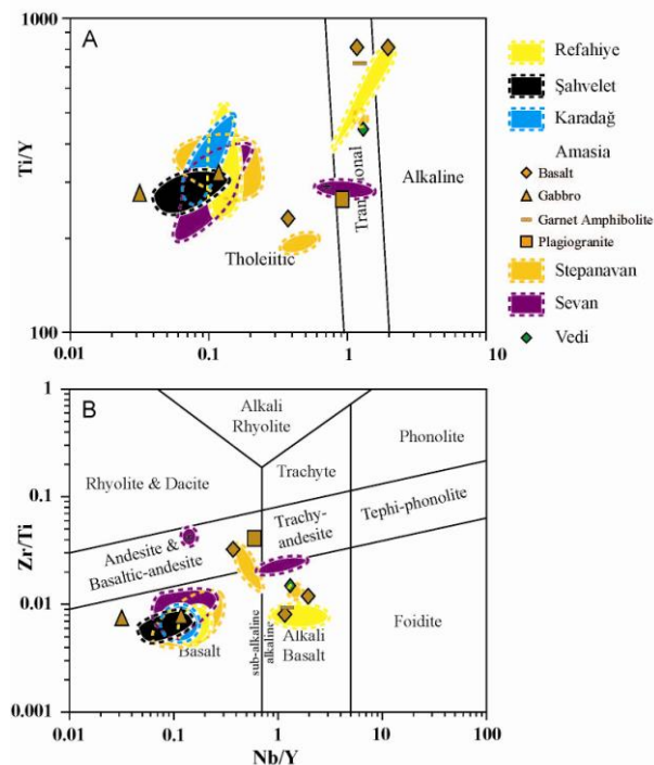
Figure 24 - Diagrams for crustal rocks of the ophiolites. Data concerning Erzinnca-Erzurum region (Refahiye, Şahvelet and Karadağ) from Parlak et al. (2012) and concerning Stepanavan, Sevan and Vedi from Galoyan et al. (2007; 2009) and Rolland et al. (2009b; 2010). A, Ti/Y versus Nb/Y (after Pearce 1982). B, Zr/Ti versus Nb/Y (after Pearce 1996).
