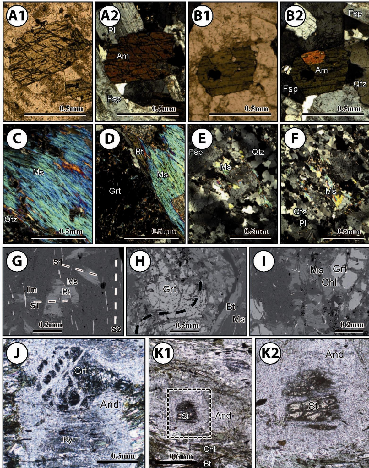
Figure 53 - Representative microphotographs of thin sections of rock samples of the Tsaghkuniats massif showing mineral relationships of ^{40}\text{Ar}/^{39}\text{Ar} dated mineral phases. A1 and A2, plane and cross-polarized images, respectively, centered on amphibole of granodiorite sample AR-03-64. B1 and B2, plane and cross-polarized images, respectively, centered on amphibole of granodiorite sample AR-03-64. C, cross-polarized images centered on white mica of micaschist sample AR-03-62M. D, cross-polarized image centered on white mica of micaschist sample AR-03-62M. The white mica molds the garnet and biotite. E, cross-polarized images centered on white mica of leucogranite sample AR-03-64. F, cross-polarized images centered on white mica of leucogranite sample AR-03-64. G, H and I, electron back-scatter (EBS) images of metaschist sample AR-03-64B. J, K1 and K2, optical microscope photography of sample AR-03-62M showing relics of garnet, kyanite and staurolite included in andalusite.
