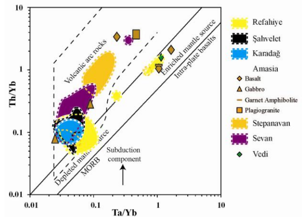
Figure 25 - Ta/Yb versus Th/Yb diagram (after Pearce 1982) for crustal rocks of the ophiolites. Data concerning Erzinnca-Erzurum region (Refahiye, Şahvelet and Karadağ) from Parlak et al. (2012) and concerning Stepanavan, Sevan and Vedi from Galoyan et al. (2007; 2009) and Rolland et al. (2009b; 2010).
