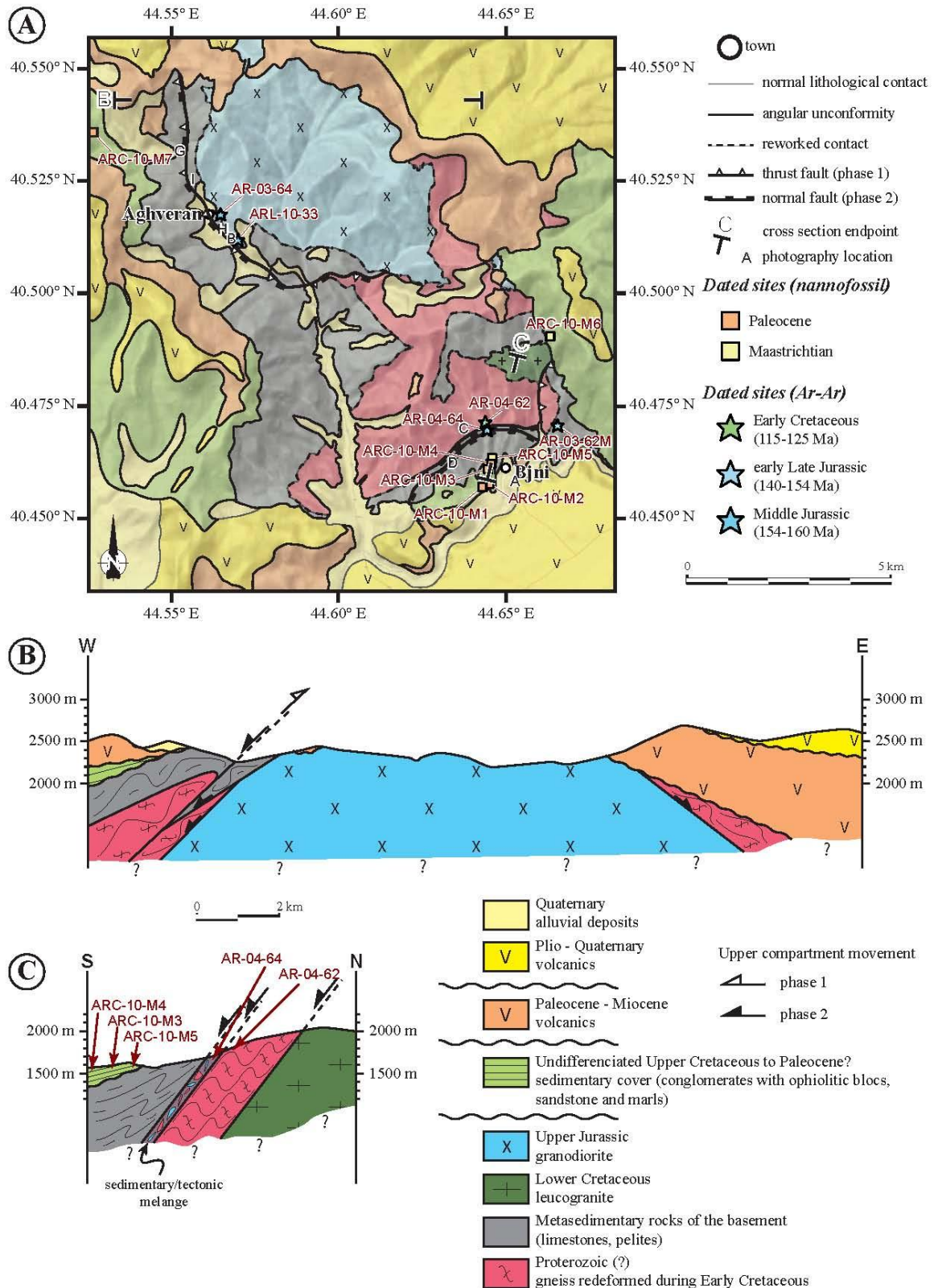
Figure 51 - A, structural map of the Tsaghkuniats massif, modified from Aghamalyan (1983). Location of this map is indicated on figure 1B. Plot of geological sections of Figure B and C along with localization of dated samples by the U-Pb and ^{40}\text{Ar}/^{39}\text{Ar} methods and paleontological identification. Location of field photographs of Figure 52 indicated as well. B and C, sketch geological cross sections of the Tsaghkuniats massif.
