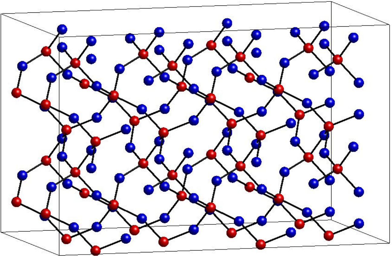
Fig.1.5: The quartz lattice (from http://volga.eng.yale.edu/sohrab/grouppage/pics/SiO2bulksupercell.jpg ). Si atoms/ions are in red, Oxygen atoms/ions in blue, iono-covalent bounds in black.
