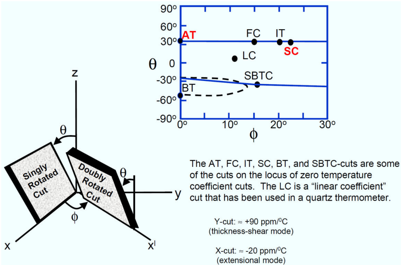
Fig.1.11: Zero temperature-coefficient quartz cuts [2].
