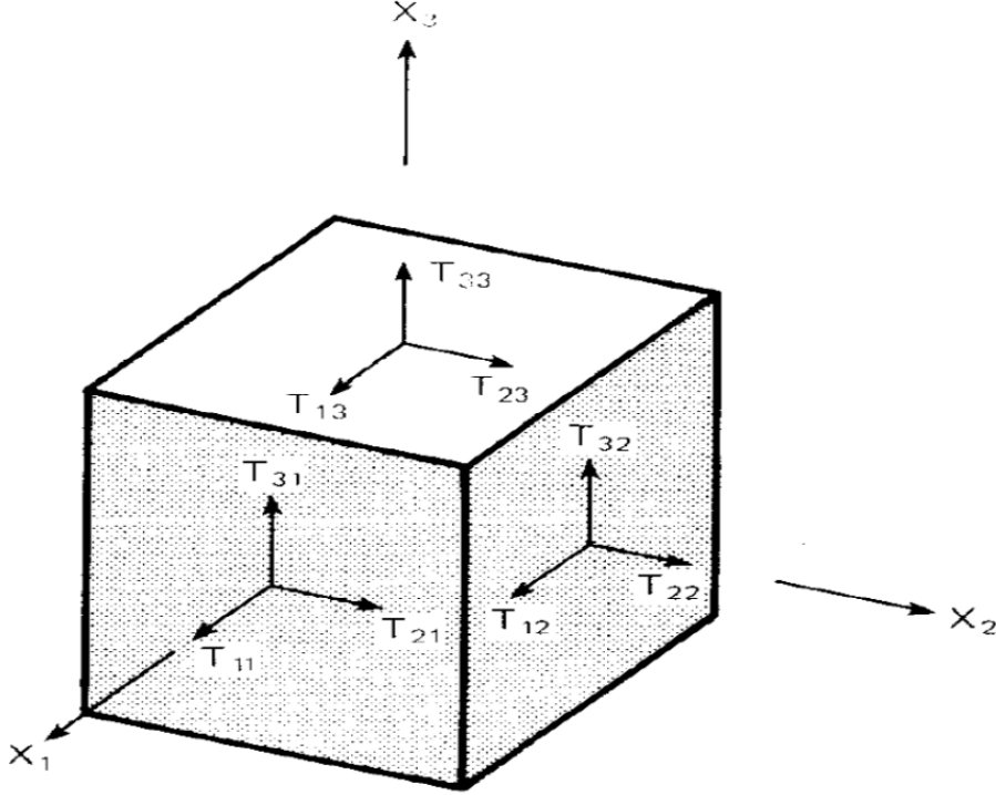
Fig. 1.3: The forces on the faces of a cube located inside a stressed body [4].
