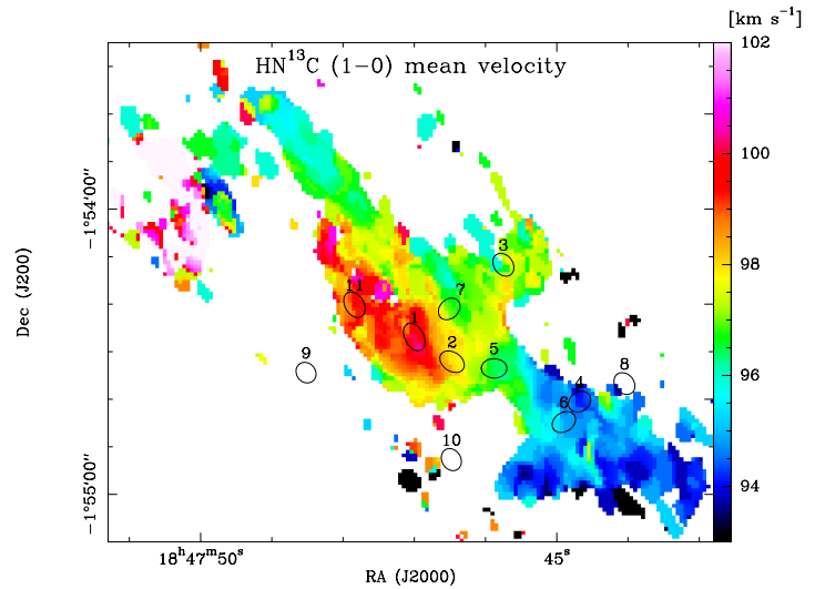
Fig. 6: Distribution of the velocity at rest throughout ridge, as traced by the Gaussian peak velocity of \text{HN}^{13}\text{C}(1-0) lines.
