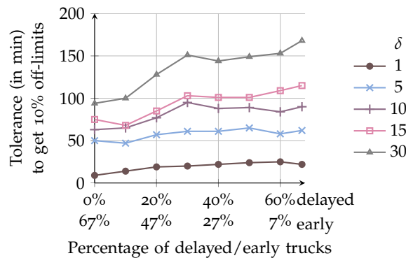
set3+3 – Aggregated I_2 to I_5 – 33% of the trucks are on time
