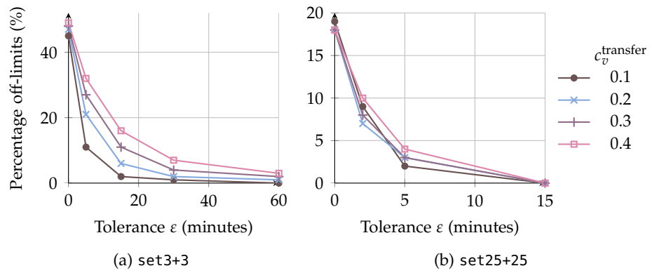
Figure 3.7: Transfer time variations: percentage off-limits for the average of I_2 to I_5
