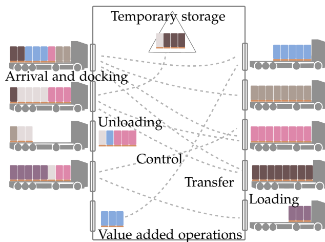
Figure 1.2: Cross-docking processes
