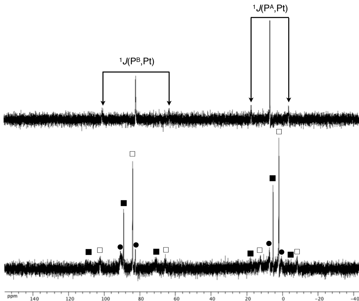
Figure 4. ^{31}\text{P}\{^1\text{H}\} NMR spectra of platinum complex 17 , recorded in \text{CDCl}_3 at 121.5 MHz +60^\circ\text{C} (top) and at -60^\circ\text{C} (bottom). The ABX patterns of the two sharp species are represented by filled and open squares whereas the two broad species are represented by dots.
