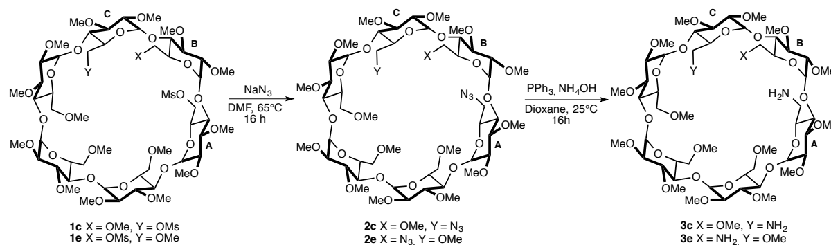
Scheme 1. Synthesis of diamines 3c,e .
