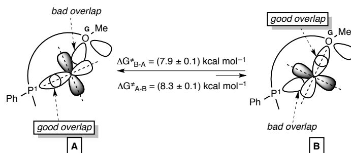
Scheme 27. Equilibrium between species A and B taking place in the dinuclear complex [\text{Pd}_2\text{Cl}_4(\mathbf{47})] .
