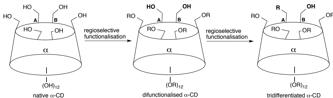
Scheme 1. Native, difunctionalised and tridifferentiated \alpha -CD.
