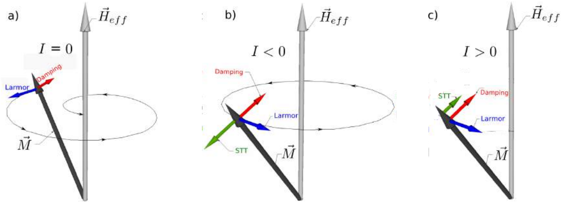
Figure 1.2.: Sketch of the magnetization motion in ferromagnetic object: the Larmor term or (adiabatic torque) induces the precession of the magnetization \vec{M} about the effective field whereas the damping term pushes magnetization in the direction of the effective field. Then, in absence of STT ( I=0 ) the magnetization is a spiral motion around the effective field. In the presence of STT ( I \neq 0 ), for I < 0 (b) the torque is opposite to the damping and therefore decreases its effect leads to a precession motion of the magnetization around the effective field, for I > 0 (c) STT is parallel to the damping and therefore increases it, then the magnetization aligns faster with \vec{H}_{eff} .
