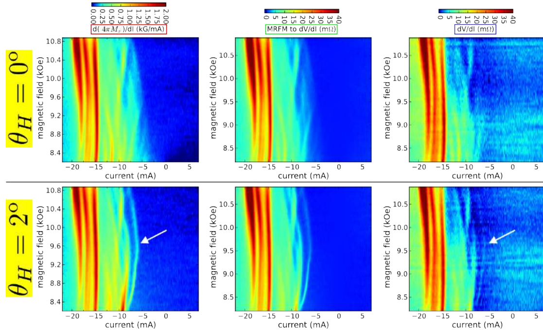
Figure A.1.: Differential phase diagrams obtained at \theta_H = 0^\circ (top row) and at \theta_H = 2^\circ (bottom row). The peak-to-peak current amplitude is I_{pp} = 0.1\text{mA} . The left column shows the raw MRFM data, the middle one, its conversion into differential resistance dV/dI , and the right one, the measured dV/dI using a lock-in amplifier.
