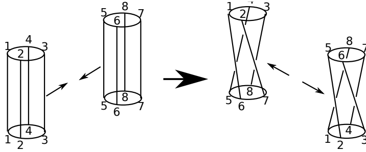
Figure 2.31: 3D reconnection of two flux tubes. Shown are four field lines on each tube. The reconnection does not occur pairwise, i.e., we do not have 1-6 and 6-1 connections on the two new flux tubes, but 1-6 and 1-8 connections, and so on. There is a twist on each new flux tube, that does not vanish when summed over the two tubes (it would be zero for pairwise reconnection, as the new tubes would be twisted in opposite directions). Adapted from Birn and Priest (2007).
