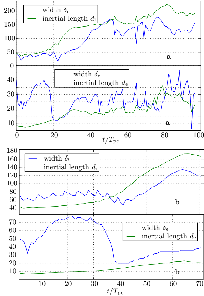
Figure 6.5: Width of the diffusion region \delta_s , and inertial length d_s measured at the center of the diffusion region, for ions and electrons. Panels a are for the simulation with \omega_{ce}/\omega_{pe} = 3 , \sigma_e^{\text{hot}} = 89 , T_{bg} = 1.5 \times 10^7 K and B_G = 0 ; panels b for \omega_{ce}/\omega_{pe} = 6 , \sigma_e^{\text{hot}} = 260 . The phase between 0 and 18T_{pe} for panels a (0 and 33T_{pe} for panels b ) corresponds to times where the tearing instability has not yet started. The decrease in \delta_e between 18 and 20T_{pe} for a ( 33 and 37T_{pe} for b ) is the linear and non-linear growth phase of the instability.
