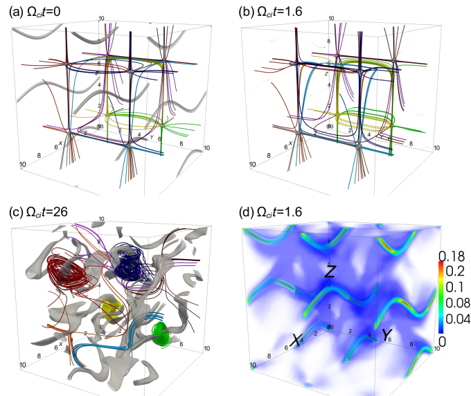
Figure 2.35: From Olshevsky et al. (2013). PIC simulation of a cluster of eight null points. Panels (a), (b) and (c) show magnetic field lines at different times, with gray contours as zones of low B . Panel (d) is the current density.
