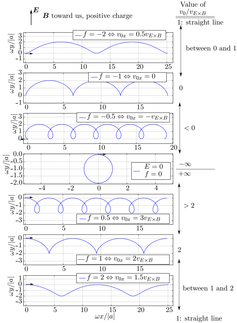
Figure 3.5: Different kind of motions for a non-relativistic particle in constants \mathbf{E} and \mathbf{B} fields. We have \mathbf{B} \propto +\hat{z} , \mathbf{E} \propto +\hat{y} , \mathbf{v}_0 \propto \pm\mathbf{x} , and the motion is drawn in the plane perpendicular to \mathbf{B} .
