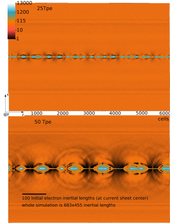
Figure 2.23: Electron number density at two different times, illustrating the tearing instability. The initial state is given by Harris equilibrium. From a PIC simulation detailed in Chapter 6.
