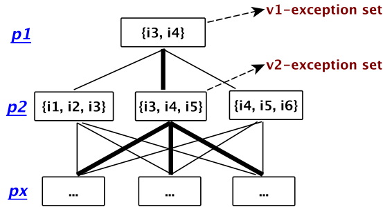
Fig. 4.8 Inclusion Pruning
