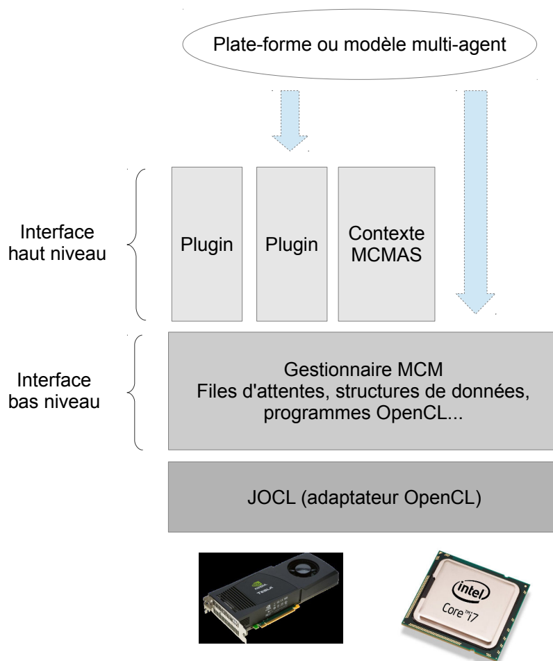
FIGURE 7.1 – Architecture de MCMAS
