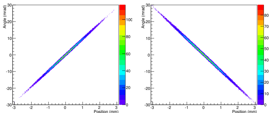
Figure 4.12: Phase space diagram of the particle distribution upon (a) entrance in the object and (b) exit from the object. The histograms were computed with 100000 events, for the following system parameters: d_{T-O} = 100 mm, d_{T-T} = 10 mm, R = 0.1 mm and x/X_0 = 0.5 %.
