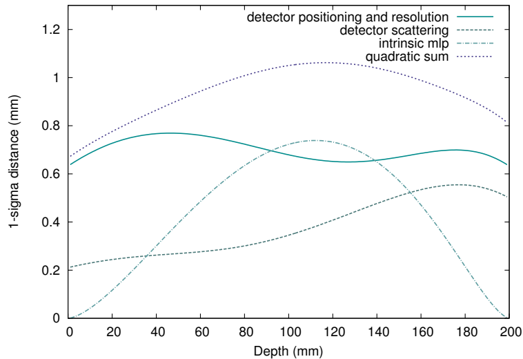
Figure 4.15: 1\text{-}\sigma error envelope as a function of the depth in the object given by the different contributions: resolution and positioning of the trackers, inner tracker material budget, intrinsic MLP uncertainty and quadratic sum of all uncertainties. The system considered has R = 0.1 mm, d_{T-T} = 10 mm and a material budget x/X_0 = 0.5\% .
