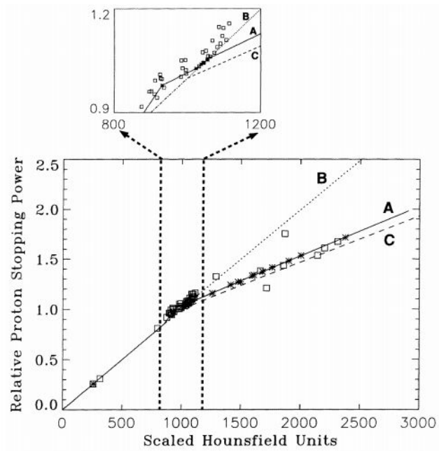
Figure 1.7: Calibration curves for the transformation of Hounsfield values into relative stopping power. The small plot shows in detail the Hounsfield number range corresponding to soft tissue. Figure from [Schneider et al., 1996].
