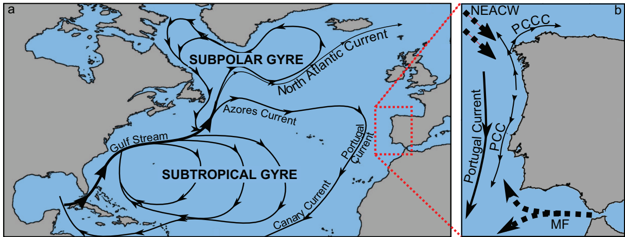
Figure 3.6: a) Schematic representation of the surface currents of the North-Atlantic Ocean [adapted from Tomczak and Godfrey, 1994] . b) Schematic representation of the surface (plain arrows) and subsurface (dashed arrows) currents influencing the Portugal Current system [based on Ambar et al. , 2002; Martins, 2002].
