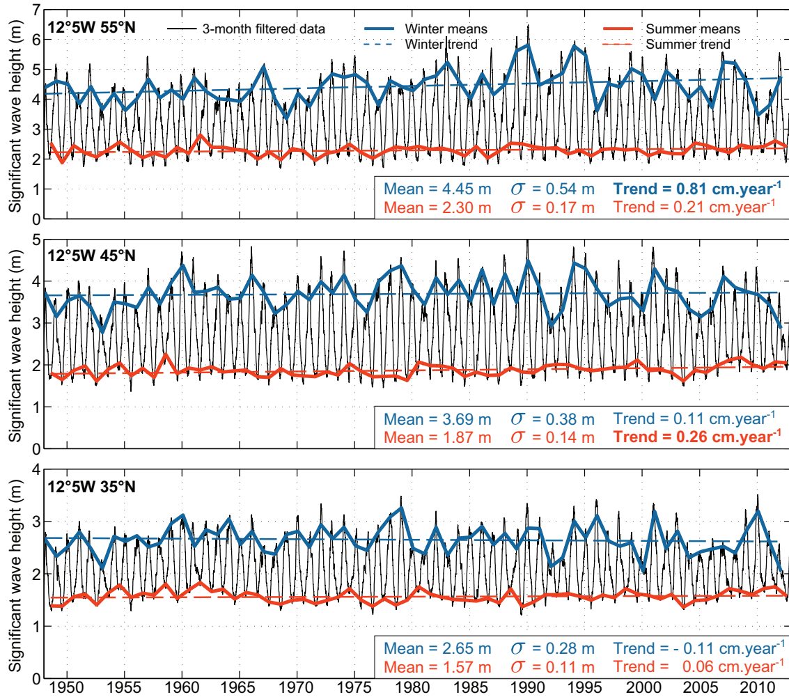
Figure 6.5: Time-series of significant wave heights at P1 (top panel), P2 (middle panel) and P3 (bottom panel) from 1948 to 2013: 3-month filtered data (black line), winter averages (blue solid line) and summer averages (red solid line). The dashed lines correspond to linear regressions fitted through the winter (blue) and summer averages (red). The mean values, the standard deviations ( \sigma ) and the coefficients of the trends are given for each season (bold font type means that the trend is significant with 95% confidence).
