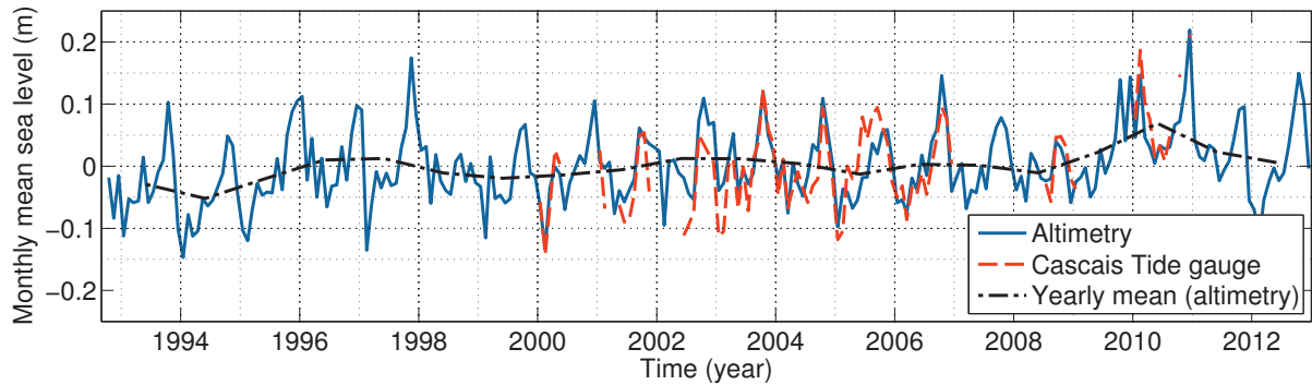
Figure 8.10: Time-series of monthly mean sea level derived from tide gauge measurements at Cascais and satellite observations (AVISO) off the bay of Cascais (CNES/LEGOS).
