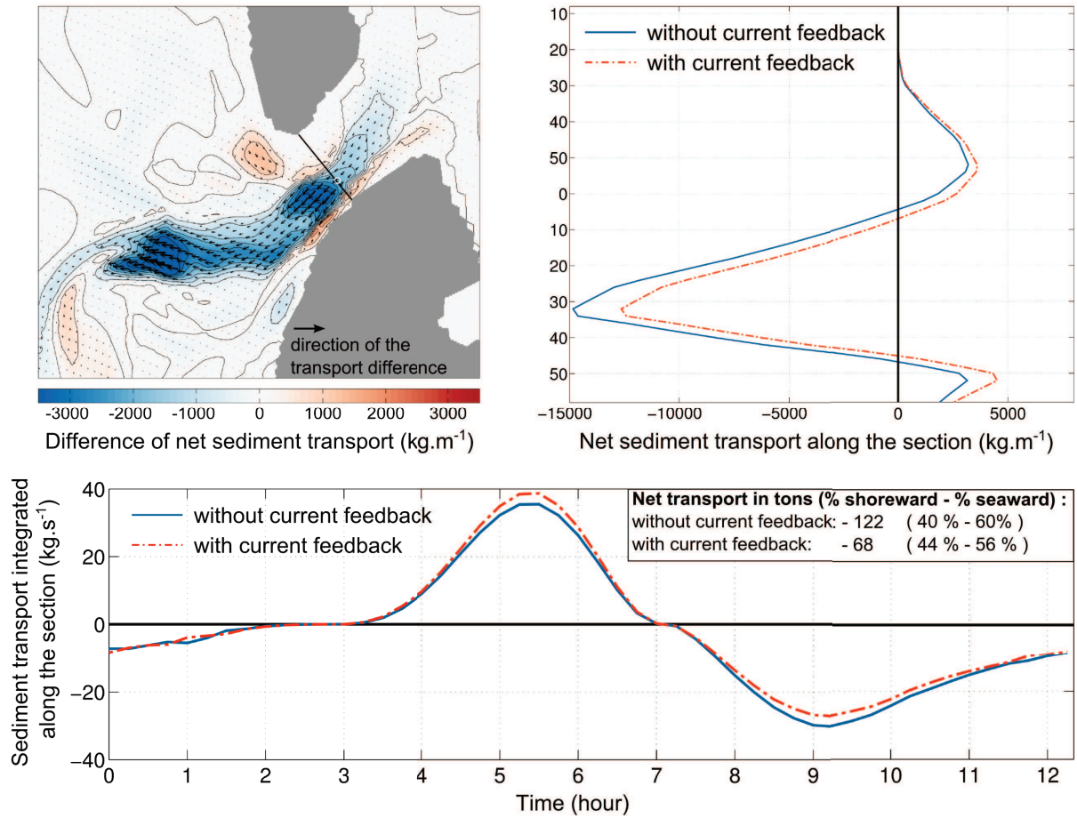
Figure 8.14: Maps of the difference of net sediment transport between the simulation including the current feedback on the waves and the simulation that does not include it (top left); net sediment transport computed across the channel for the two configurations (top right); time-series of sediment transport integrated across the channel for the two configurations (bottom panel).
