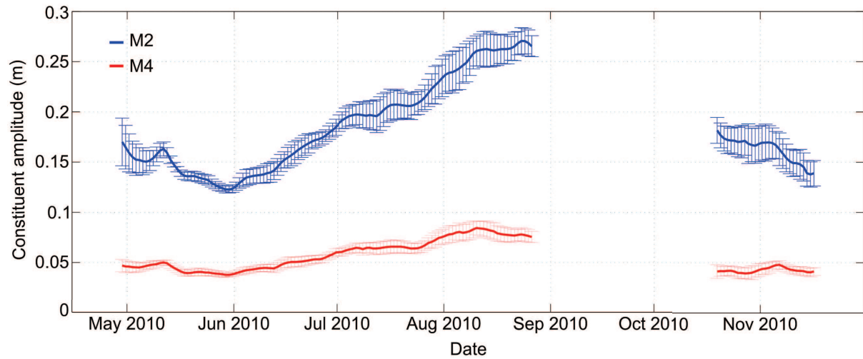
Figure 8.4: Amplitudes and 95% confidence intervals for the tidal constituents M2 (blue) and M4 (red) in the lagoon between April and December 2010 [Dodet et al., 2013].
