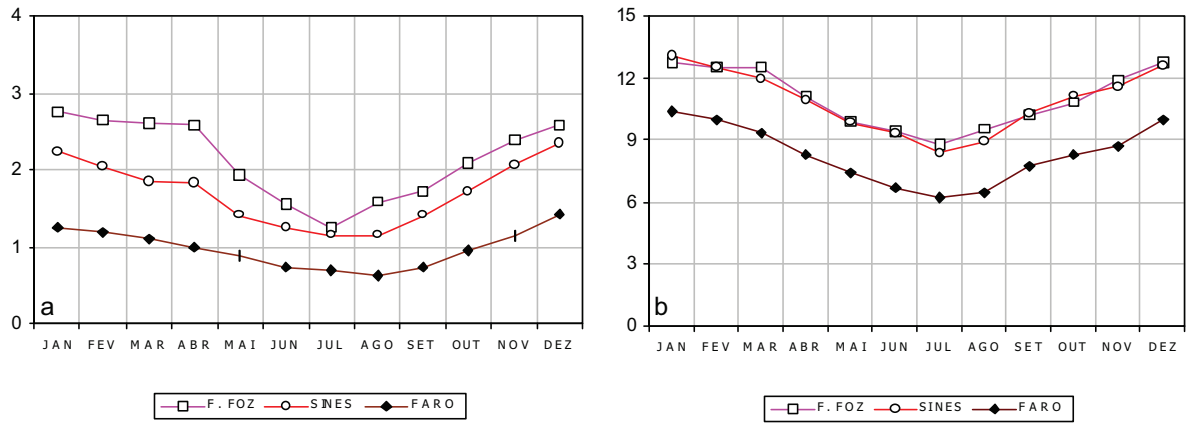
Figure 3.4: Monthly mean evolution along the year of the significant wave height (in m) (a) and the peak period (in s) (b) at Figueira da Foz, Sines and Faro [Costa et al., 2001].
