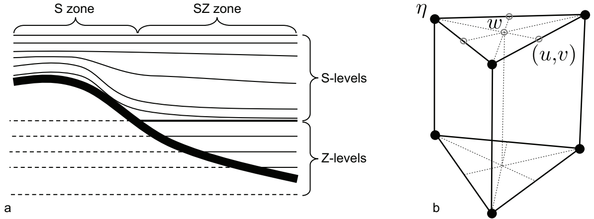
Figure 5.2: Schematic description of the vertical hybrid S - Z coordinates used in SELFIE (a) and location on computational unit of the computed elevations and velocities (b). Adapted from Zhang and Baptista [2008a].
