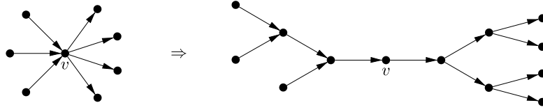
Figure 1.3: Replacement of N^+(v) and N^-(v) by switching out and in-arborescence with root v and leaves N^+(v) and N^-(v) .
