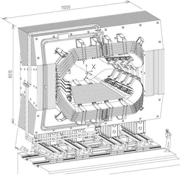
Figure 2.8: Scheme of the LHCb dipole magnet. The interaction point lies behind the magnet.
