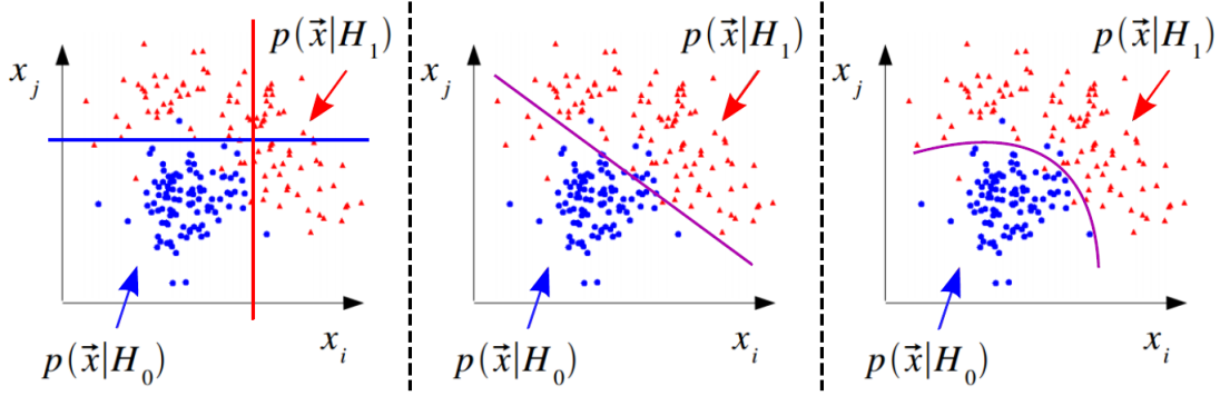
Figure 6.1: Illustration of rectangular cuts (on the left) and multivariate algorithms (on the middle and right), for two variables x_i and x_j . Red and blue points correspond to signal and background samples [93].
