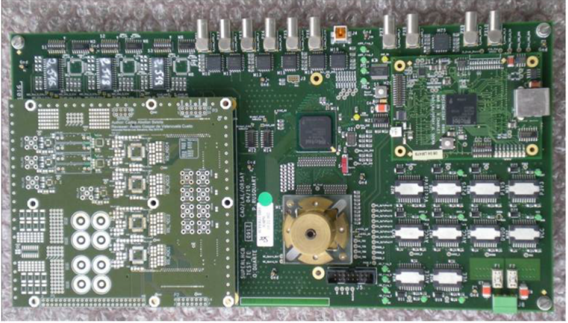
Figure 7.1: Picture of the prototype of the Front-End board. The analogue mezzanine is visible on the left. The two FPGAs are in the central part of the board, one is black and other is under the copper socket.
