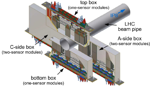
Figure 2.6: The IT station layout.
