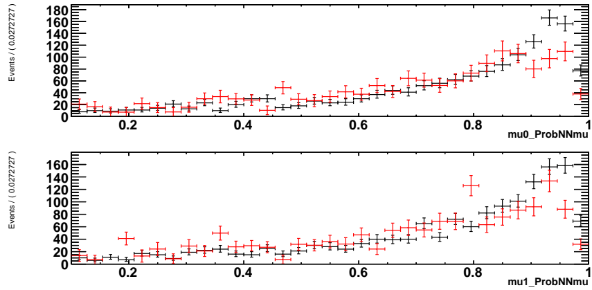
Figure C.1: ProbNNmu distributions in MC (black) and sPlotted data (red) in 20% sample, selected with nominal L0 trigger cuts (L0HadronTIS).
