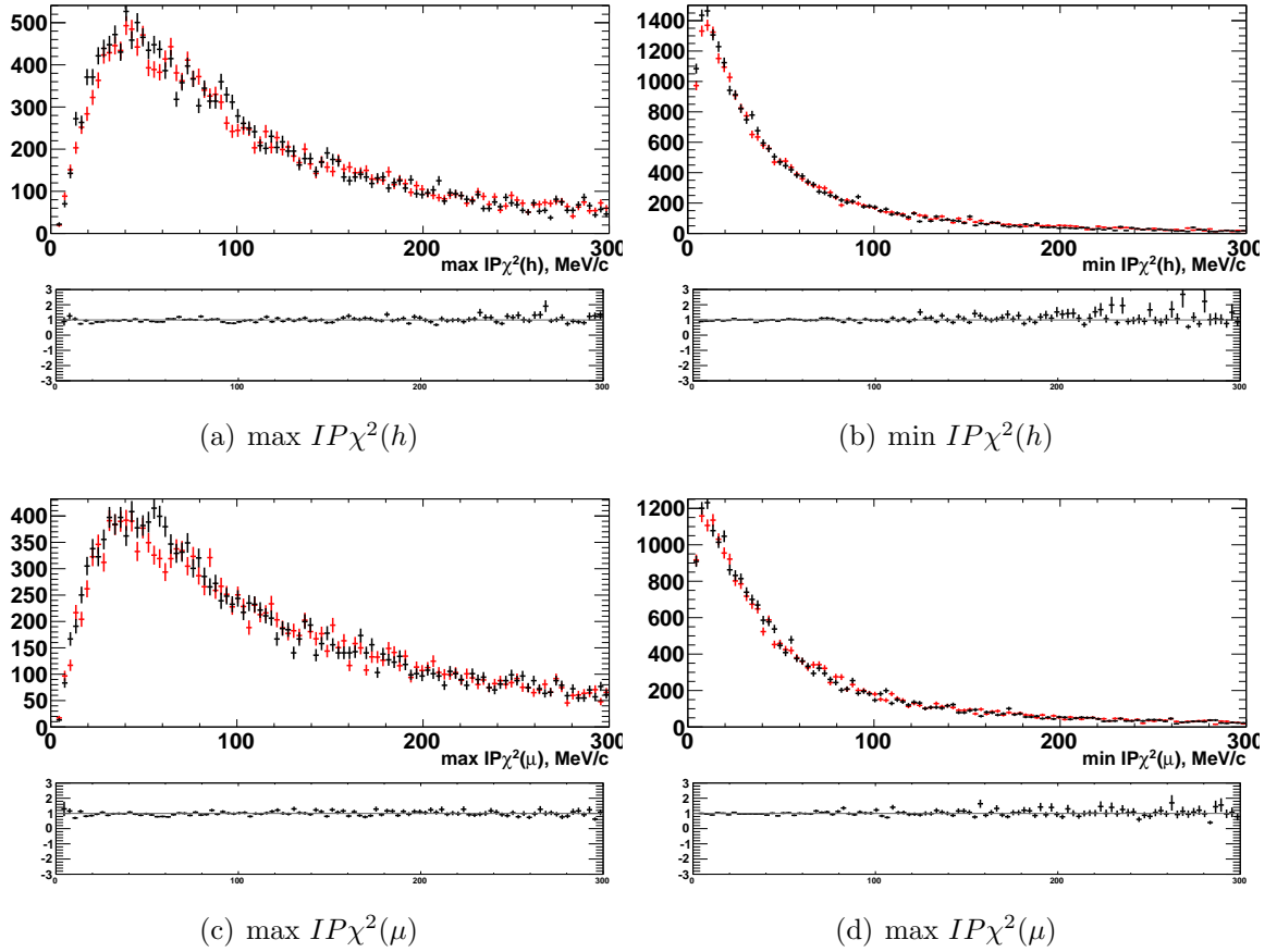
Figure 5.14: Impact parameter \chi^2 distributions of daughters tracks in data (red) and MC (black) in D^0 \rightarrow K^- \pi^+ \pi^+ \pi^- with nominal selection (LOHadronTIS). The pull distributions show the ratio between these two sets of points.
