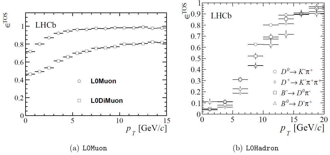
Figure 2.26: The efficiency \epsilon^{TOS} [78] of L0Muon for B^+ \rightarrow J/\psi(\rightarrow \mu^+\mu^-)K^+ and L0Hadron for B^0 \rightarrow D^-\pi^+ , B^- \rightarrow D^0\pi^- , D^0 \rightarrow K^-\pi^+ and D^+ \rightarrow K^-\pi^+\pi^+ are shown as a function of p_T .
