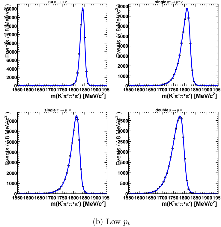
Figure 5.41: RooKeysPDFs describing the invariant mass of the D^0 \rightarrow K^- \pi^+ \pi^+ \pi^- peaking background. Both the “high p_t ” (top) and “low p_t ” (bottom) components receive four contributions: no decay in flight (top left), \pi^+ decay in flight (top right), \pi^- decay in flight (bottom left), both misidentified pions decayed in flight (bottom right). These shapes are obtained by recalculating the mass of candidates after the kinematics of one or two pions has been modified to reproduce the effect of a decay in flight (see the detailed description in the text).
