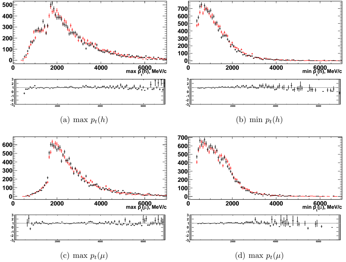
Figure 5.16: Momentum distributions of daughter tracks in data (red) and MC (black) in D^0 \rightarrow K^- \pi^+ \rho/\omega (\rightarrow \mu^+ \mu^-) with nominal selection ( L0HadronTOS || L0MuonTOS ). The pull distributions show the ratio between these two sets of points.
