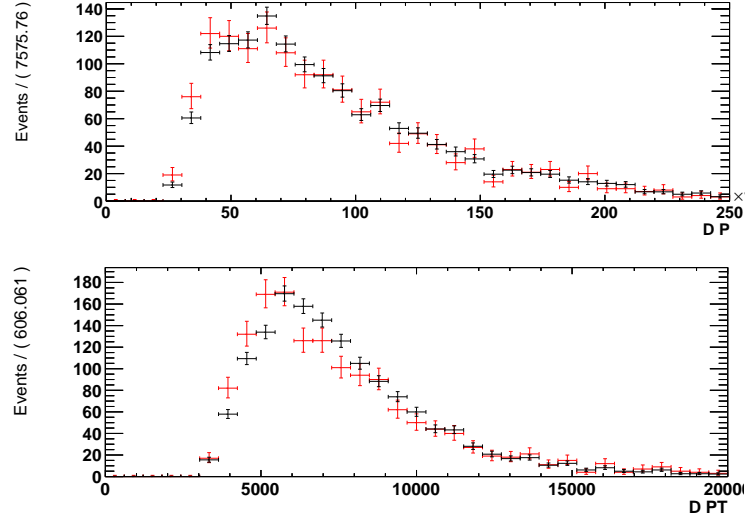
(a) MC
