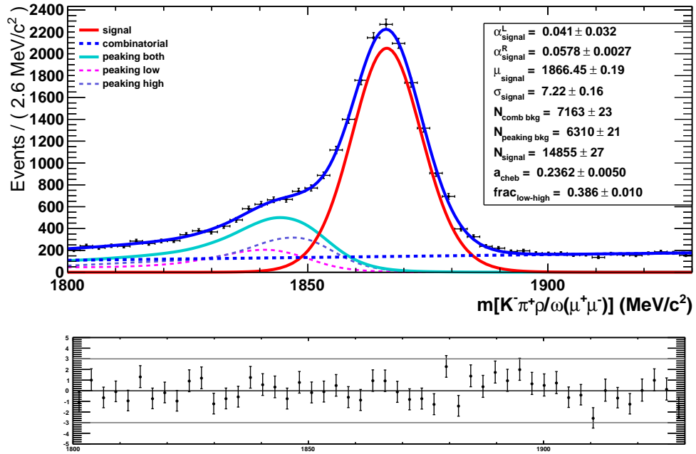
Figure 5.36: Fit to the D^0 \rightarrow K^- \pi^+ \rho/\omega (\rightarrow \mu^+ \mu^-) data sample, selected with LOHadronTOS|LOMuonTOS requirement, using the Cruijff function to parametrize the signal peak. The other contributions to the total PDF are described in detail in sections 5.7.3 and 5.7.4.
