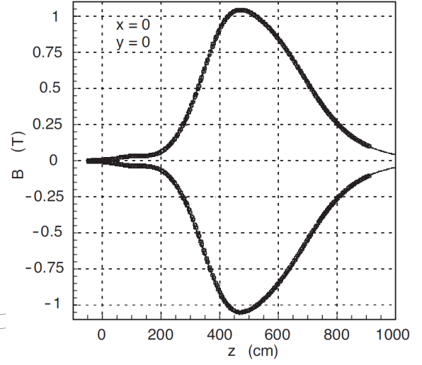
Figure 2.9: Magnetic field along the z axis.
