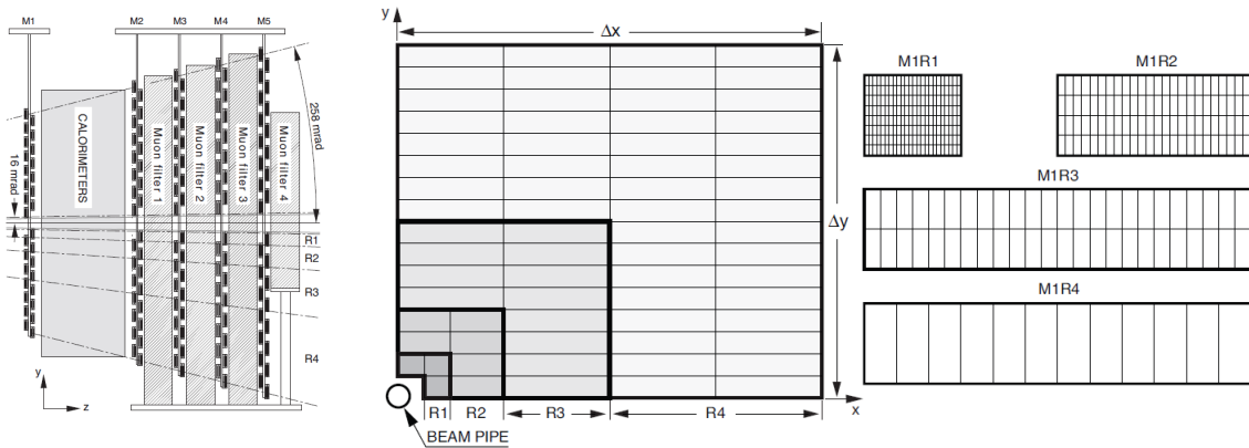
Figure 2.18: Overview of the LHCb muon stations (left) and their segmentation (right).
