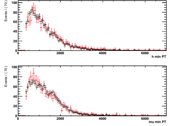
(a) MC
