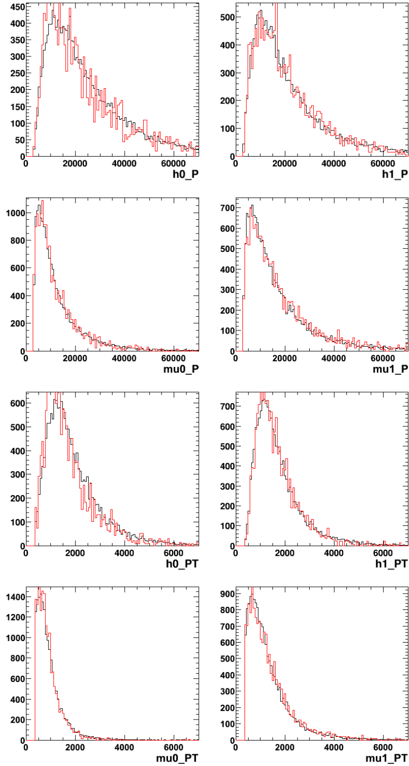
Figure 5.20: Momentum distributions of daughters tracks in MC for signal (red) and normalization (black).
