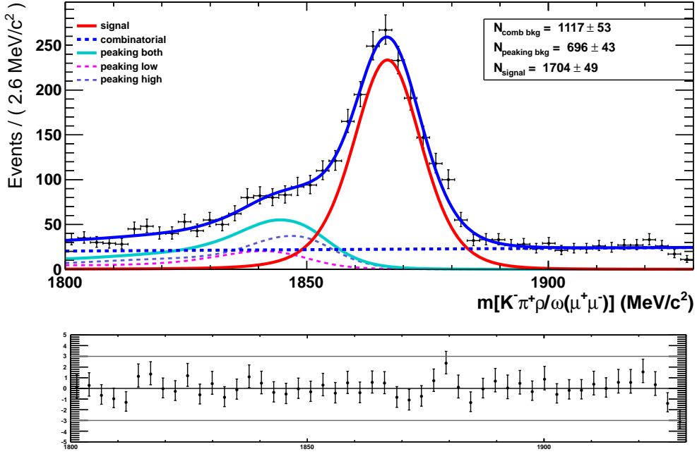
Figure 5.50: Invariant mass distribution in unblinded D^0 \rightarrow K^- \pi^+ \rho/\omega (\rightarrow \mu^+ \mu^-) data sample, selected with LOMuonTIS. Red solid line - signal, blue dashed - combinatorial, cyan solid - peaking background, violet and magenta dashed - components of “highPT” and “lowPT” peaking forms. The fit parameters can be found in Table 5.14.
