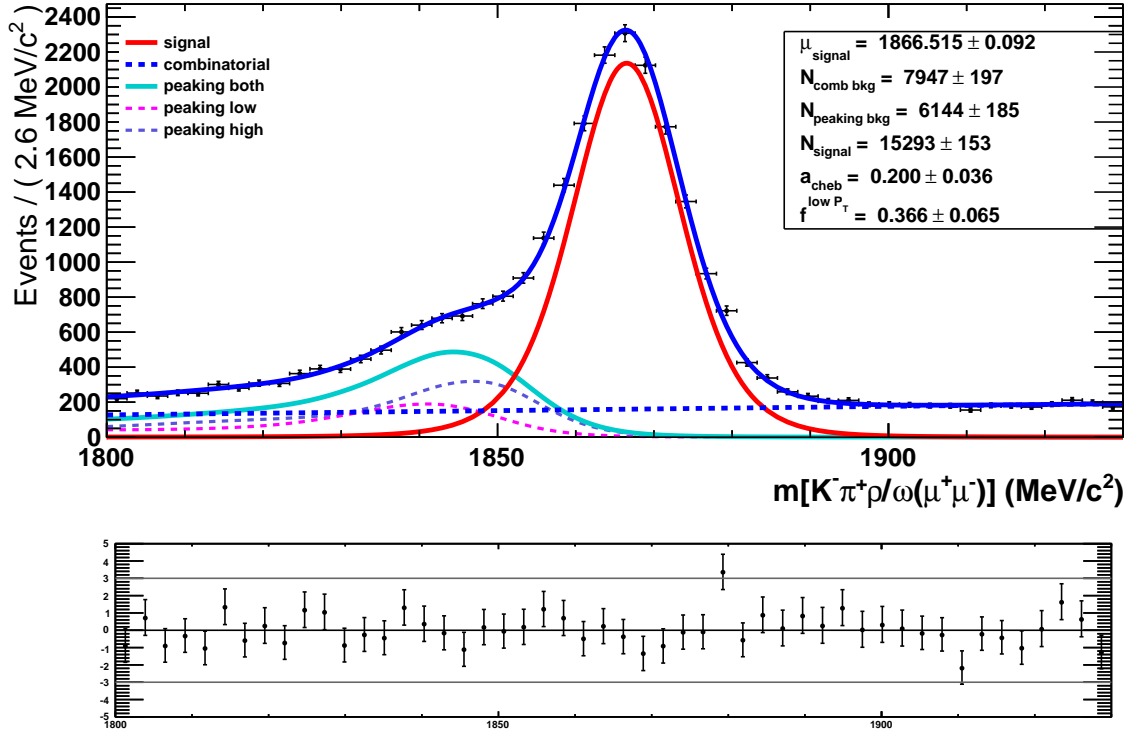
Figure 5.47: Fit to the D^0 \rightarrow K^- \pi^+ \rho/\omega (\rightarrow \mu^+ \mu^-) data sample, selected with L0HadronTOS||L0MuonTOS requirement. The fit model built from Section 5.7.1 to Section 5.7.4 is employed. This is a way to validate it. The components of the total PDF (blue solid line) are: the signal (red solid line), the combinatorial background (blue dashed line) and the “high p_t ” (violet dashed line) and “low p_t ” (magenta dashed line) components of the peaking background. The coefficient of the first order Chebyshev polynomial describing the combinatorial background is free to float.
