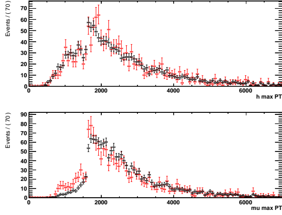
(a) MC
