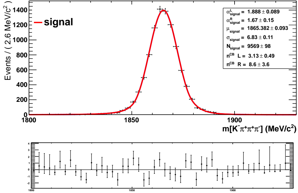
Figure B.2: Fit to the D^0 \rightarrow K^- \pi^+ \pi^+ \pi^- MC sample with the Double Crystal Ball function.
