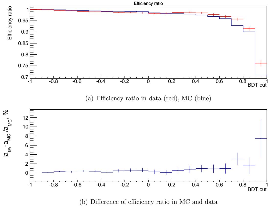
Figure 5.26: Efficiency ratio in data and MC (top) and relative difference between these two ratios (bottom). This based on the samples selected with the L0\text{HadronTOS} | L0\text{MuonTOS} criteria. The cut used in the analysis is BDT > 0.2 .
