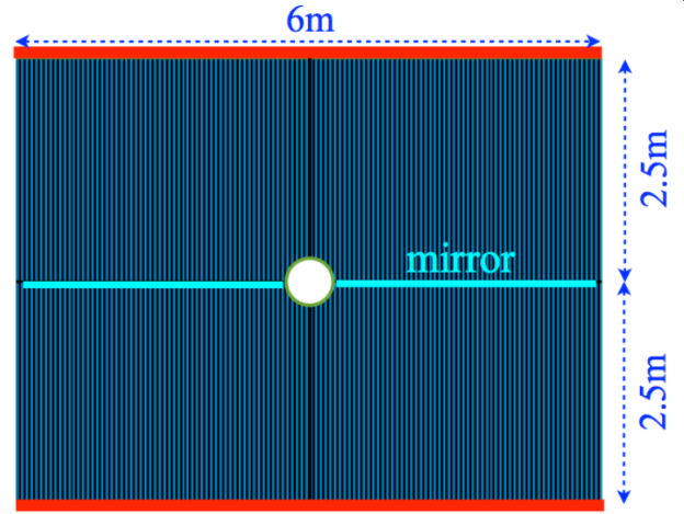
Figure 2.23: Layout of scintillating fibre detector (SciFi). The SiPMs are in red.
