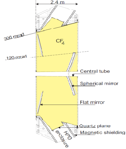
Figure 2.13: Side view schematic layout of the RICH2 detector.
