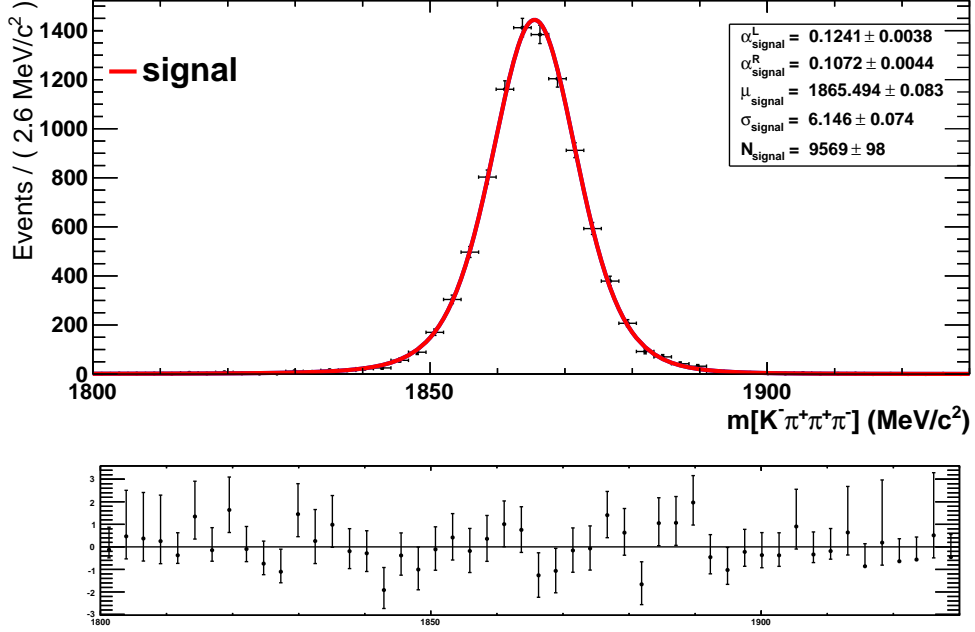
Figure 5.32: Fit to the D^0 \rightarrow K^- \pi^+ \pi^+ \pi^- MC sample with the Cruijff function.
