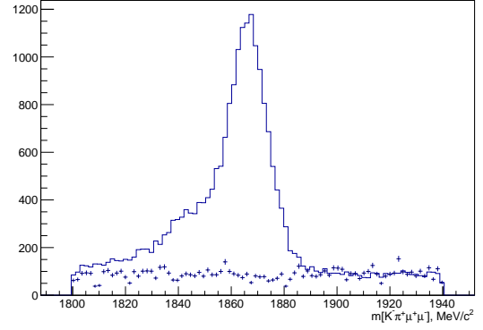
Figure 5.38: Invariant mass distribution and generated combinatorial background (crosses) for the D^0 \rightarrow K^- \pi^+ \rho/\omega(\rightarrow \mu^+ \mu^-) selected with LOHadronTOS || LOMuonTOS requirement.
