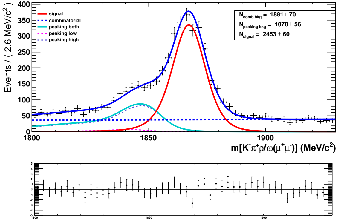
Figure 5.48: Invariant mass distribution in unblind D^0 \rightarrow K^- \pi^+ \rho/\omega (\rightarrow \mu^+ \mu^-) data sample, selected with L0HadronTIS. Red solid line - signal, blue dashed - combinatorial, cyan solid - peaking background, violet and magenta dashed - components of “highPT” and “lowPT” peaking forms. Fit parameters can be found in Table 5.14.
