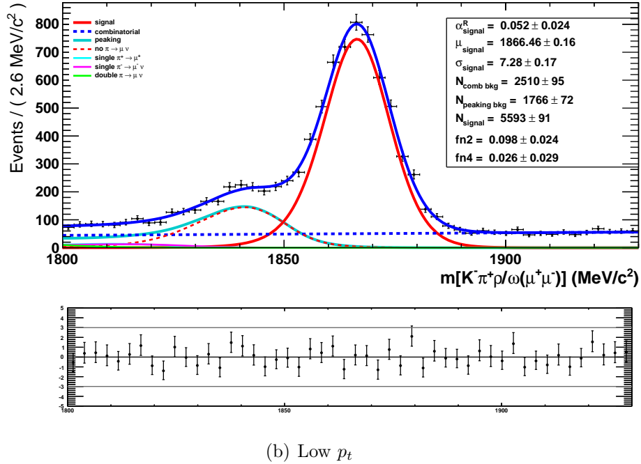
Figure 5.44: Fit to the D^0 \rightarrow K^- \pi^+ \rho/\omega (\rightarrow \mu^+ \mu^-) sample selected with LOHadronTOS|LOMuonTOS requirement. It is performed in order to validate the description of the D^0 \rightarrow K^- \pi^+ \pi^+ \pi^- peaking background based on the RooKeysPDFs which determination is described in the text, as well as in order to determine the relative fractions of the four contributions this background is made of. The components of the total PDF are: the signal (red solid), the combinatorial background (blue dashed) and the various components of the peaking background. These components are with: no pion decayed in flight (red dashed), one \pi^+ decayed in flight (solid cyan), one \pi^- decayed in flight (magenta solid), both pions decayed in flight (solid green). The coefficient of the first order Chebyshev polynomial describing the combinatorial background is fixed to the value found by a fit to the generated combinatorial background (see Section 5.7.3).
