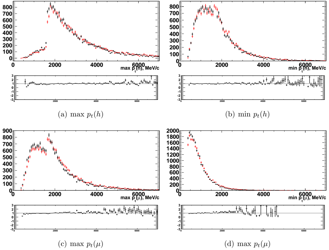
Figure E.1: Momentum distributions of daughters tracks in data (red) and MC (black) in D^0 \rightarrow K^- \pi^+ \pi^+ \pi^- with nominal selection ( L0HadronTOS | L0MuonTOS ).
