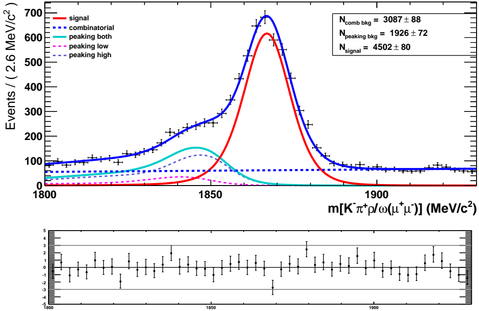
Figure 5.51: Invariant mass distribution in the unblinded D^0 \rightarrow K^- \pi^+ \rho/\omega (\rightarrow \mu^+ \mu^-) data sample, selected with LOHadronTIS||LOMuonTIS. Red solid line - signal, blue dashed - combinatorial, cyan solid - peaking background, violet and magenta dashed - components of “highPT” and “lowPT” peaking forms. The fit parameters can be found in Table 5.14.
