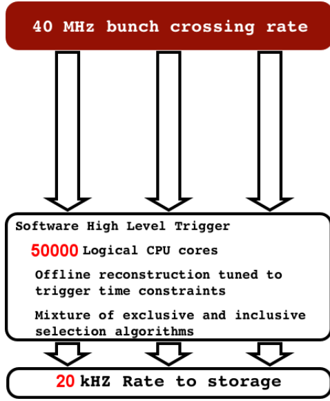
Figure 2.22: Scheme of the LHCb trigger system after upgrade.
