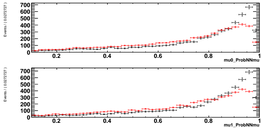
Figure C.2: ProbNNmu distributions in MC (black) and sPlotted data (red) in the sample, selected with L0HadronTOS | L0MuonTOS L0 trigger cuts.
