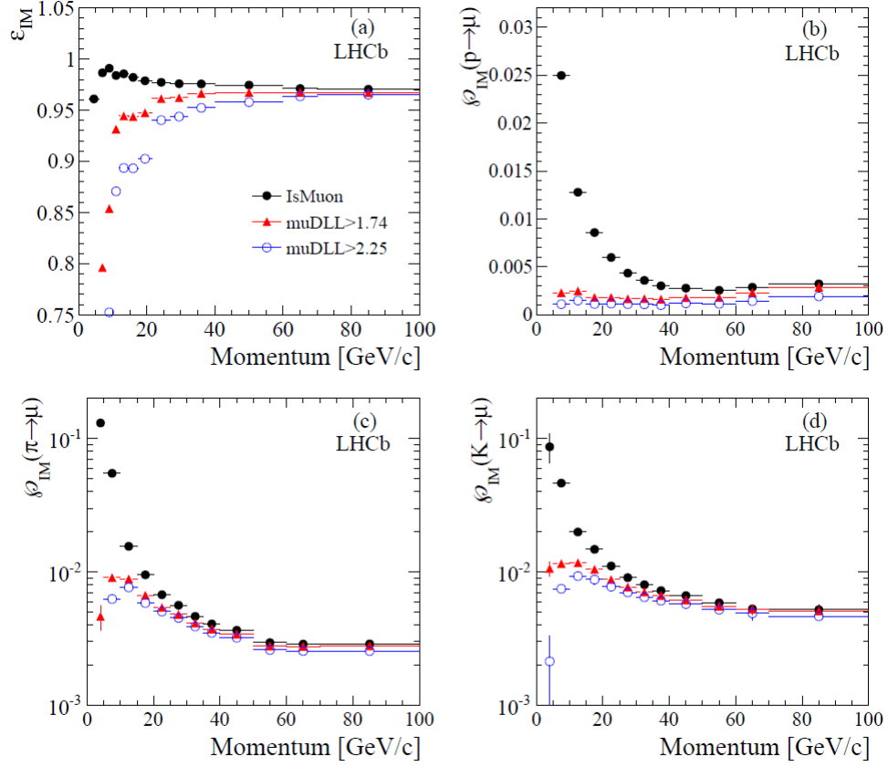
Figure 2.27: Muon efficiency [79] (a) and misidentification probabilities for protons (b), pions (c) and kaons (d) as a function of the particle momentum for the IsMu requirement alone (black solid circles) and with the additional cuts \text{PID}_{\text{mu}} > 1.74 (red triangles) and \text{PID}_{\text{mu}} > 2.25 (blue open circles).
