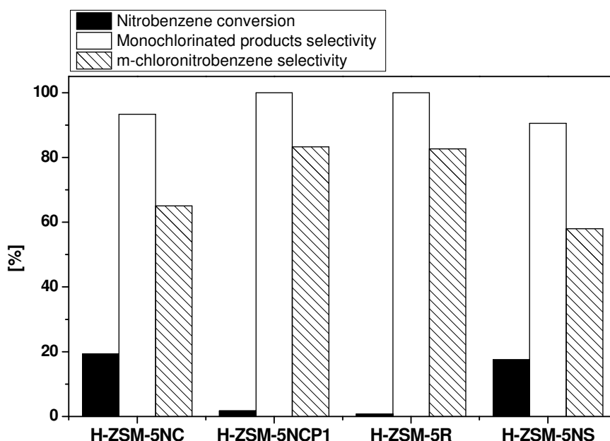
Figure 5.24 Nitrobenzene chlorination reaction over the four MFI-type zeolite samples. Conditions: T = 150 °C; TCCA: PhNO 2 = 1: 1; 214 mg of catalyst; Flow = 100 mL/min; TOS = 5 h
