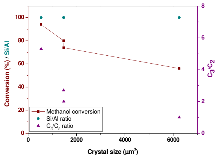
Figure 4.9 Influence of crystal size on the catalytic performance in MTO reaction Conditions: T=698 \text{ K} , 60 \text{ mg H-ZSM-5F} activated 1 \text{ h} at 823 \text{ K} , \text{WHSV} = 1.12 \text{ g}_{\text{MeOH}}/\text{g}_{\text{cat}} \cdot \text{h}^{-1} , \text{TOS} = 2 \text{ h}
